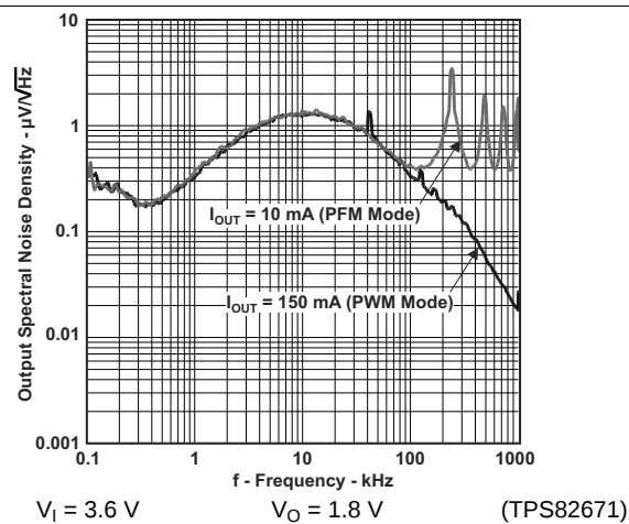
Figure 6. Output Spectral Noise Density vs. Frequency
