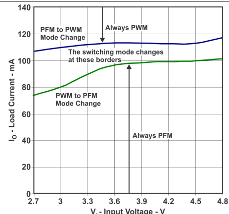
Figure 40. PFM/PWM Boundaries
