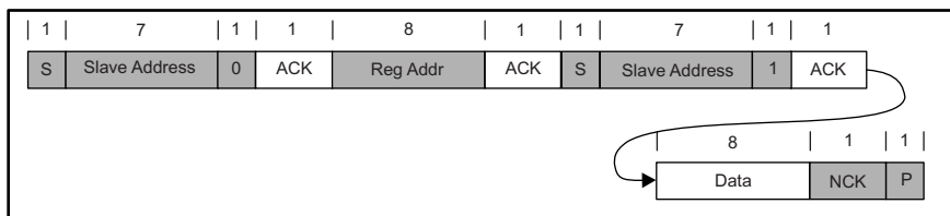
Figure 22. Single Read
