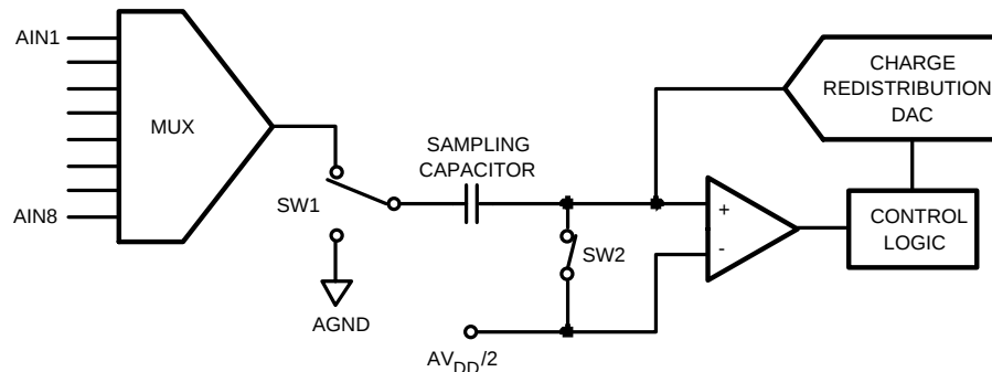
Figure 21. ADC78H90 in Track Mode
