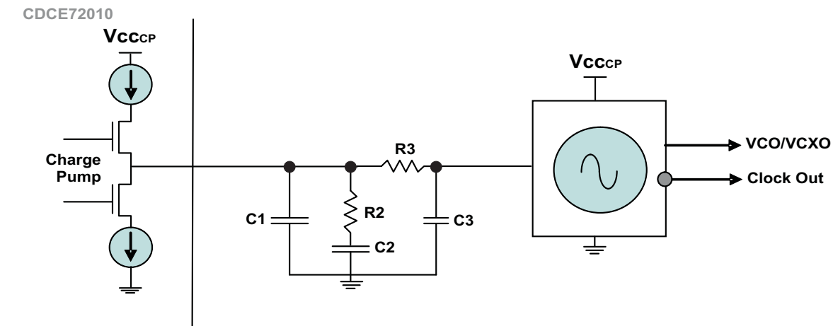
Figure 34. Loop Filter
