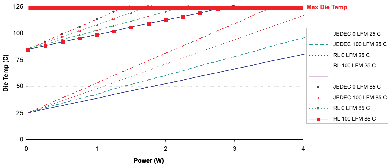
Figure 33. Die Temperature
