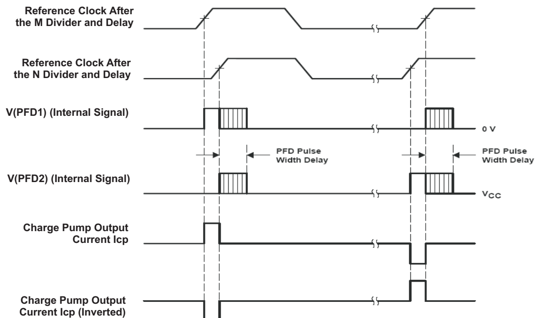
Figure 25. Charge Pump
