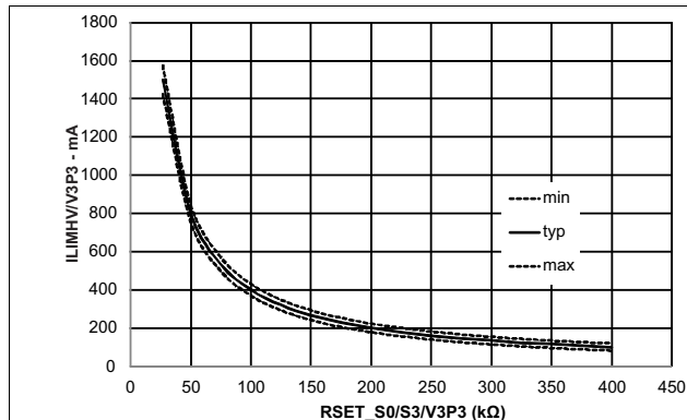
Figure 3. I_{LIM} vs R_{SET} for VHV and V3P3
