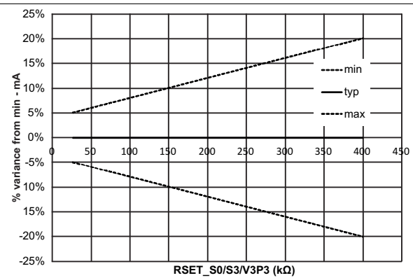
Figure 4. % Variance from Minimum I_{LIM} vs R_{SET}
