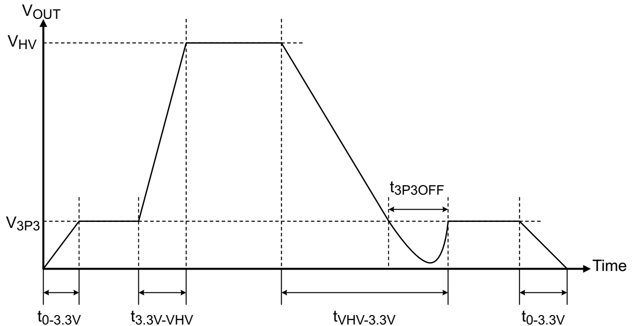
Figure 5. Output Voltage Transitions (Timing Transitions are 10% to > 90%)
