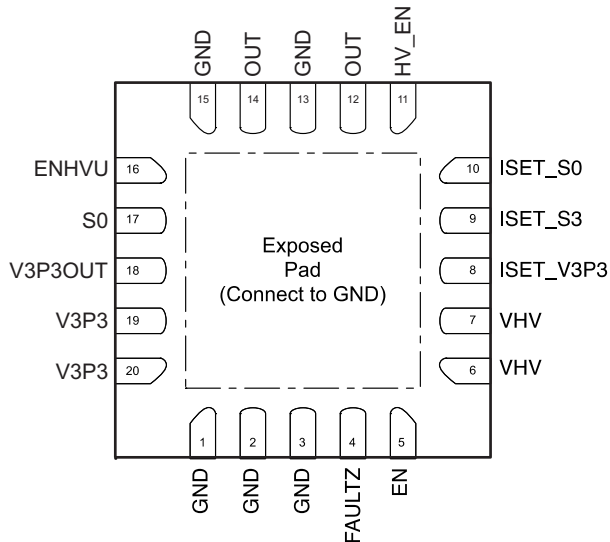
RGP Package VQFN With Exposed Thermal Pad Top View
