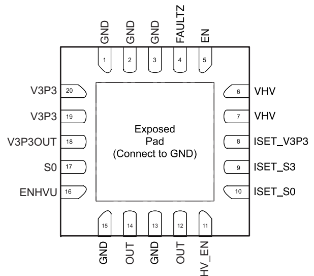
RGP Package VQFN With Exposed Thermal Pad Bottom View
