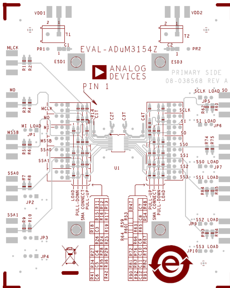
Figure 5. Top Side Layout
