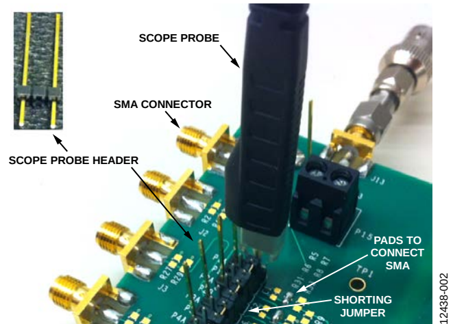
Figure 2. Optional Components
