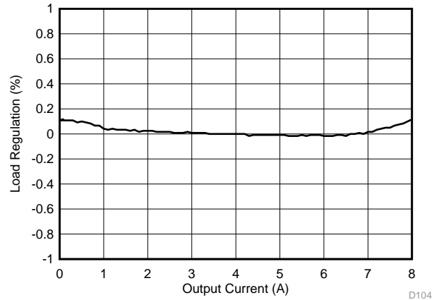
Figure 27. Load Regulation, V_{IN} = 12\text{ V}
