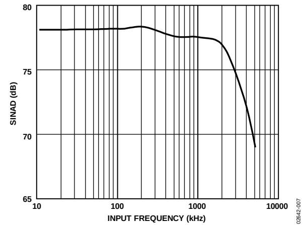
Figure 7. SINAD vs. Input Tone (AD8021 Input Circuit)
