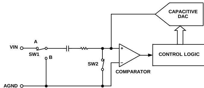
Figure 13. ADC Acquisition Phase
