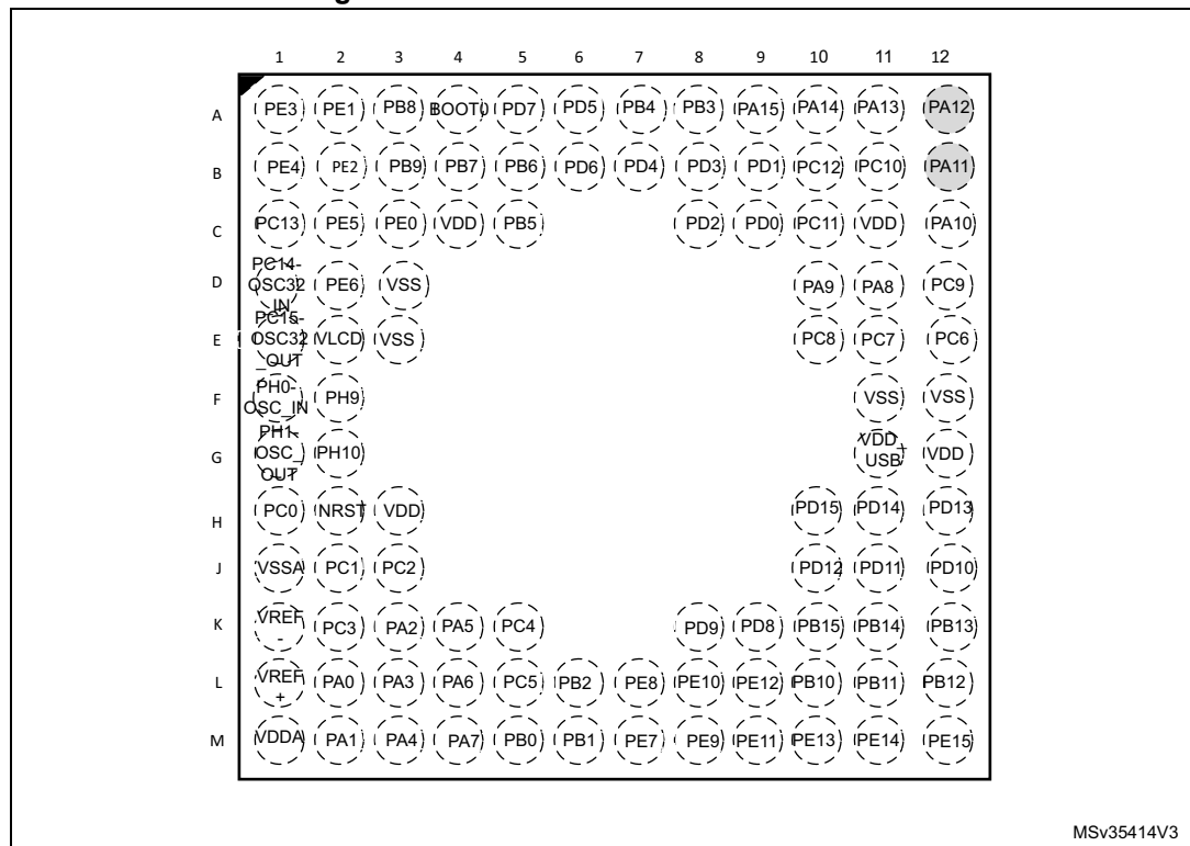
Figure 4. STM32L073xx UFBGA100 ballout
