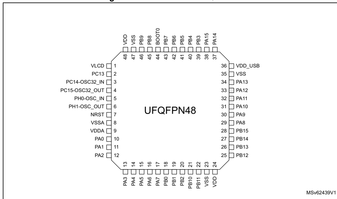
Figure 8. STM32L073xx UFQFPN48
