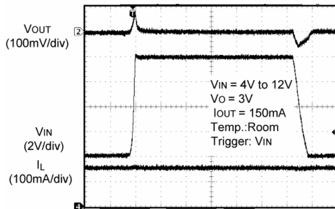
Line Transient
