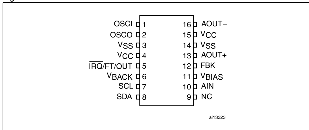
Figure 2. Pin connection
