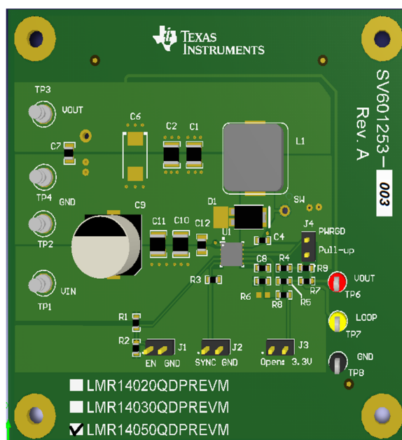
Figure 1. LMR14050QDPREVM Board
