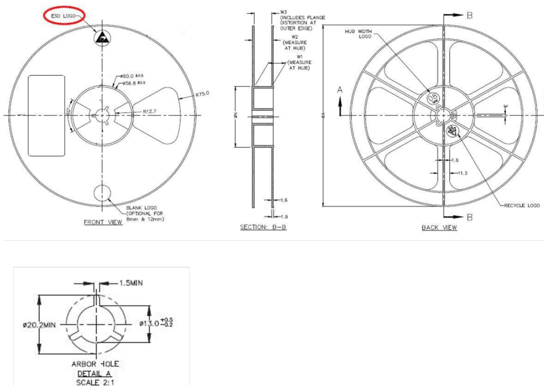
Figure 32. DFN4 1x1 reel outline
