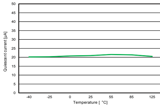
Figure 9. Quiescent current vs. temperature ( I_{OUT} = 0 mA)
