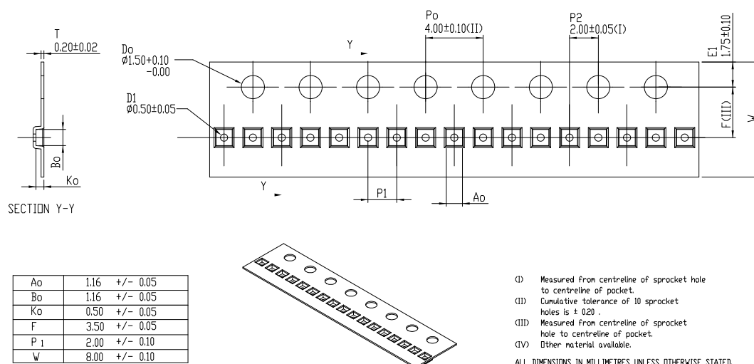
Figure 31. DFN4 1x1 tape outline
