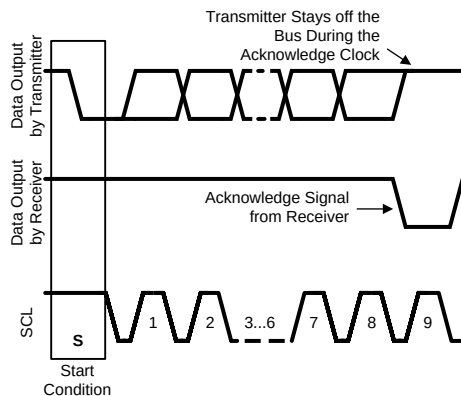
Figure 20. Acknowledge Signal
