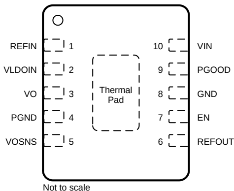
Pin Functions
