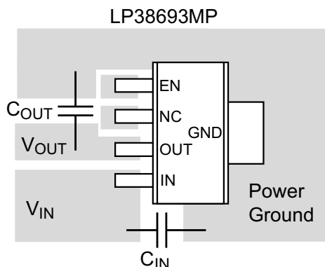
Figure 32. SOT-223 Layout
