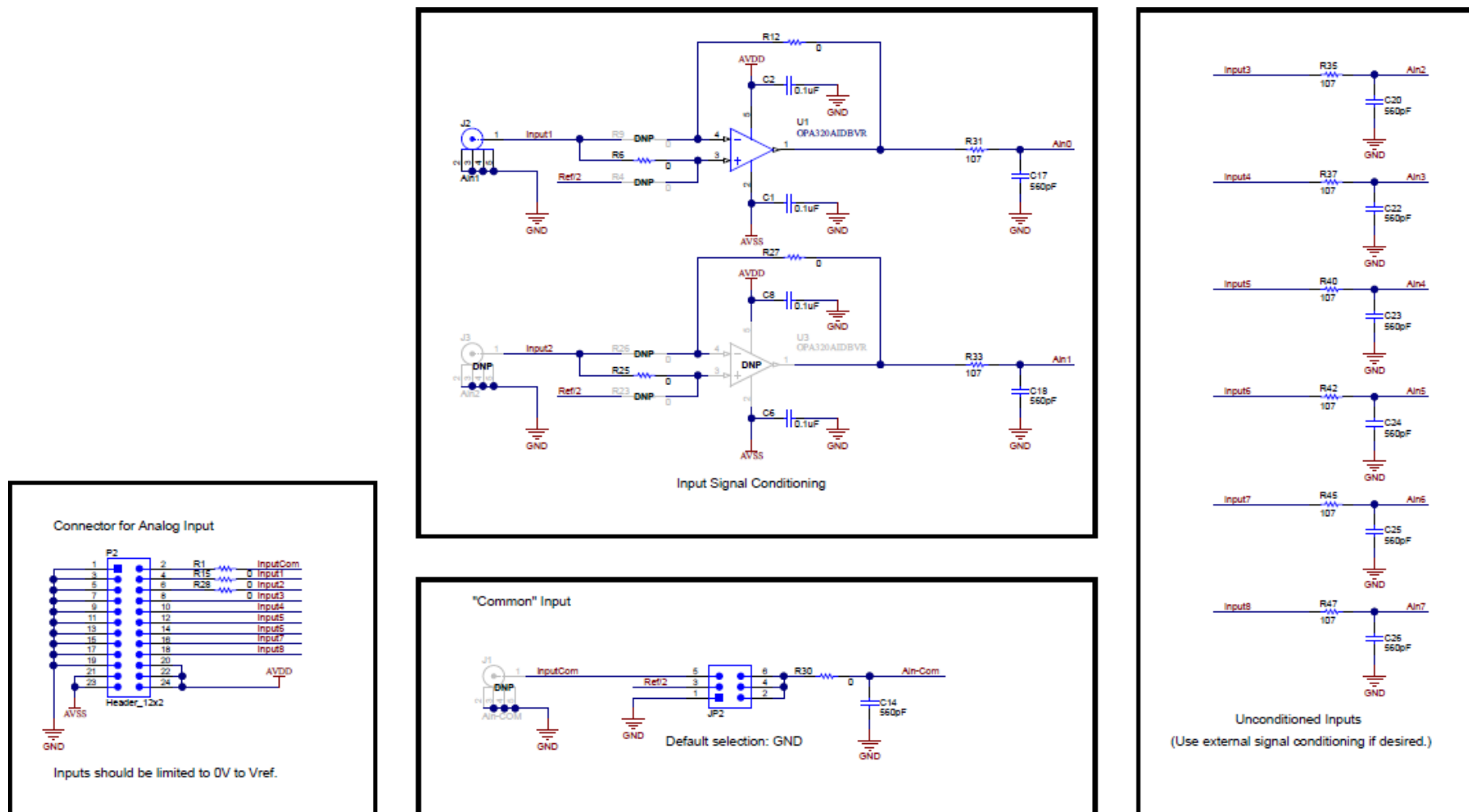
Figure 23. ADS8588EVM-PDK Schematic
