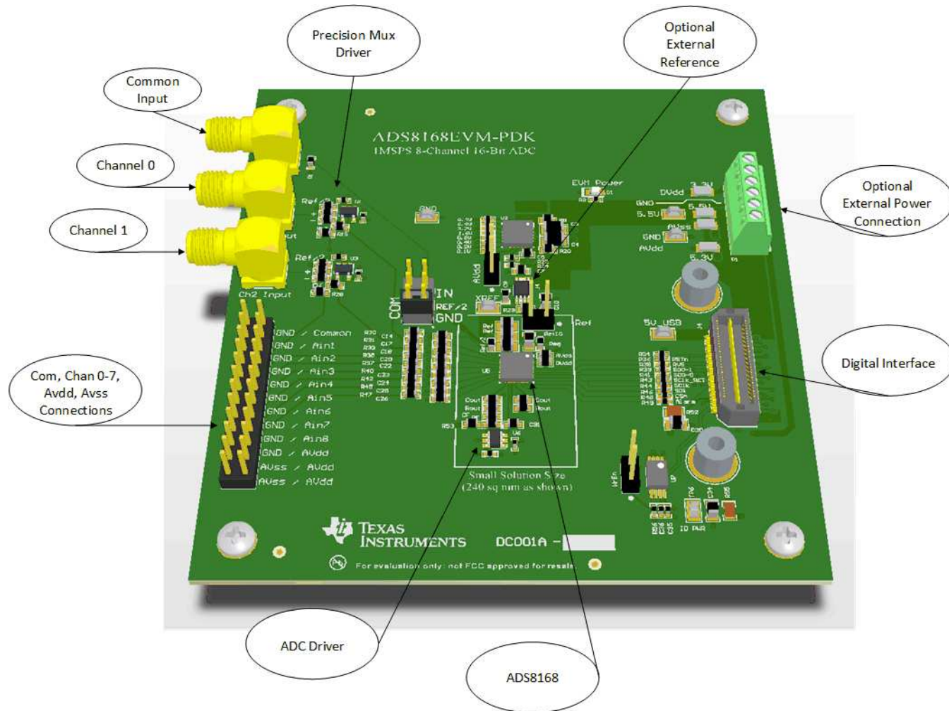
Figure 2. ADS8168EVM Features
