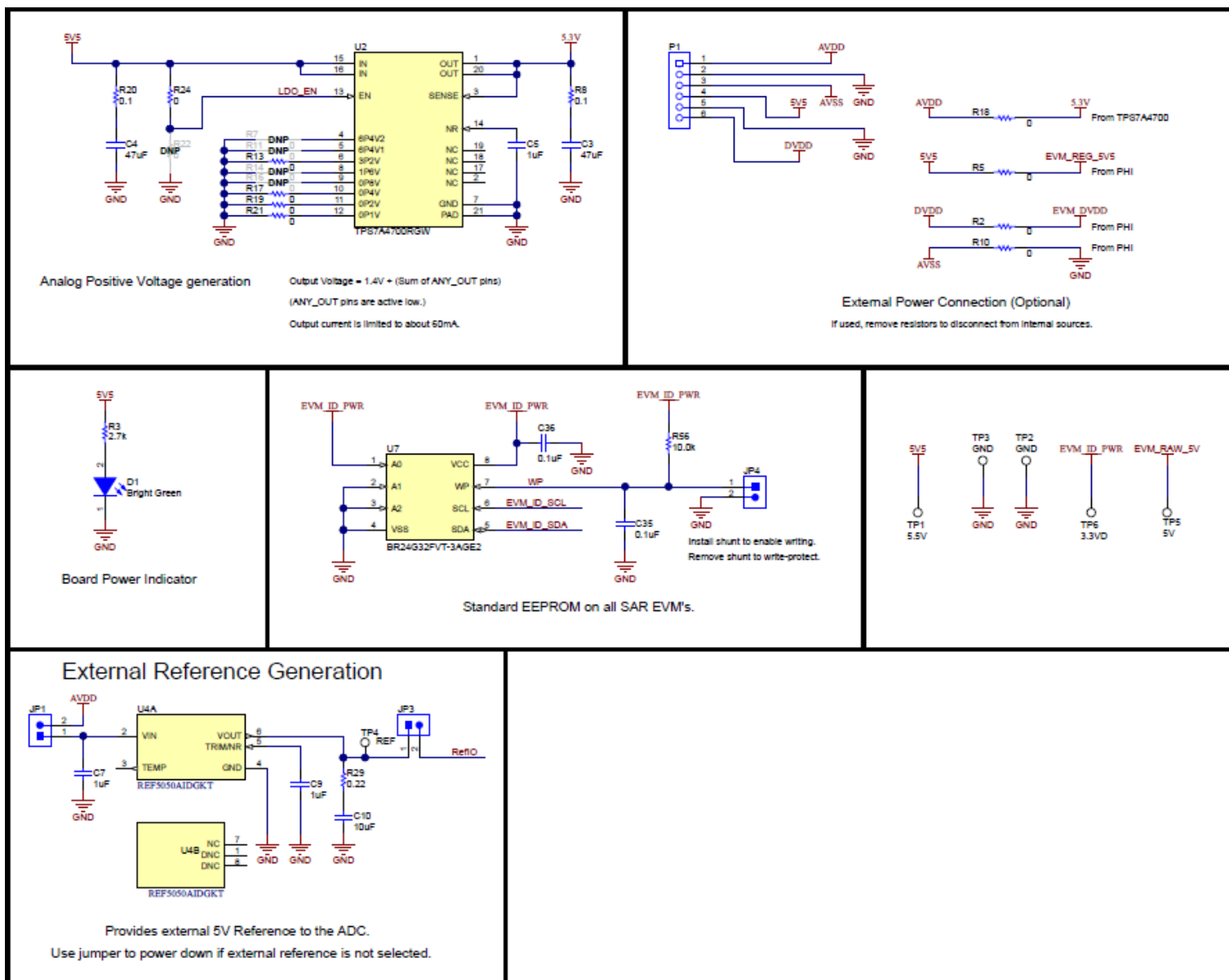
Figure 24. ADS8588EVM-PDK Schematic
