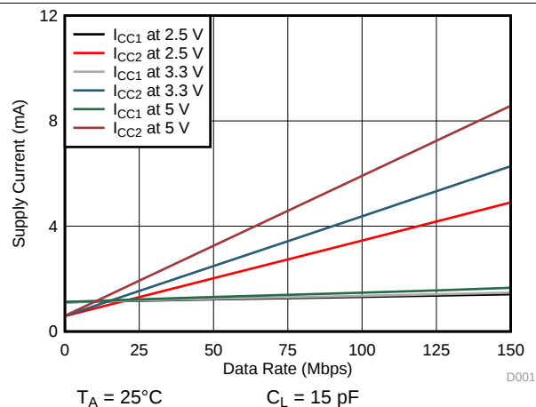
Figure 7. Supply Current vs Data Rate (With 15-pF Load)
