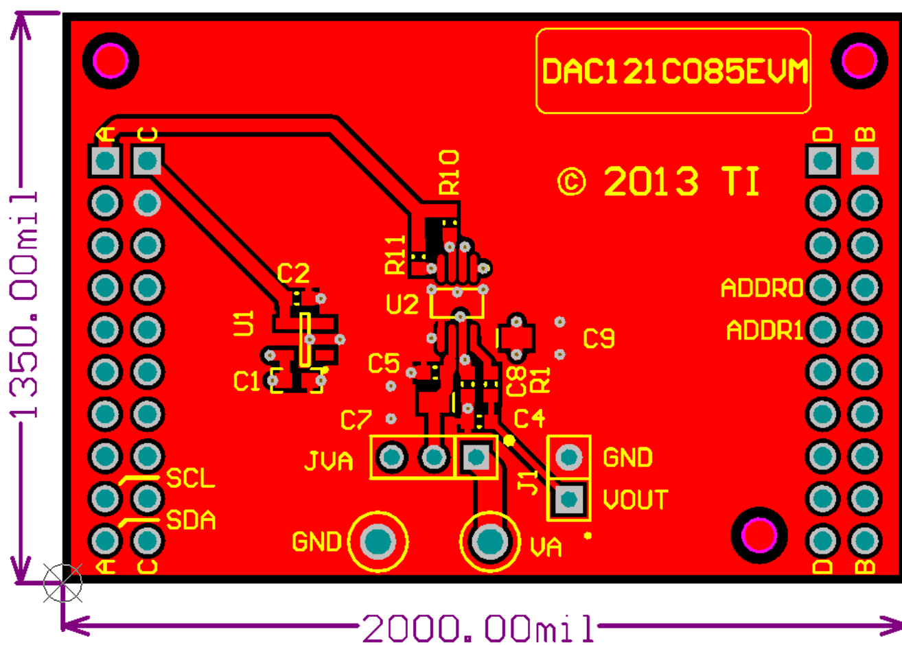
Figure 4-1. Top Assembly Layer
