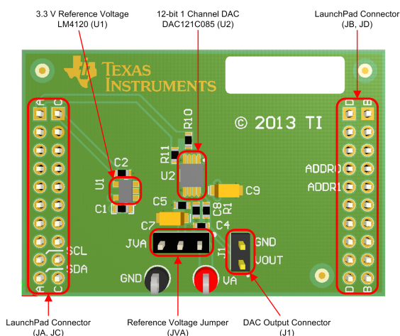
Figure 3-1. DAC121C085EVM Attached to MSP430
