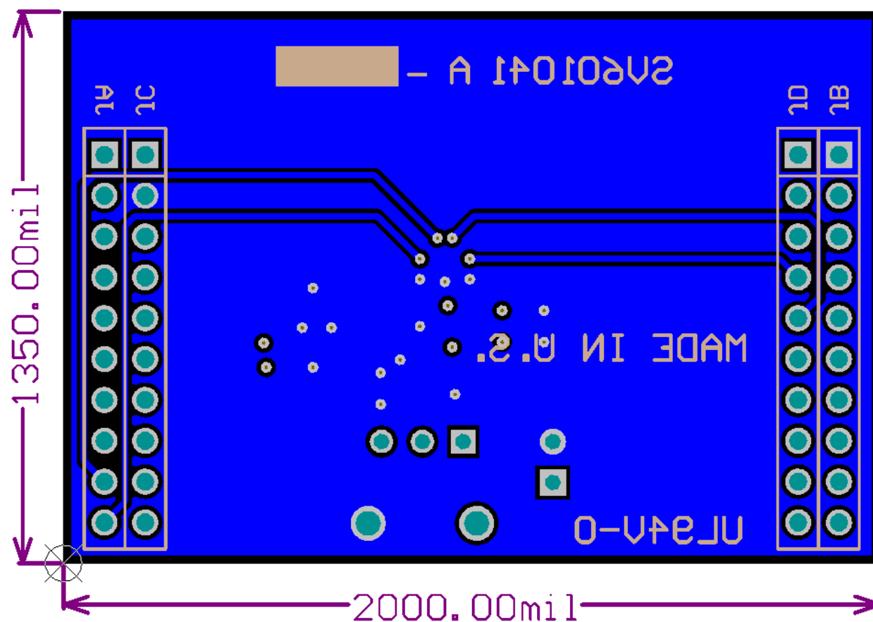
Figure 4-6. Bottom Assembly
