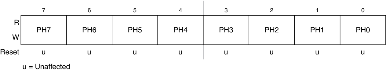
Figure 8-8. Carrier Generator Data Register High 1(CMTCGH1)
