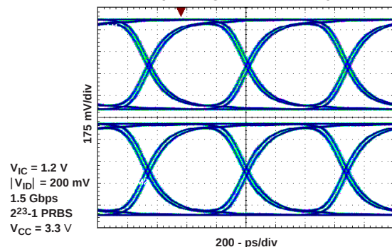
Eye Pattern of Two Outputs Operating Simultaneously
