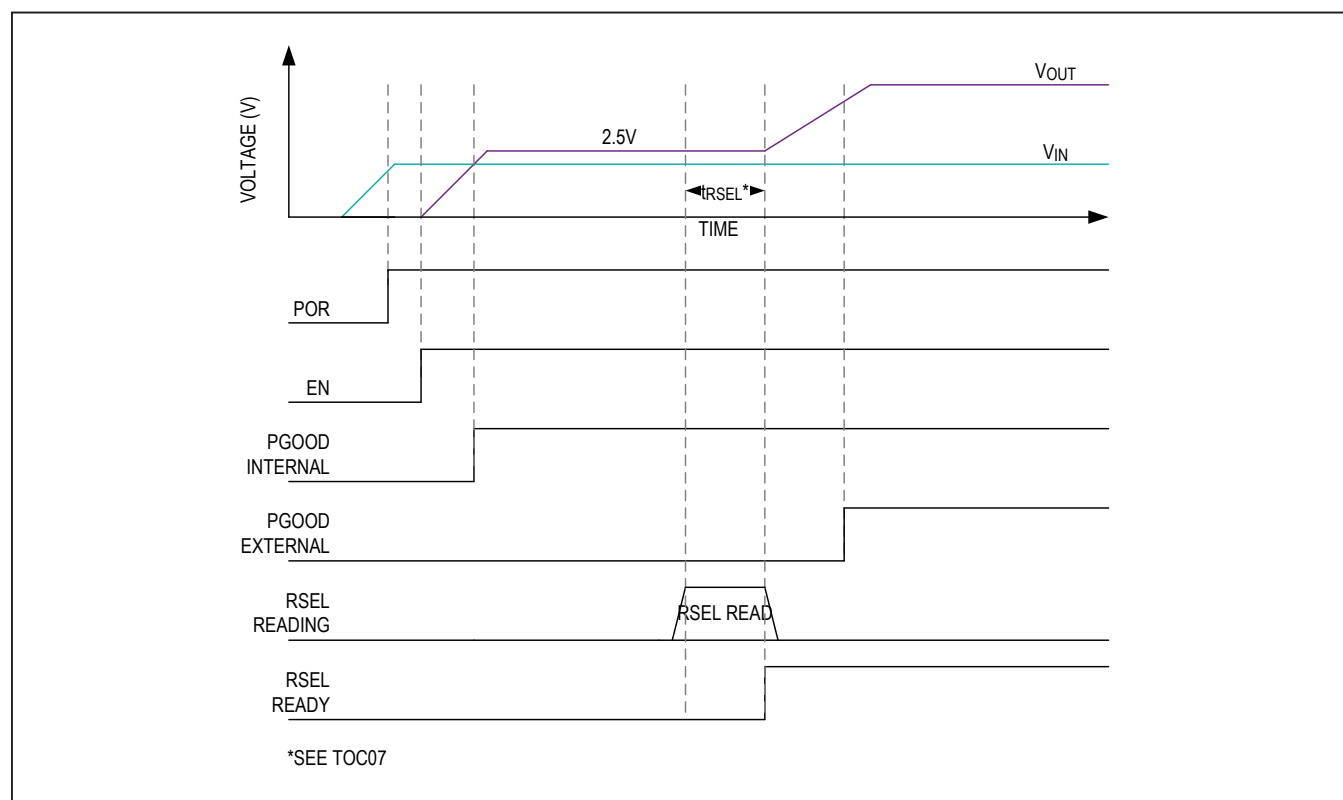
Figure 8. MAX20343 RSEL Startup Sequence
