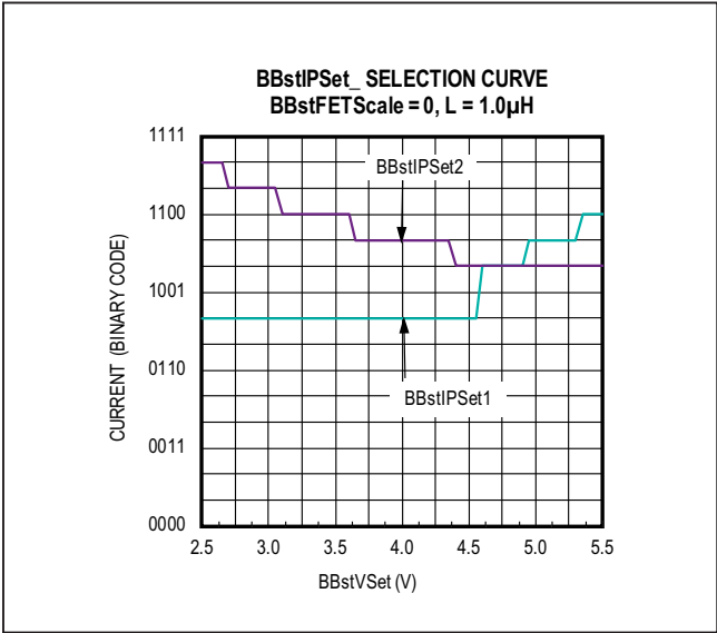
Figure 6. Recommended BBstIPSet1 and BBstIPSet2 Settings for BBstFETScale = 0 (MAX20343B Only)
