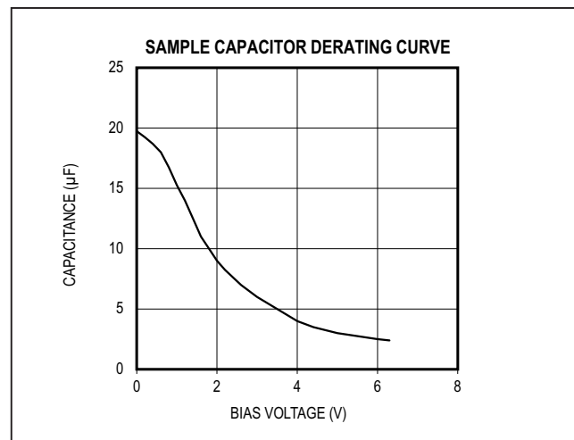
Figure 9. Capacitor Derating for Input and Output Capacitance
