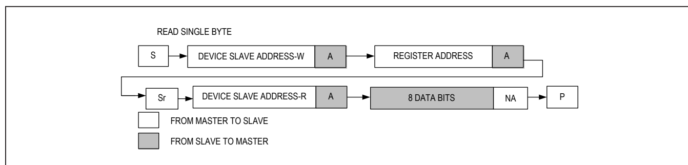
Figure 13. Read Byte Sequence
