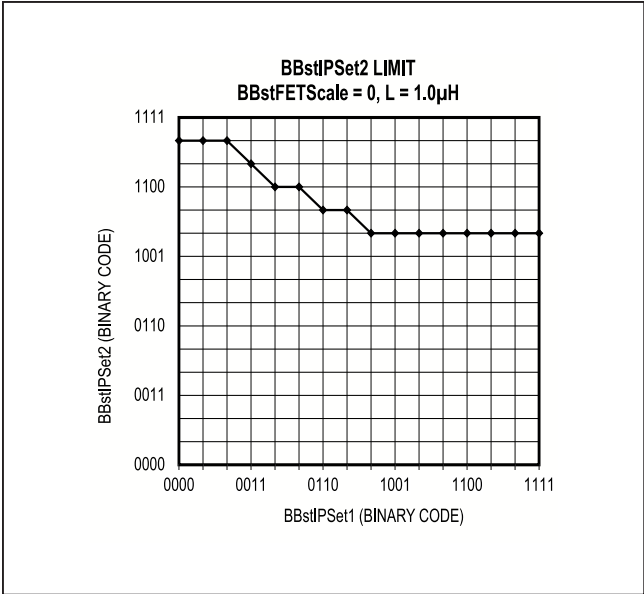
Figure 4. Minimum BBstIPSet2 Limit for a Given BBstIPSet1 Setting for BBstFETScale = 0 (MAX20343B Only)
