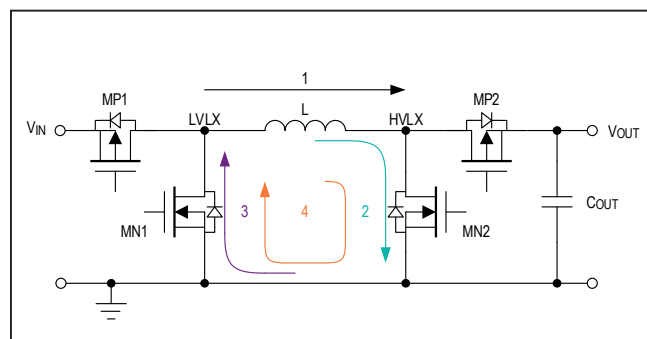
Figure 1. The Buck-Boost Regulator and Switching Phases
