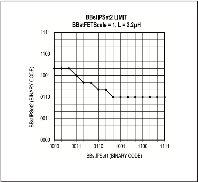
Figure 5. Minimum BBstIPSet2 Limit for a Given BBstIPSet1 Setting for BBstFETScale = 1 (on MAX20343B, and for either BBstFETScale setting for all other versions)
