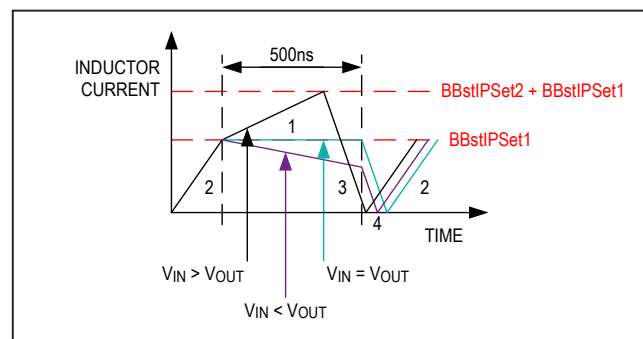
Figure 2. Buck-Boost Inductor Current in Buck-Boost Mode
