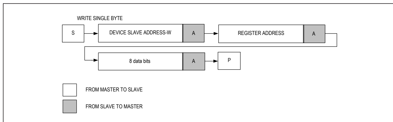
Figure 11. Write Byte Sequence
