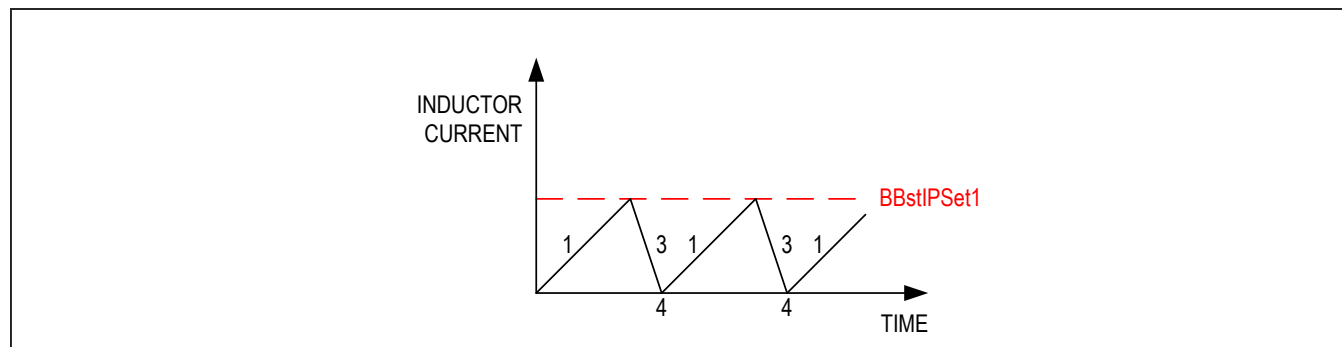
Figure 3. Buck-Boost Inductor Current in Buck-Only Mode
