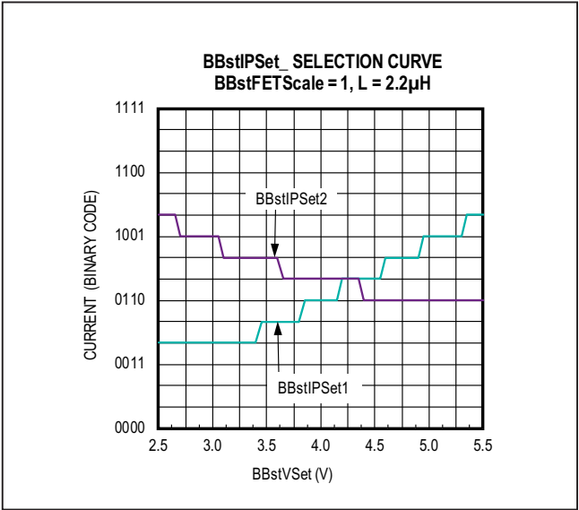
Figure 7. Recommended BBstIPSet1 and BBstIPSet2 Settings for BBstFETScale = 1 (on MAX20343B, and for either BBstFETScale setting for all other versions)
