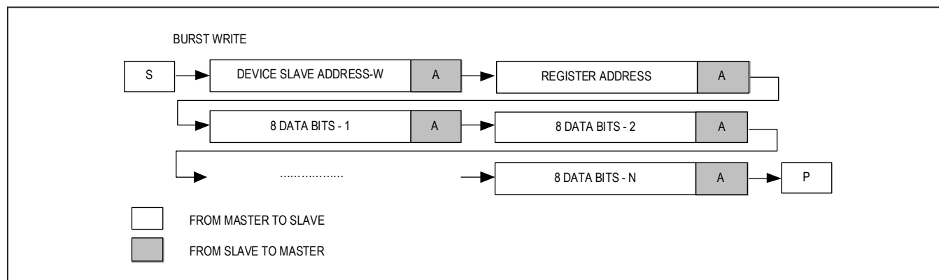
Figure 12. Burst Write Sequence
