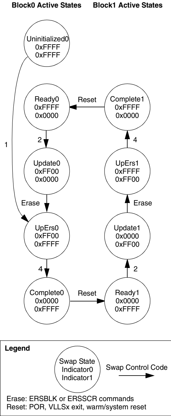
Figure 28-35. Valid Swap State Sequencing
