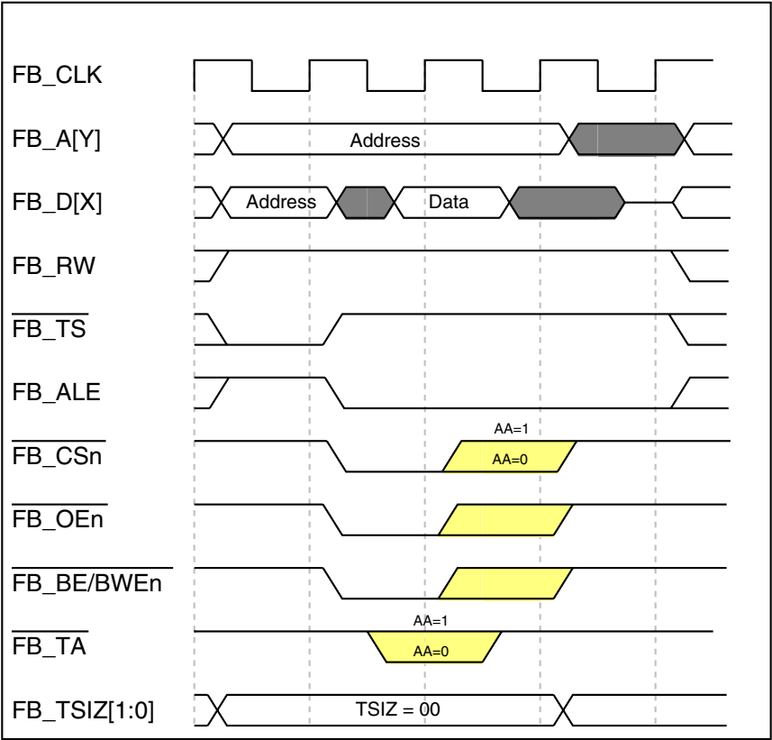
Figure 29-34. Longword-Read Transfer
