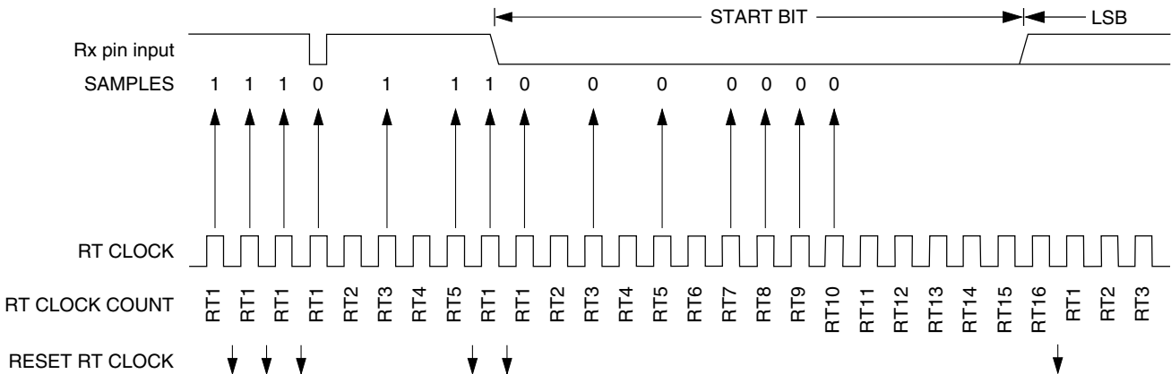
Figure 48-191. Start bit search example 1 ( C7816[ISO\_7816E] = 0 )
