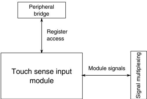
Figure 3-63. TSI configuration
