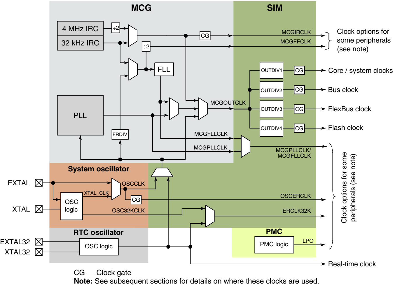
Figure 5-1. Clocking diagram
