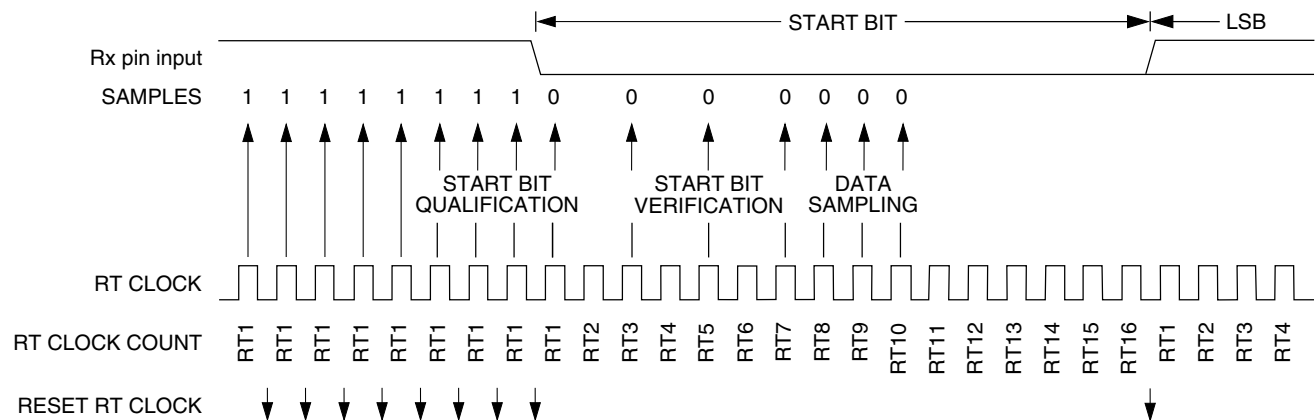
Figure 48-190. Receiver data sampling
