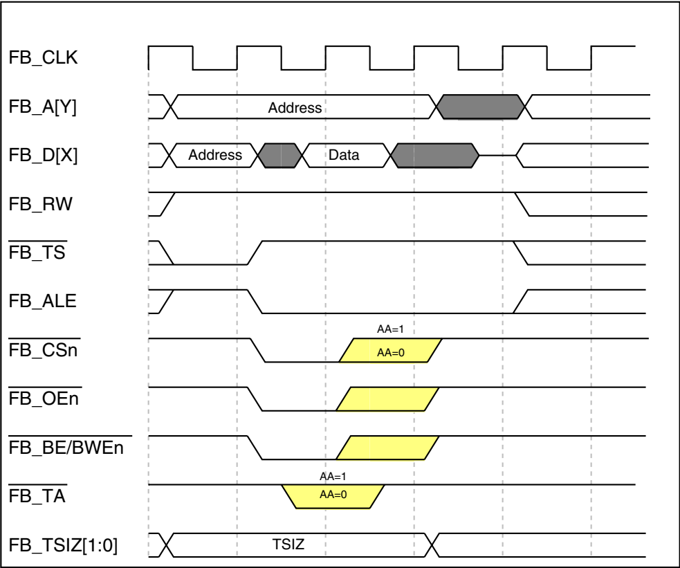
Figure 29-36. Basic Read-Bus Cycle (No Wait States)
