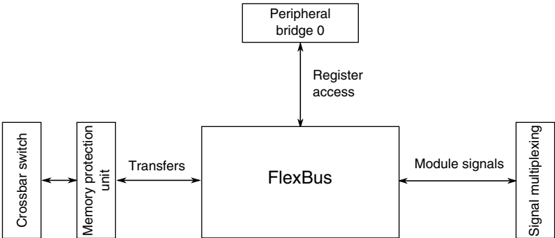
Figure 3-31. FlexBus configuration
