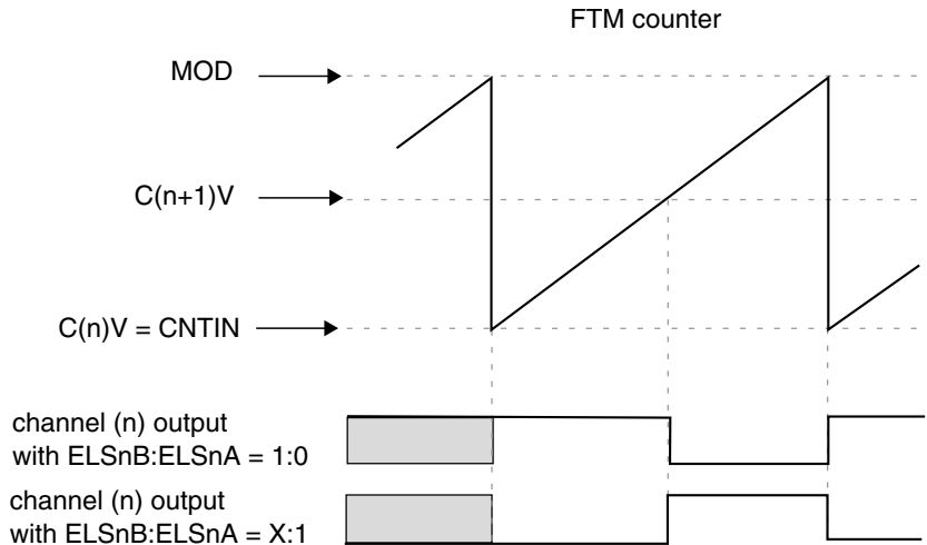
Figure 37-190. Channel (n) Output If (C(n)V = CNTIN) and (CNTIN < C(n+1)V < MOD)
