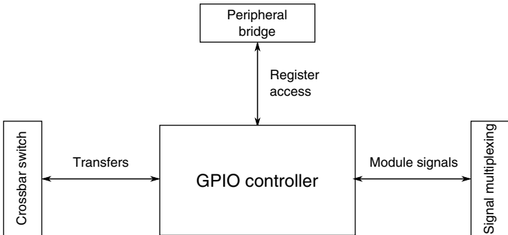
Figure 3-62. GPIO configuration
