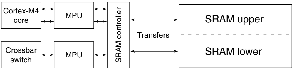
Figure 3-24. SRAM configuration
