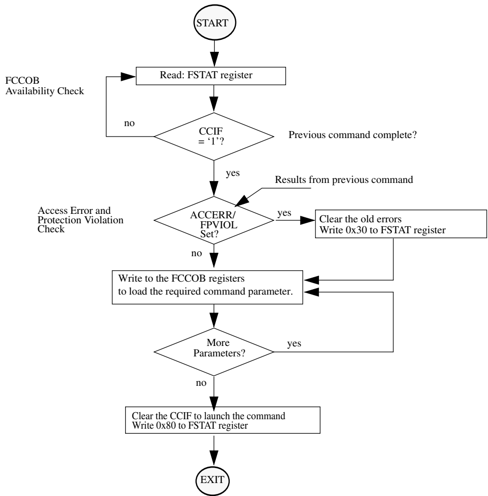
Figure 28-33. Generic FTFL Command Write Sequence Flowchart
