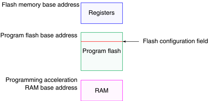
Figure 4-2. Flash memory map for devices containing only program flash
