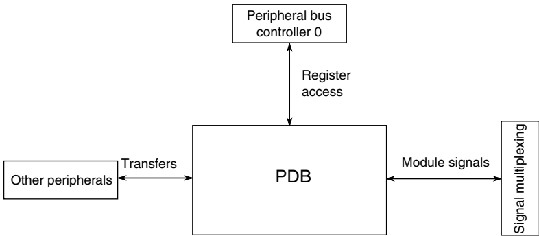
Figure 3-41. PDB configuration
