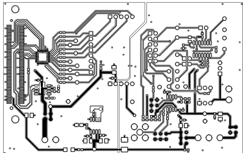
Figure 15. Component Placement Drawing of Motherboard
