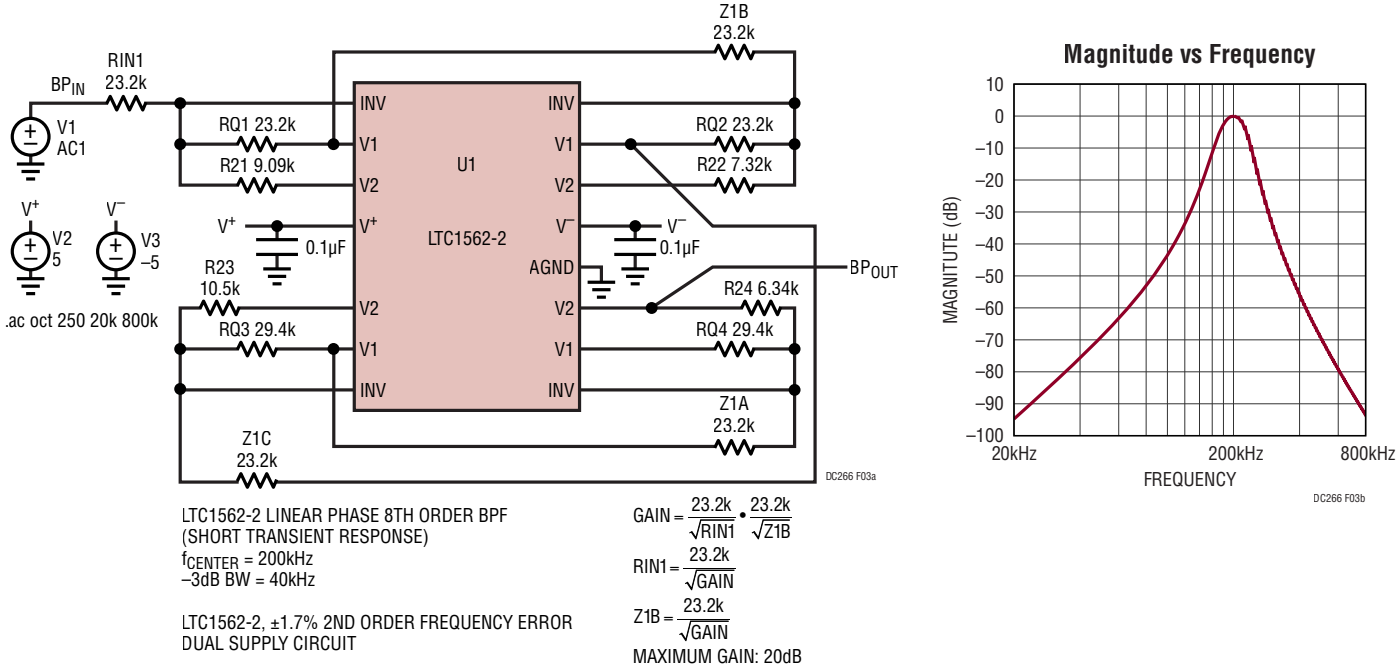
Figure 3. The Default DC266B-B Circuit
