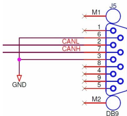
Figure 5: CAN DB9 connector Pin out
