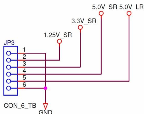
Figure 20: Terminal power input connections
