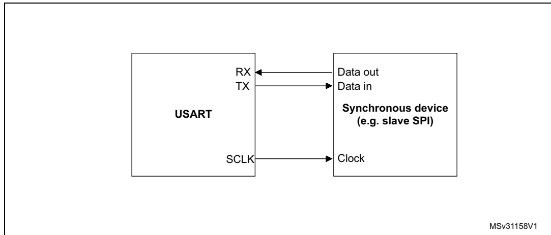
Figure 325. USART example of synchronous master transmission
