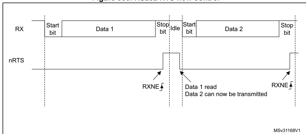
Figure 350. RS232 RTS flow control
