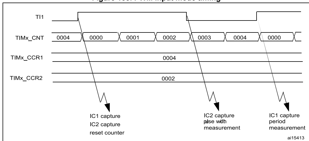
Figure 188. PWM input mode timing
