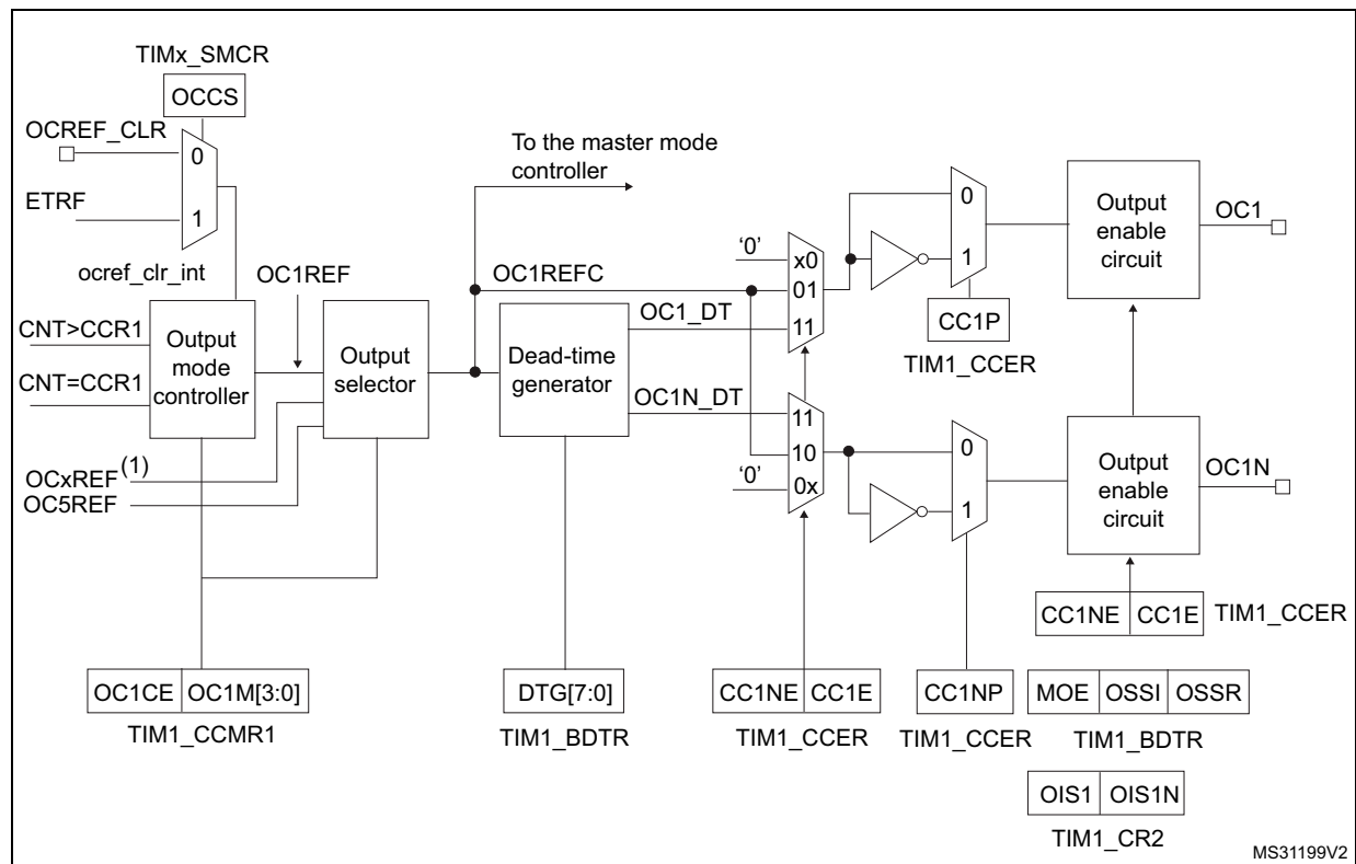
Figure 130. Output stage of capture/compare channel (channel 1, idem ch. 2 and 3)
