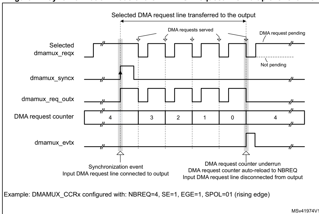
Figure 22. Synchronization mode of the DMAMUX request line multiplexer channel
