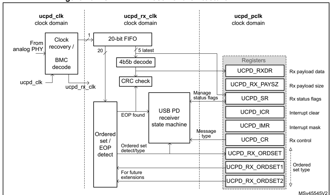
Figure 401. UCPD BMC receiver architecture
