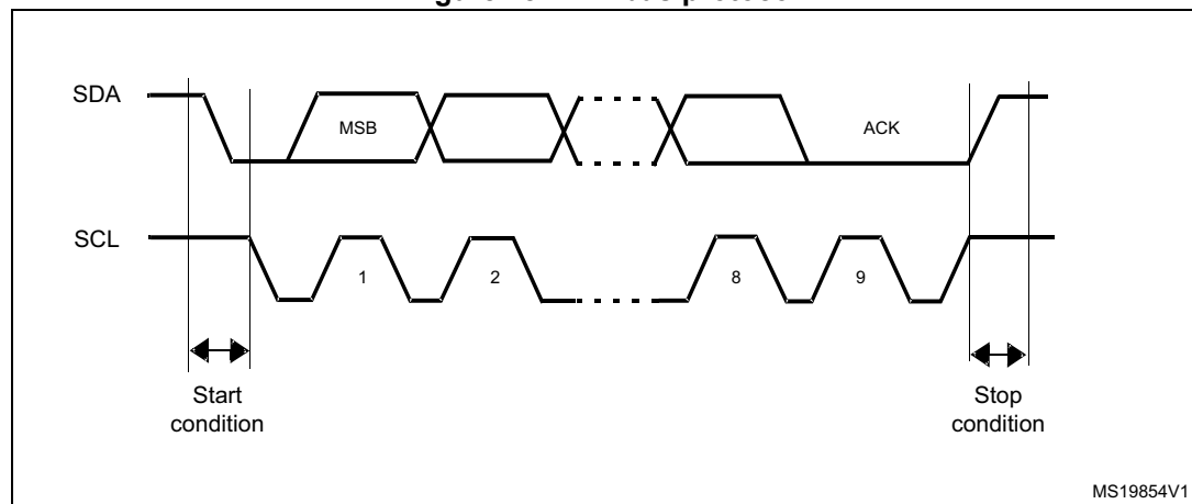
Figure 284. I 2 C bus protocol
