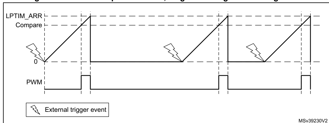
Figure 271. LPTIM output waveform, single counting mode configuration
