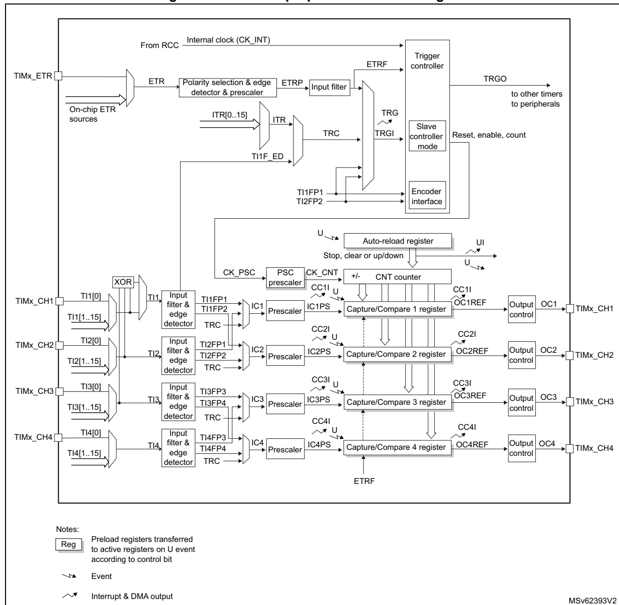
Figure 160. General-purpose timer block diagram
