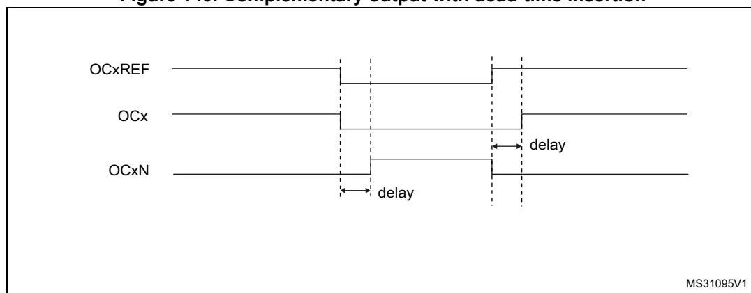
Figure 140. Complementary output with dead-time insertion
