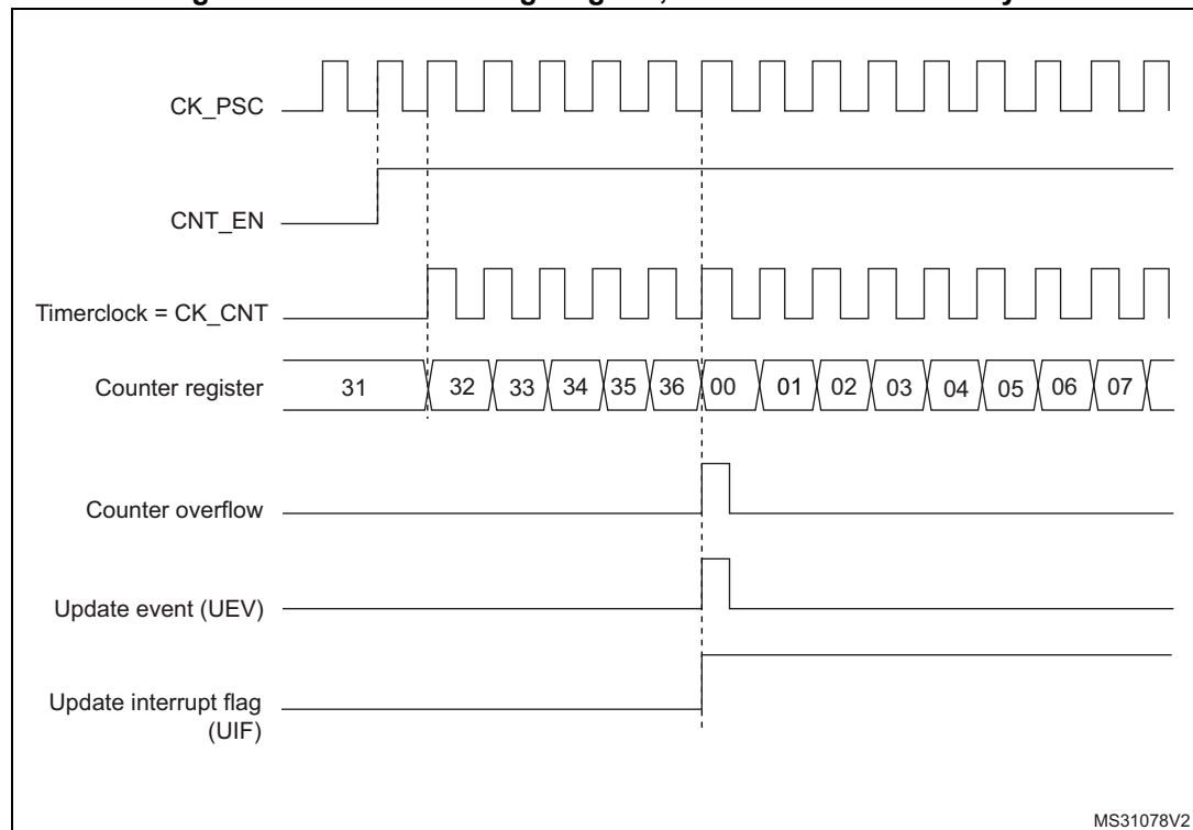
Figure 213. Counter timing diagram, internal clock divided by 1
