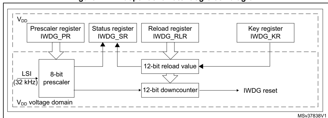
Figure 277. Independent watchdog block diagram
