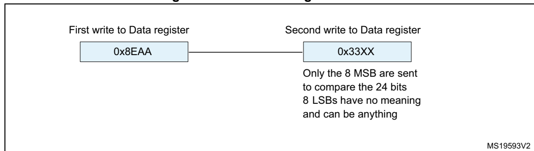
Figure 373. Transmitting 0x8EAA33
