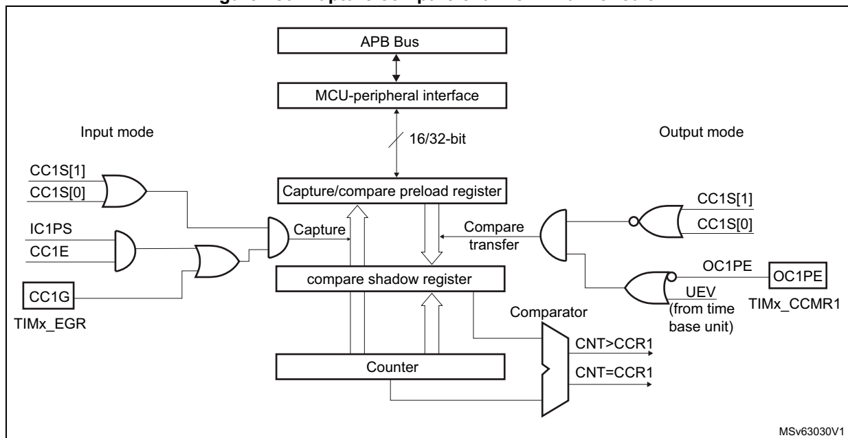
Figure 250. Capture/compare channel 1 main circuit
