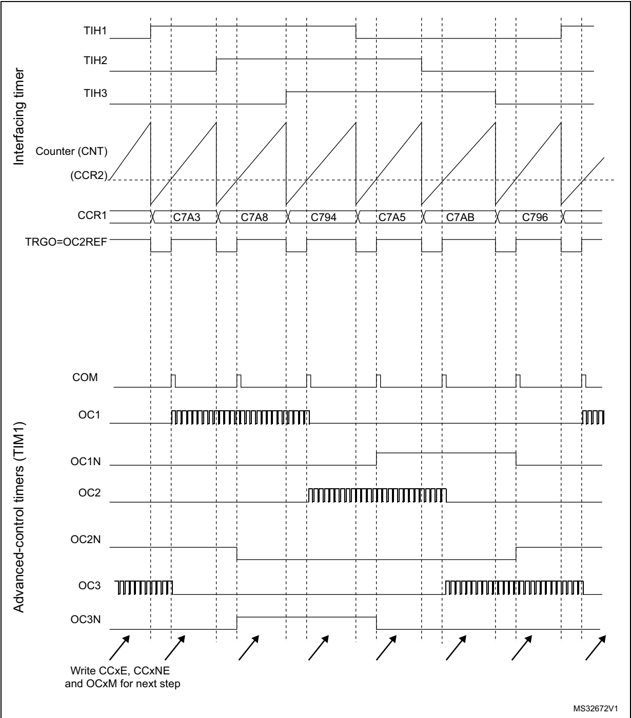
Figure 155. Example of Hall sensor interface
