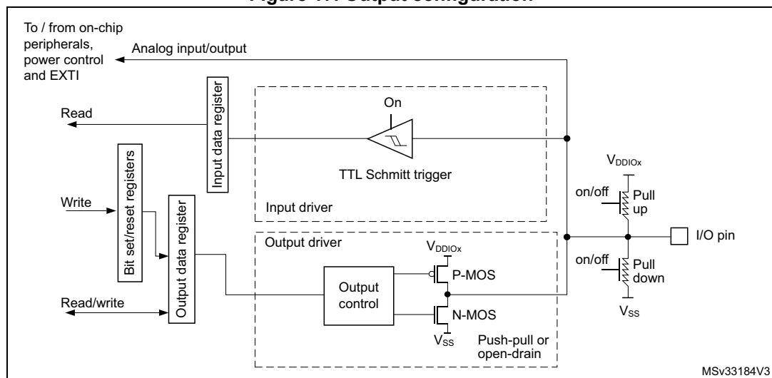
Figure 17. Output configuration
