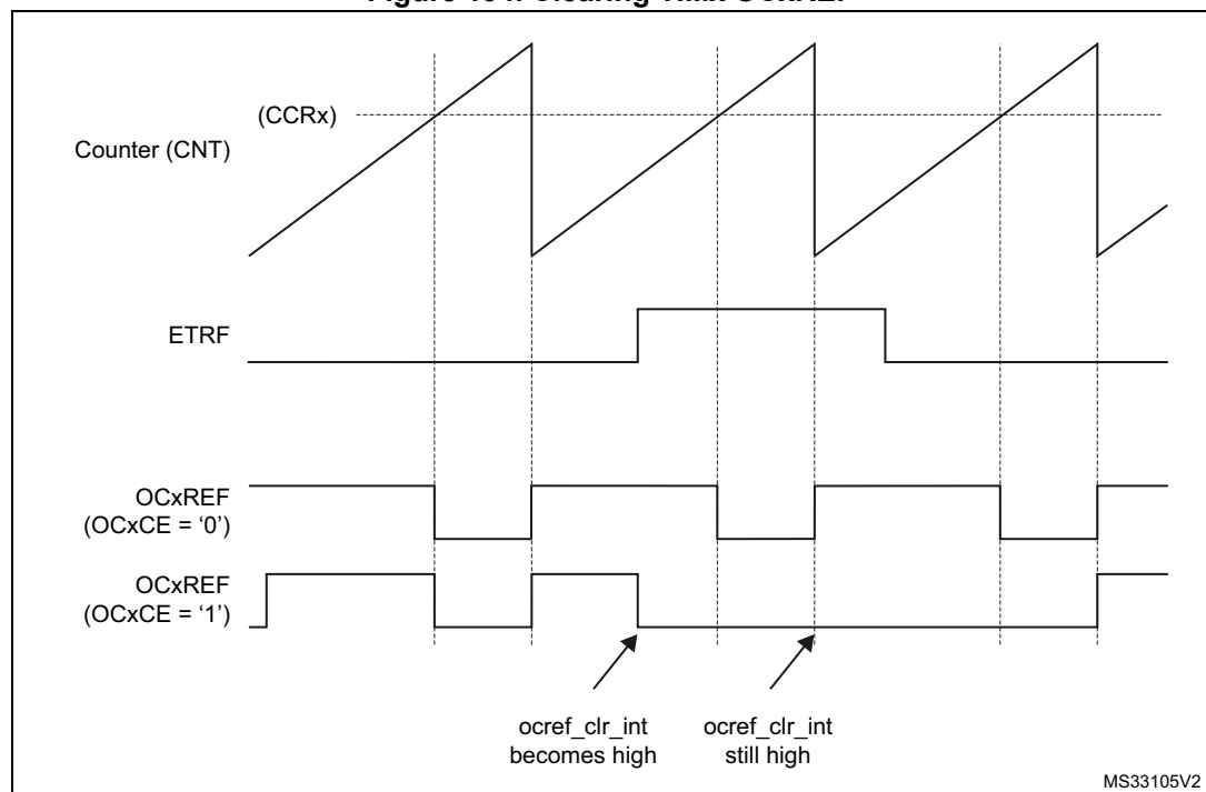
Figure 194. Clearing TIMx OCxREF
