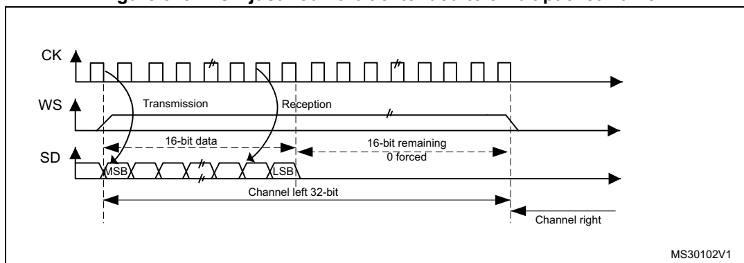
Figure 379. MSB justified 16-bit extended to 32-bit packet frame
