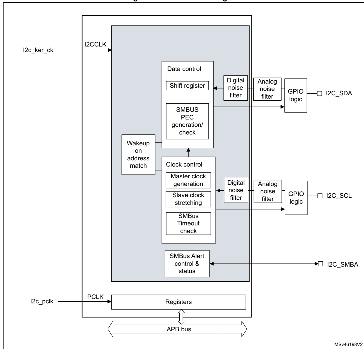
Figure 282. I2C1 block diagram
