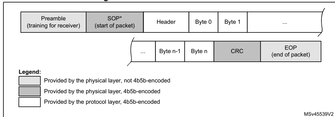
Figure 395. Packet format
