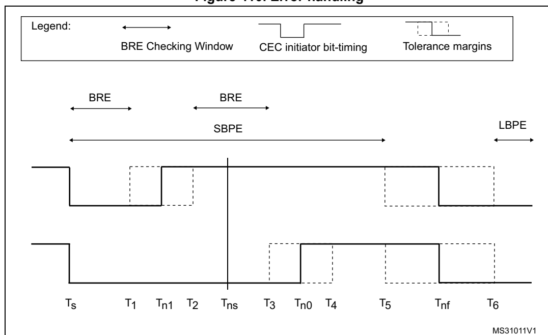
Figure 410. Error handling
