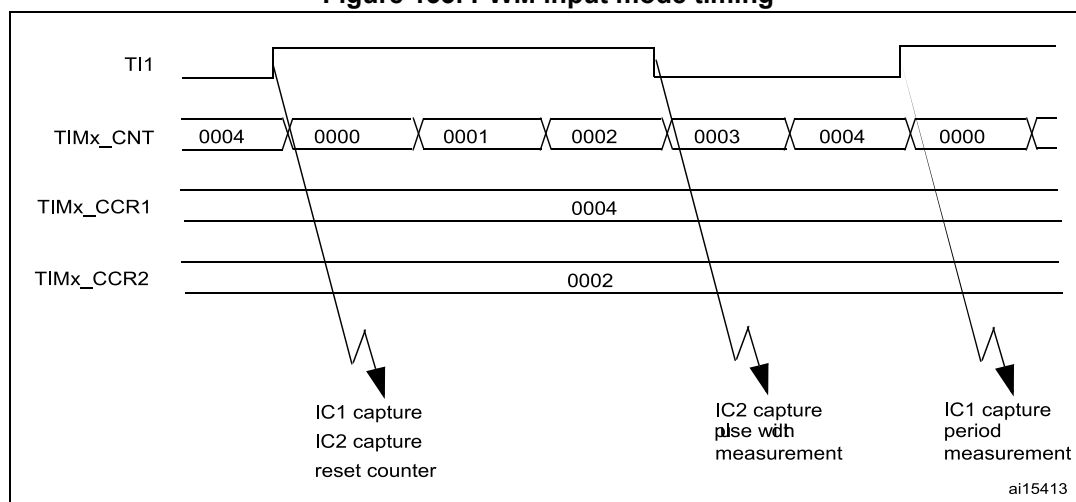
Figure 133. PWM input mode timing
