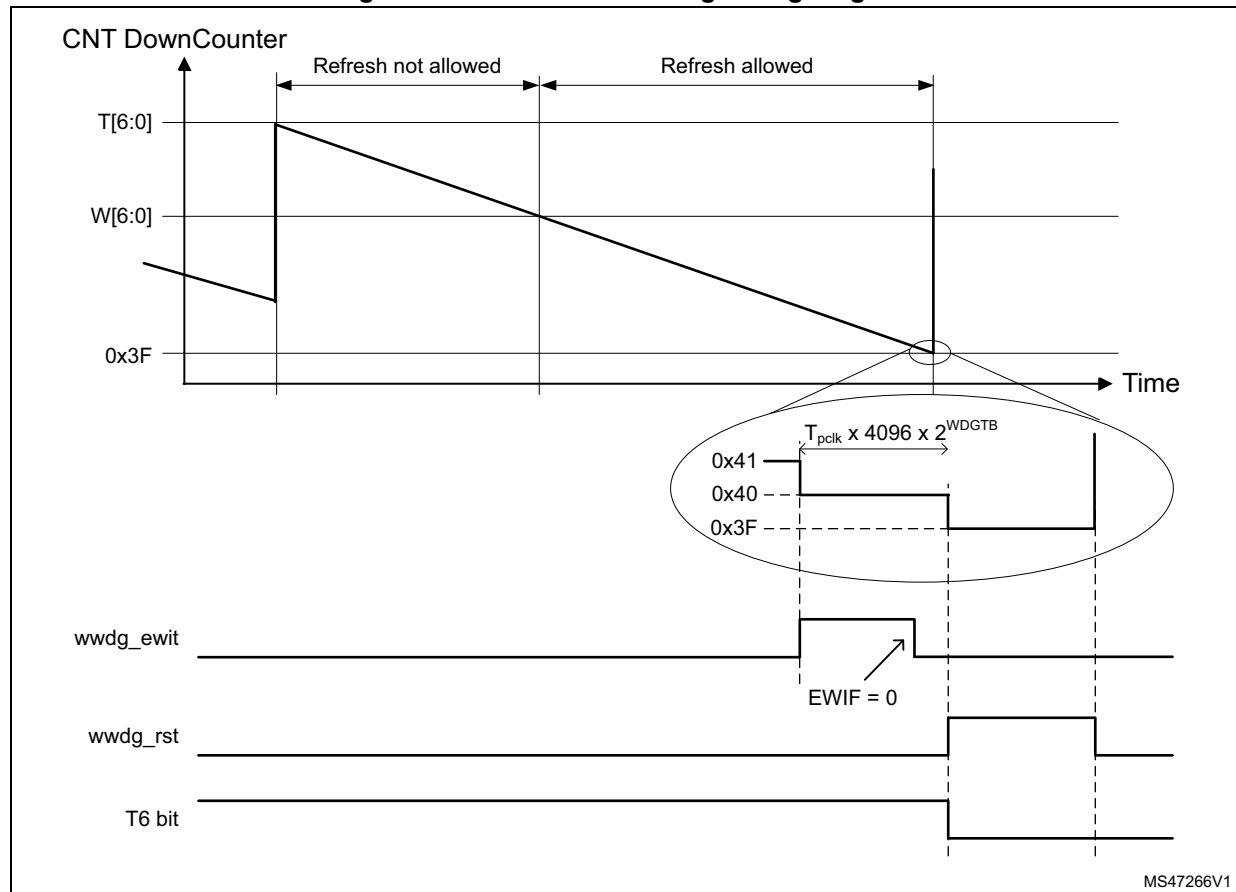
Figure 279. Window watchdog timing diagram
