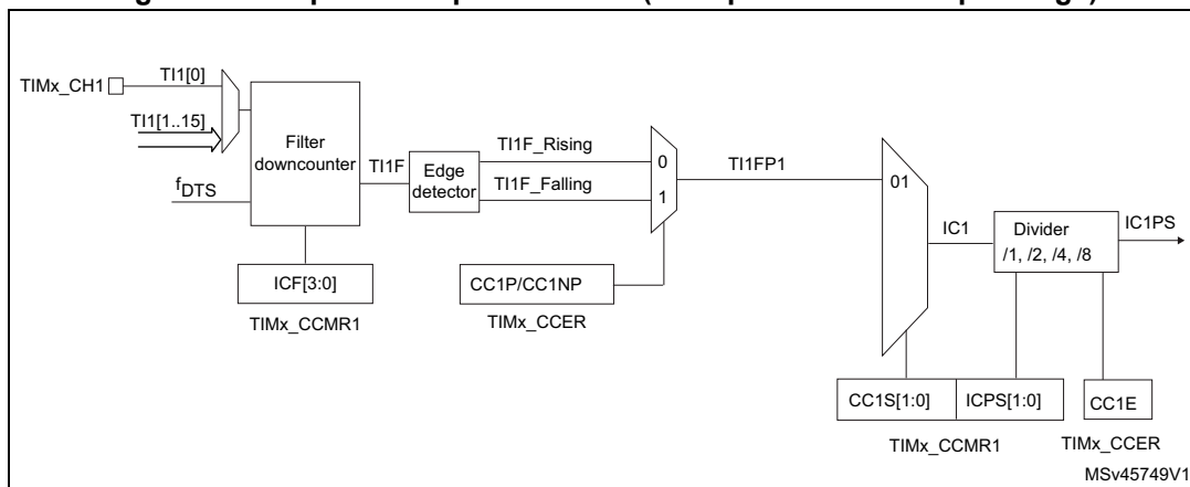
Figure 230. Capture/compare channel (example: channel 1 input stage)
