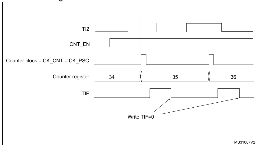
Figure 248. Control circuit in external clock mode 1
