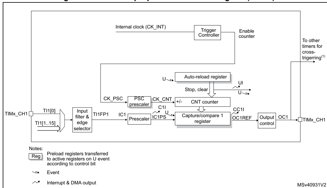
Figure 220. General-purpose timer block diagram (TIM14)
