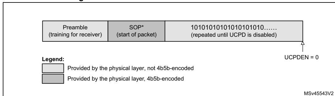
Figure 399. BIST Carrier Mode 2 frame
