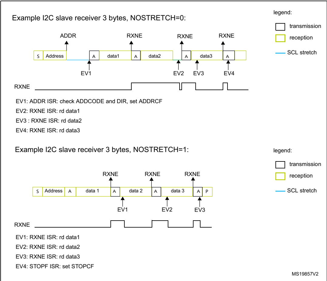
Figure 295. Transfer bus diagrams for I2C slave receiver
