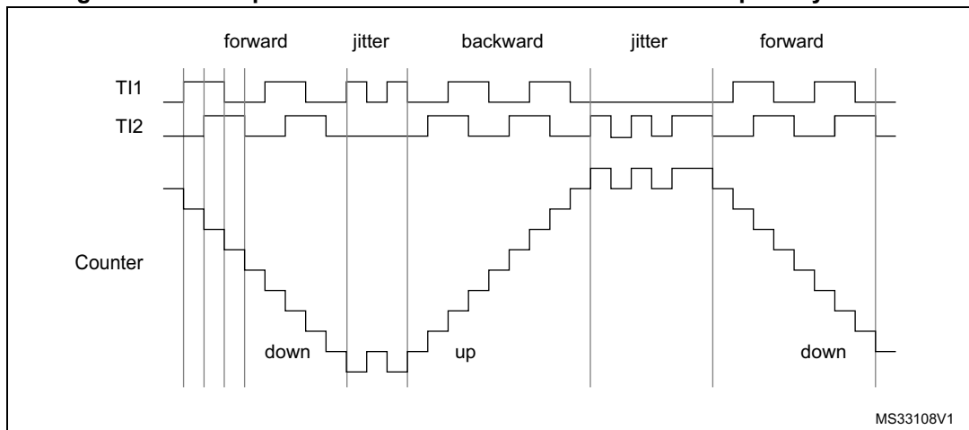
Figure 198. Example of encoder interface mode with TI1FP1 polarity inverted
