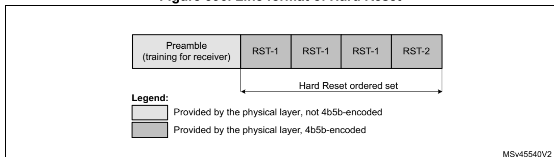
Figure 396. Line format of Hard Reset
