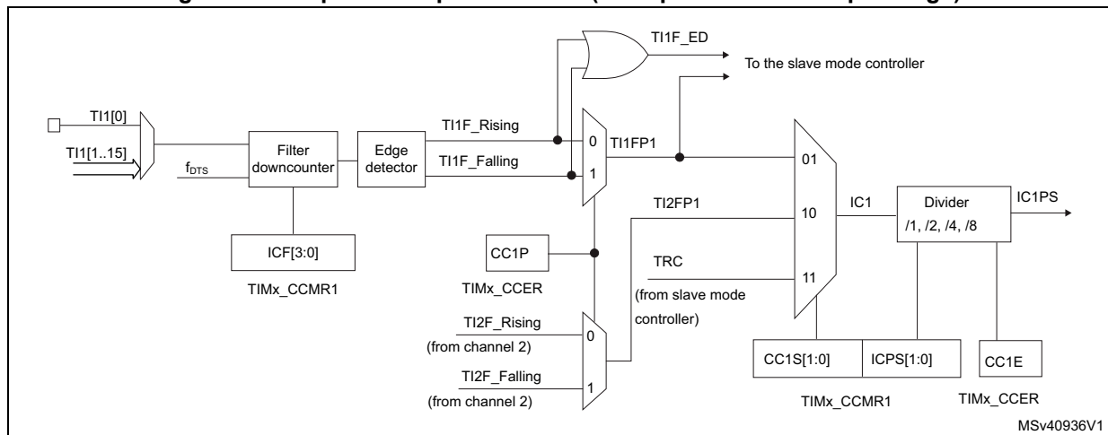
Figure 249. Capture/compare channel (example: channel 1 input stage)
