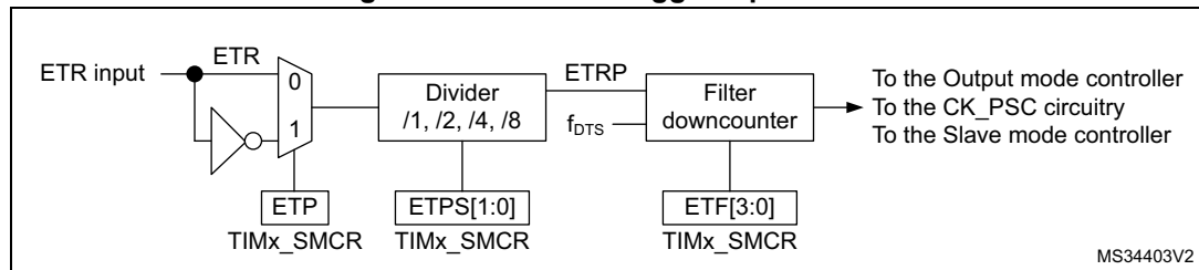
Figure 121. External trigger input block
