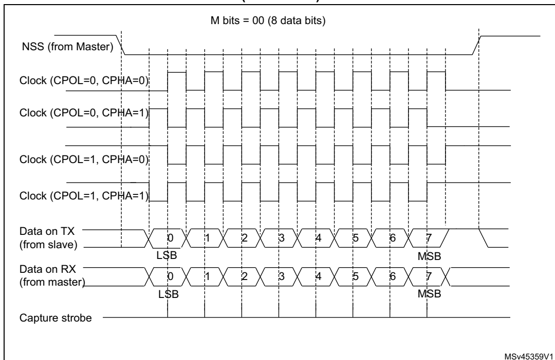
Figure 328. USART data clock timing diagram in synchronous slave mode (M bits = 00)
