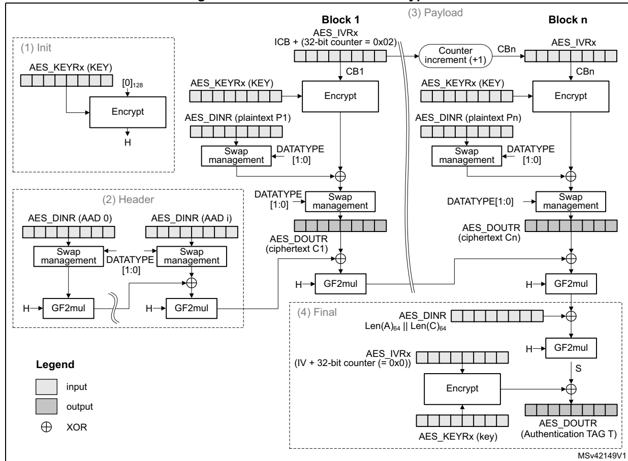
Figure 92. GCM authenticated encryption
