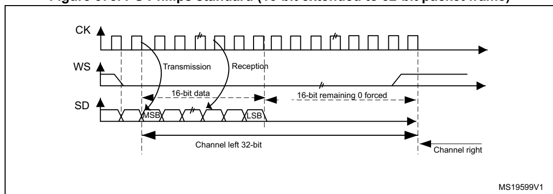
Figure 375. I 2 S Philips standard (16-bit extended to 32-bit packet frame)
