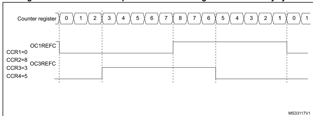
Figure 192. Generation of 2 phase-shifted PWM signals with 50% duty cycle
