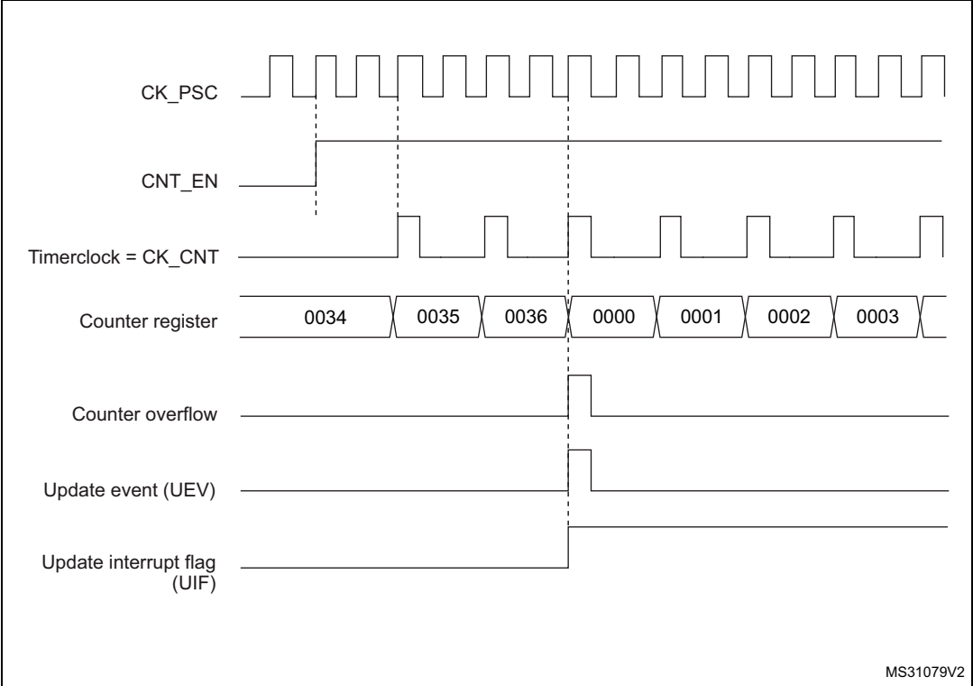
Figure 240. Counter timing diagram, internal clock divided by 2
