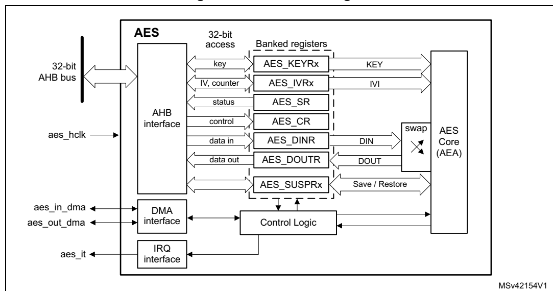
Figure 73. AES block diagram
