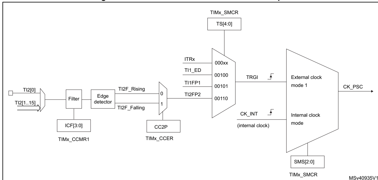
Figure 247. TI2 external clock connection example
