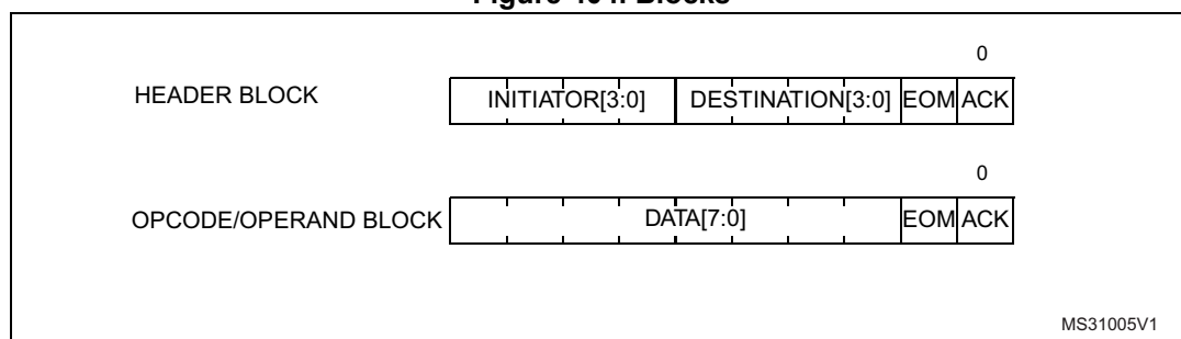
Figure 404. Blocks
