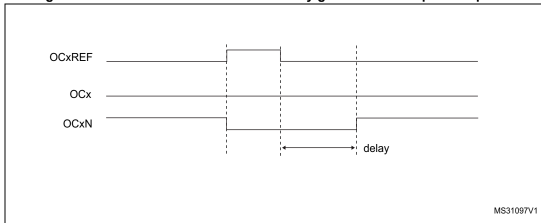
Figure 259. Dead-time waveforms with delay greater than the positive pulse.
