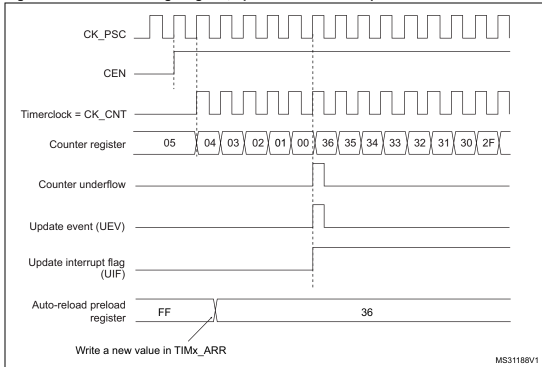
Figure 113. Counter timing diagram, update event when repetition counter is not used
