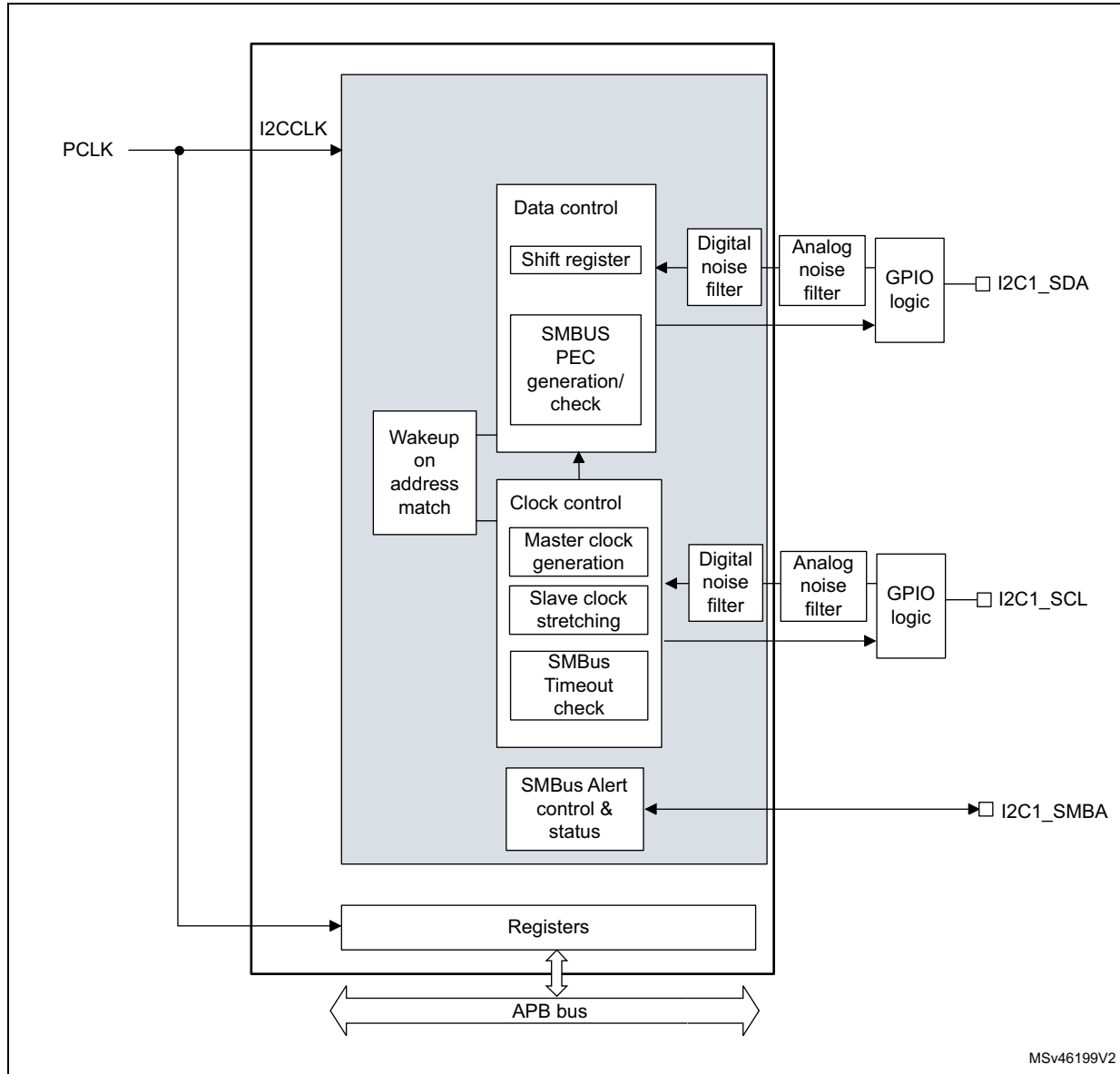
Figure 283. I2C2 block diagram
