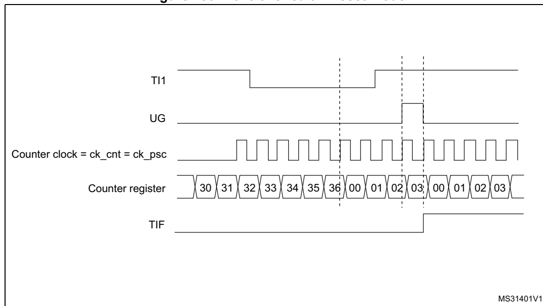
Figure 156. Control circuit in reset mode
