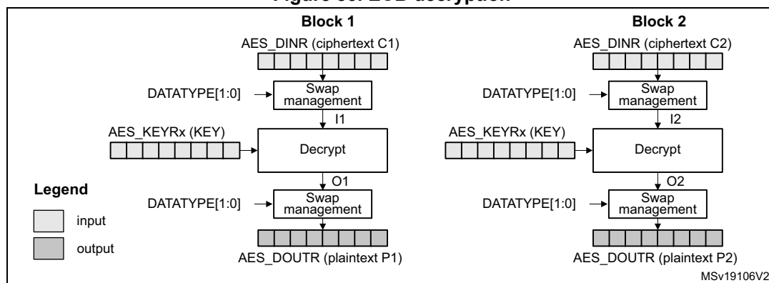
Figure 83. ECB decryption
