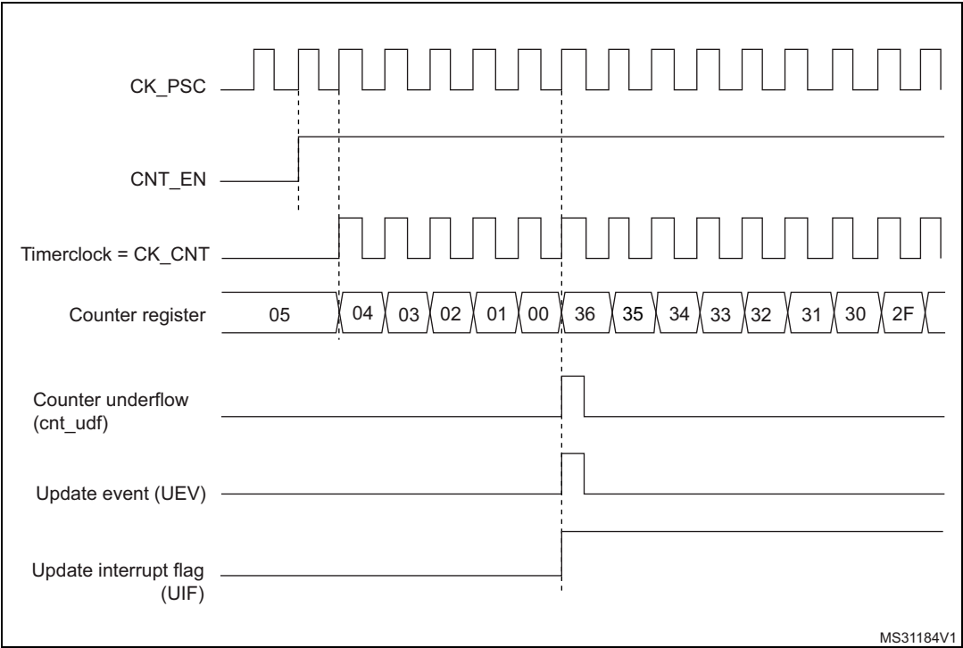
Figure 169. Counter timing diagram, internal clock divided by 1
