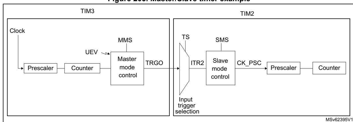
Figure 203. Master/Slave timer example
