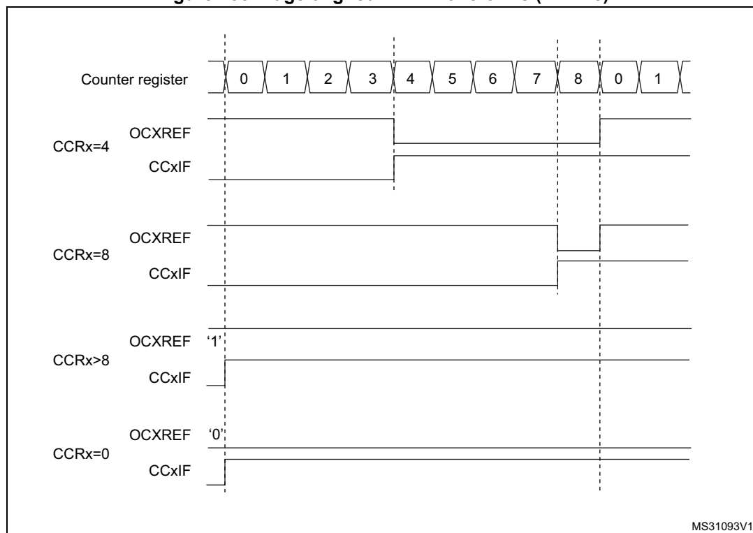
Figure 255. Edge-aligned PWM waveforms (ARR=8)
