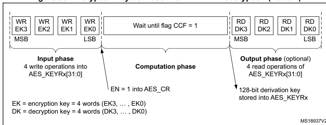
Figure 80. Encryption key derivation for ECB/CBC decryption (Mode 2)
