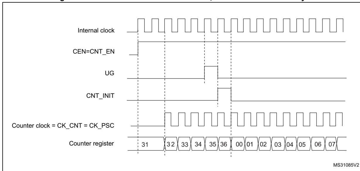
Figure 246. Control circuit in normal mode, internal clock divided by 1
