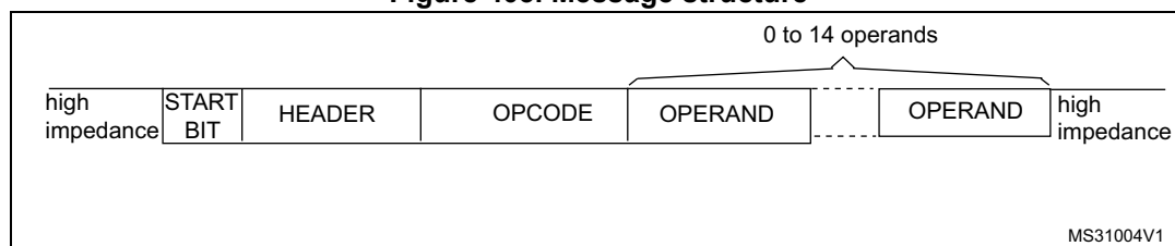
Figure 403. Message structure
