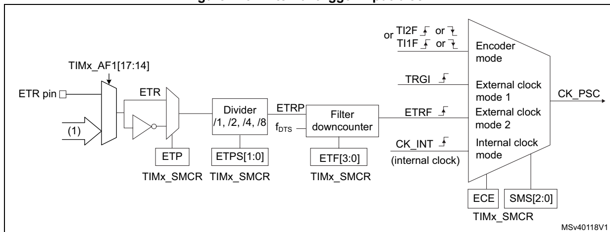
Figure 126. External trigger input block
