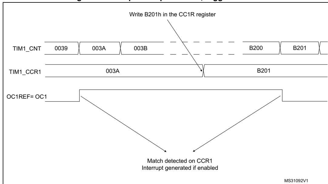
Figure 233. Output compare mode, toggle on OC1.
