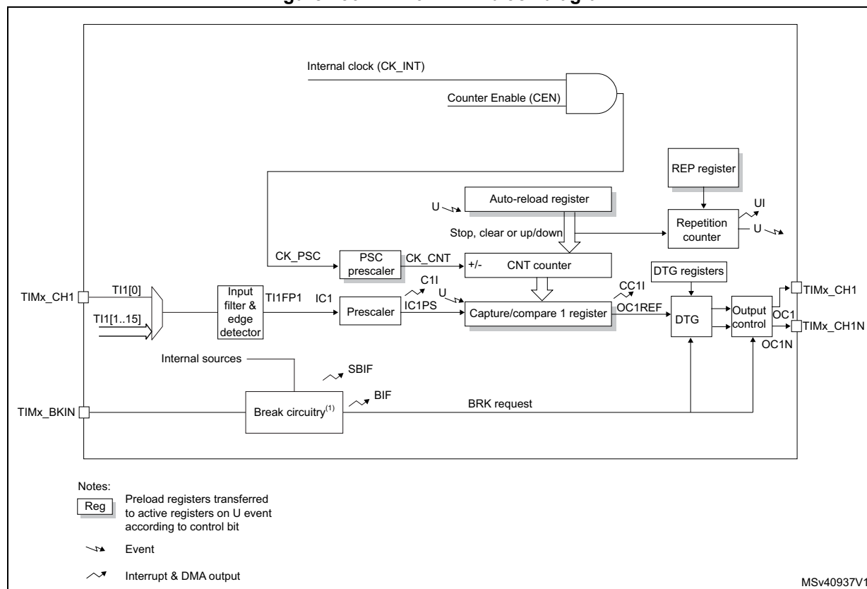
Figure 236. TIM16/TIM17 block diagram
