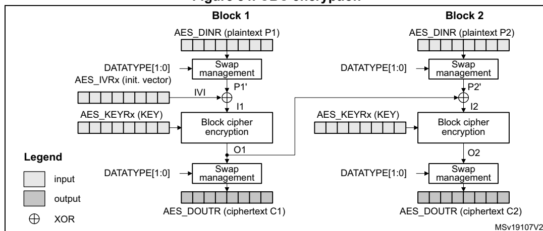
Figure 84. CBC encryption
