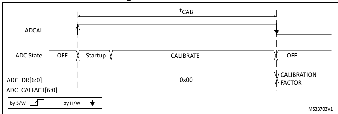
Figure 30. ADC calibration
