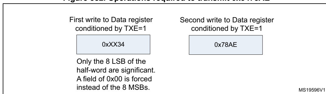
Figure 382. Operations required to transmit 0x3478AE
