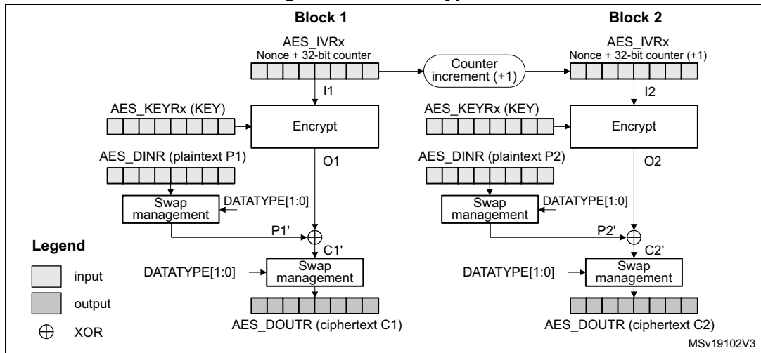
Figure 89. CTR encryption
