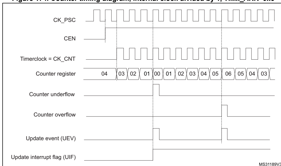
Figure 174. Counter timing diagram, internal clock divided by 1, TIMx_ARR=0x6
