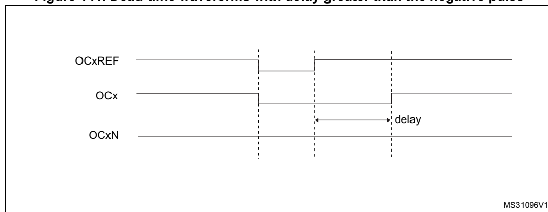
Figure 141. Dead-time waveforms with delay greater than the negative pulse
