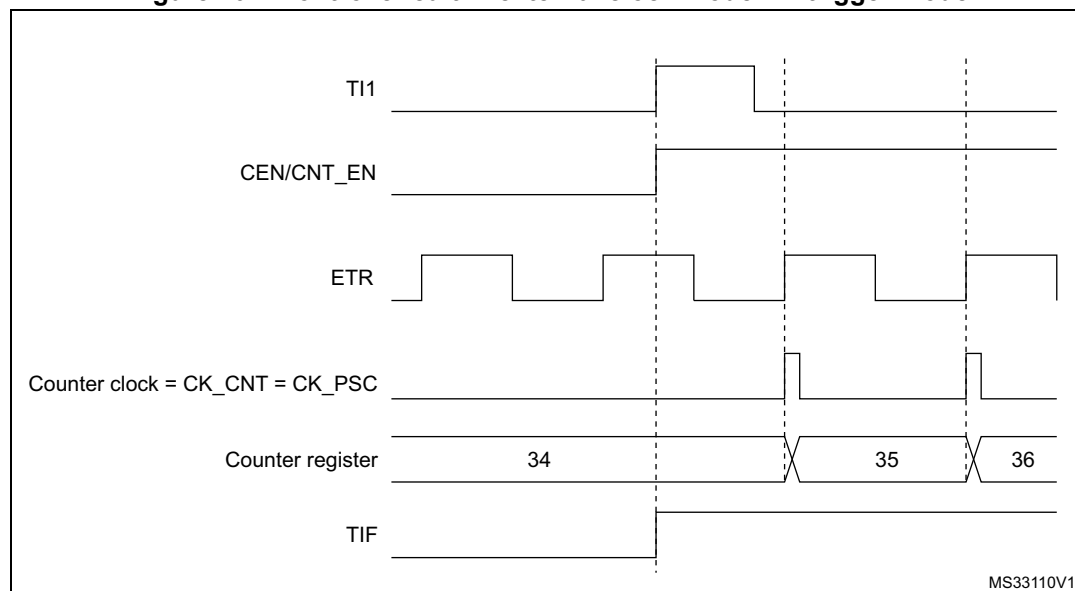
Figure 202. Control circuit in external clock mode 2 + trigger mode
