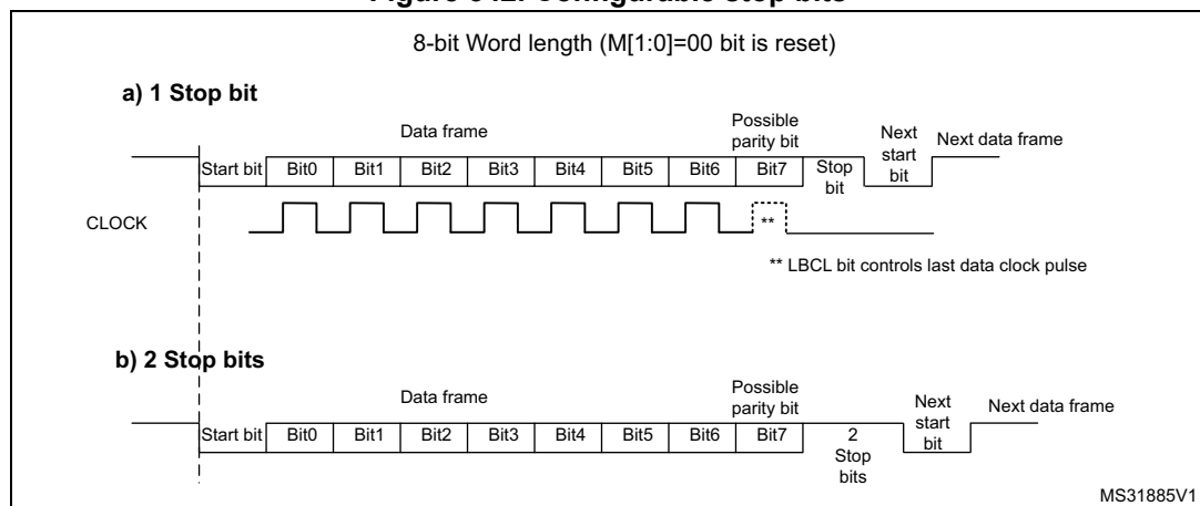
Figure 342. Configurable stop bits
