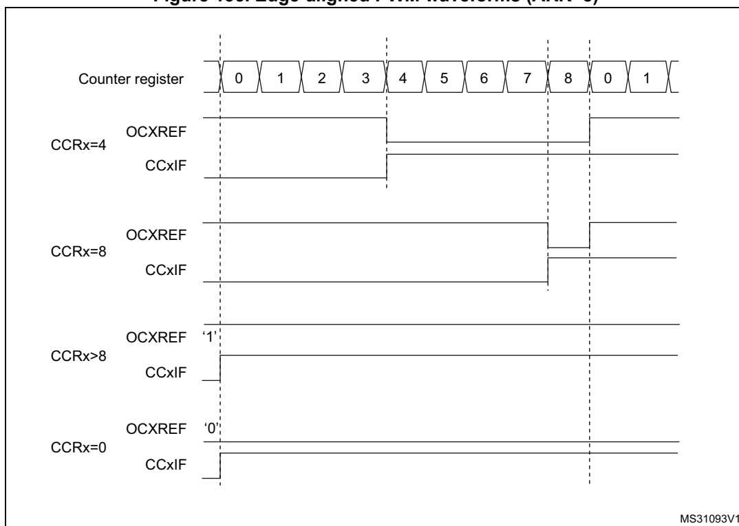
Figure 135. Edge-aligned PWM waveforms (ARR=8)
