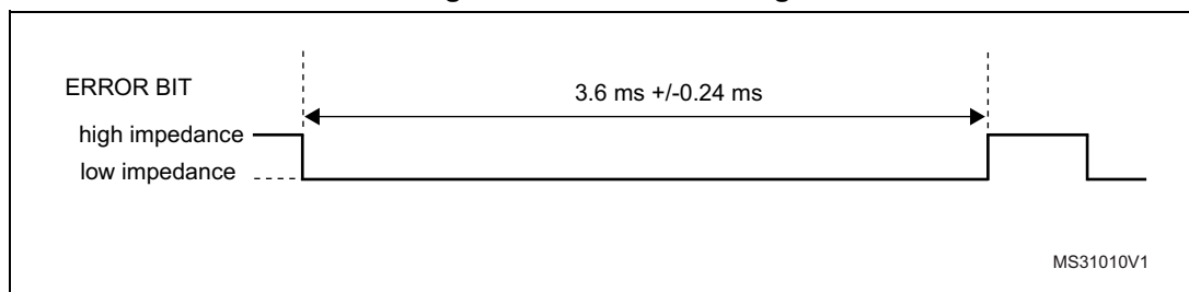
Figure 409. Error bit timing
