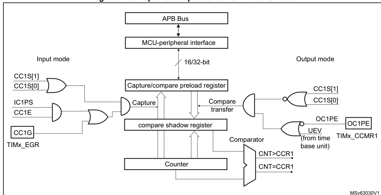
Figure 129. Capture/compare channel 1 main circuit
