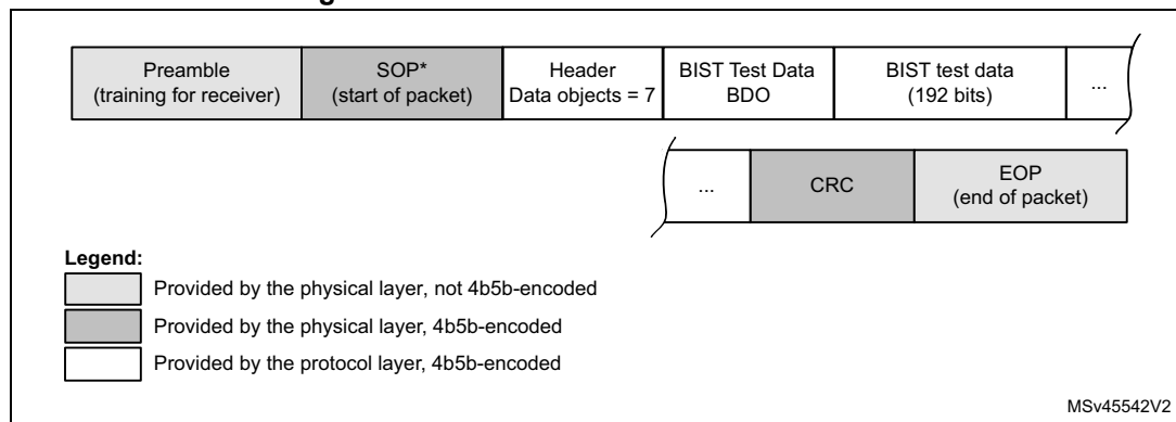
Figure 398. BIST test data frame
