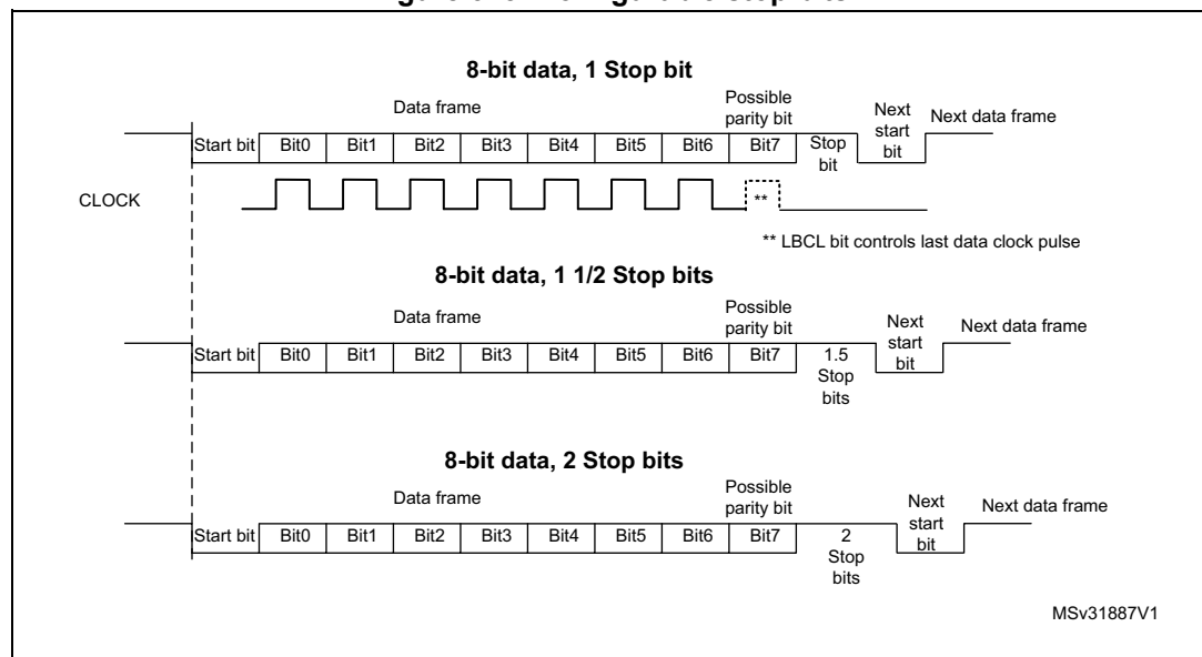
Figure 315. Configurable stop bits
