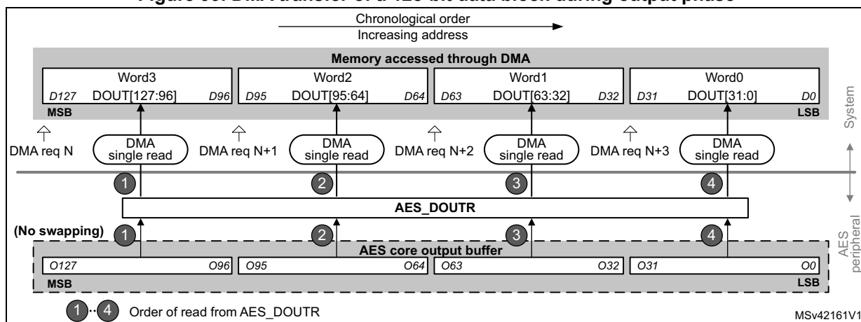
Figure 99. DMA transfer of a 128-bit data block during output phase
