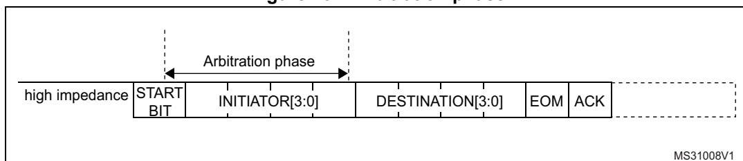
Figure 407. Arbitration phase
