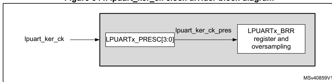
Figure 344. lpuart_ker_ck clock divider block diagram
