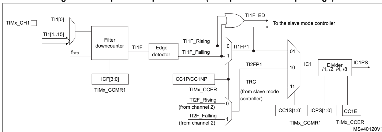
Figure 185. Capture/Compare channel (example: channel 1 input stage)
