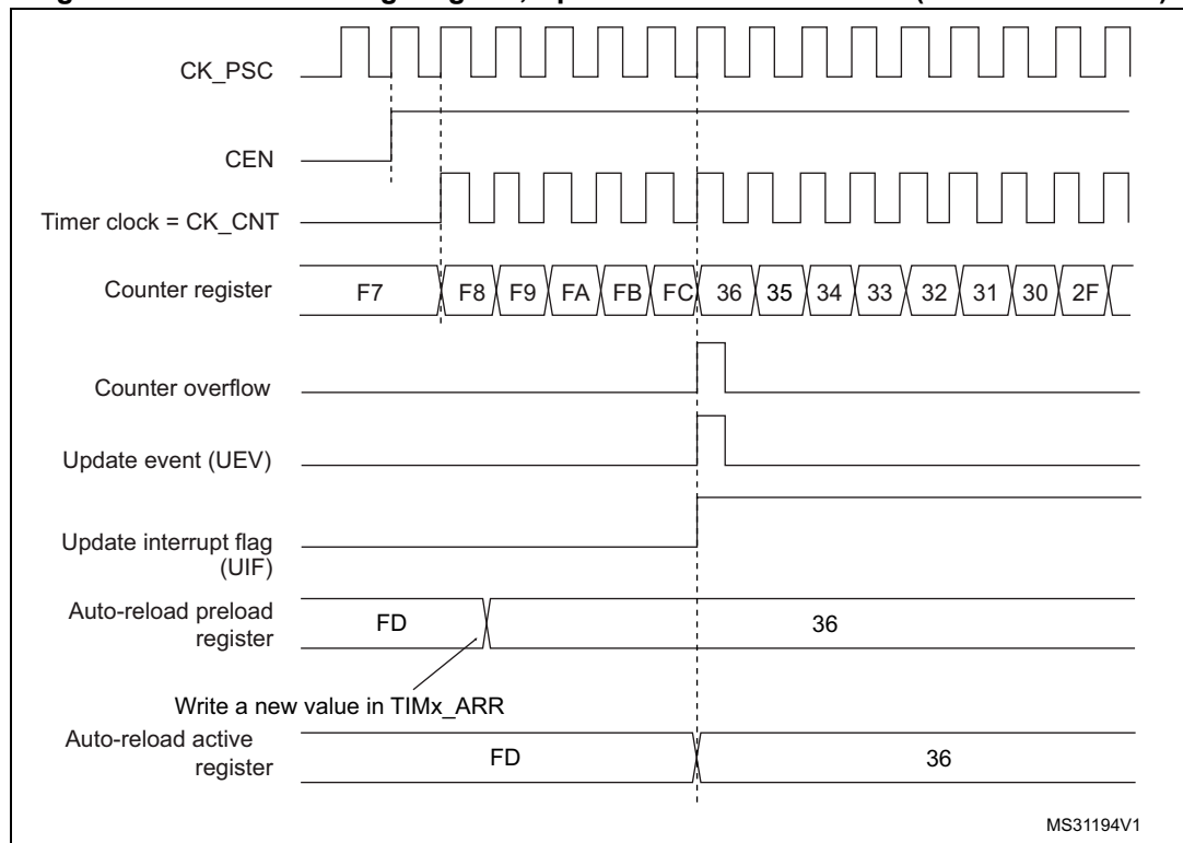
Figure 119. Counter timing diagram, Update event with ARPE=1 (counter overflow)
