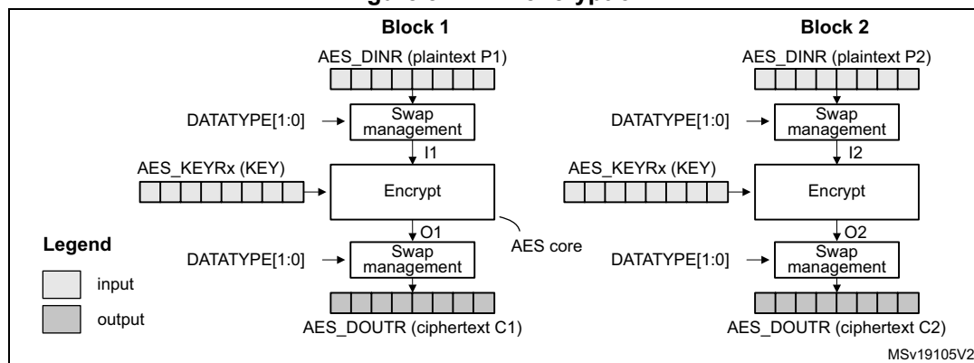
Figure 82. ECB encryption
