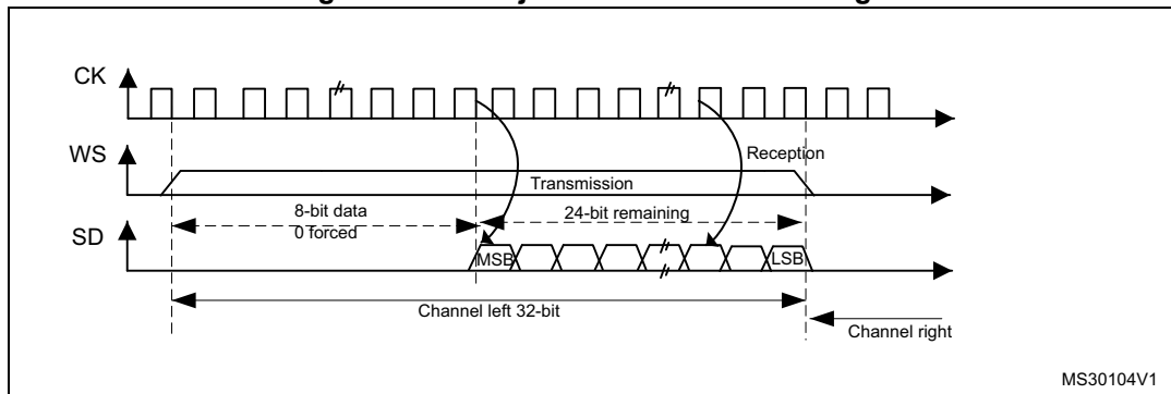
Figure 381. LSB justified 24-bit frame length
