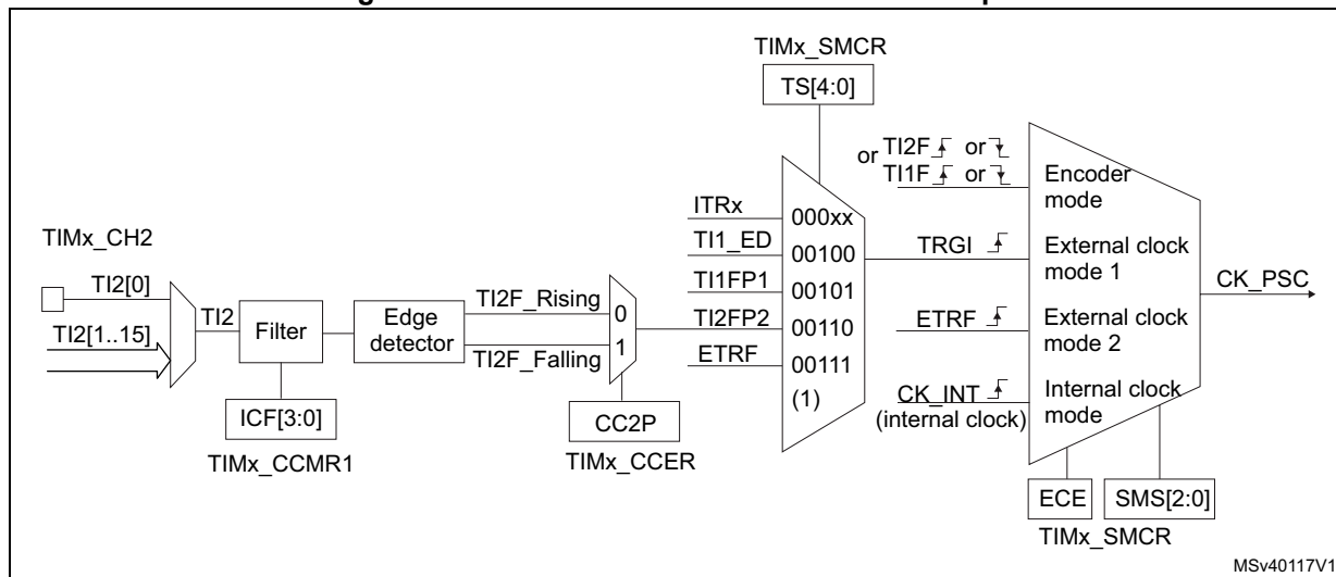
Figure 181. TI2 external clock connection example
