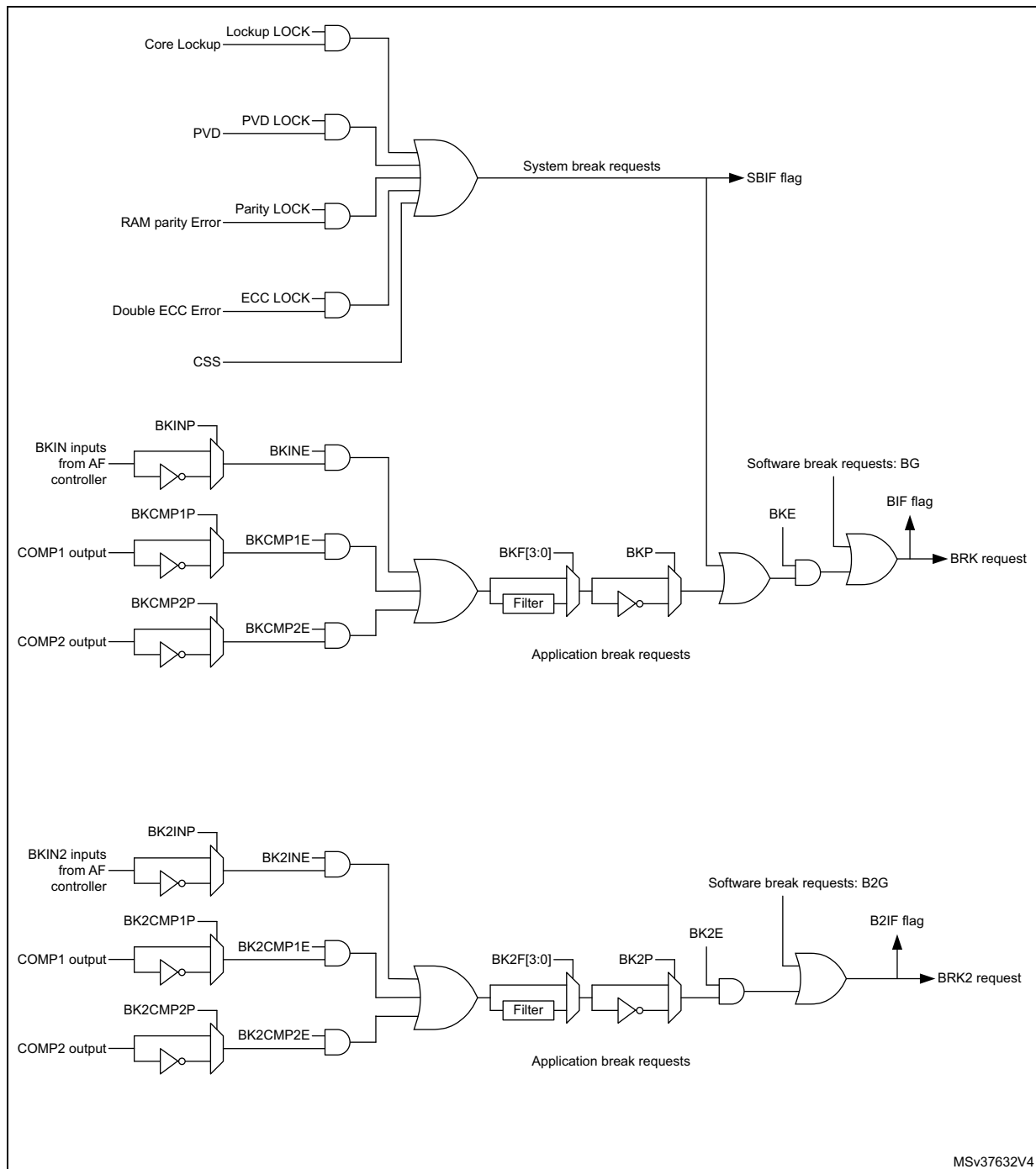
Figure 143. Break and Break2 circuitry overview
