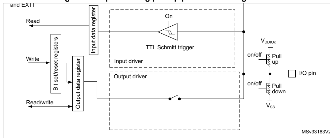
Figure 16. Input floating/pull up/pull down configurations
