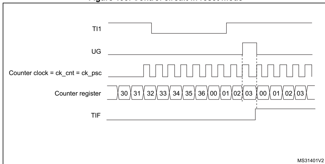
Figure 199. Control circuit in reset mode
