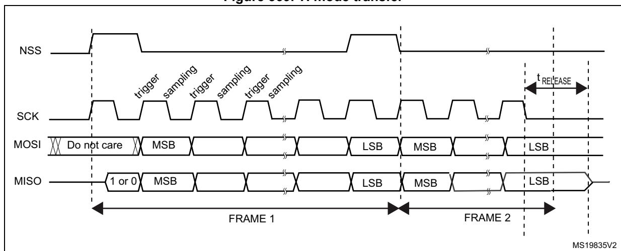
Figure 369. TI mode transfer
