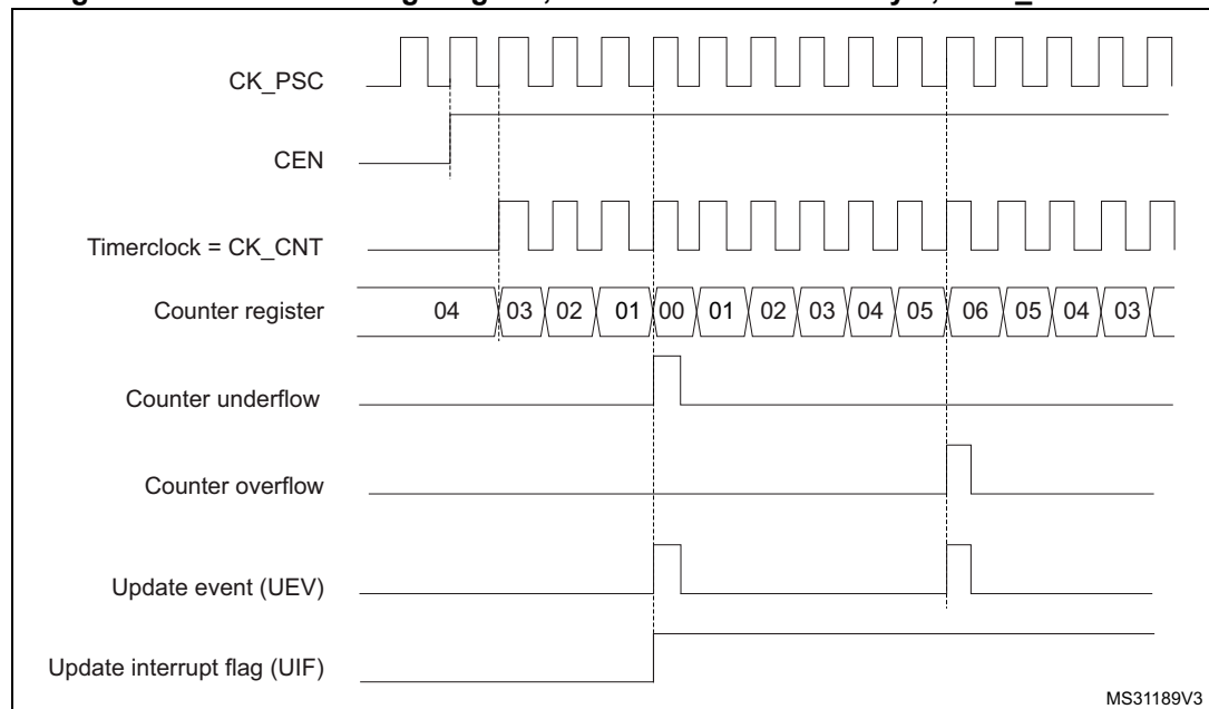
Figure 114. Counter timing diagram, internal clock divided by 1, TIMx_ARR = 0x6
