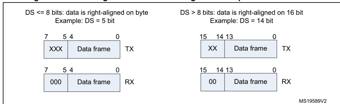
Figure 362. Data alignment when data length is not equal to 8-bit or 16-bit
