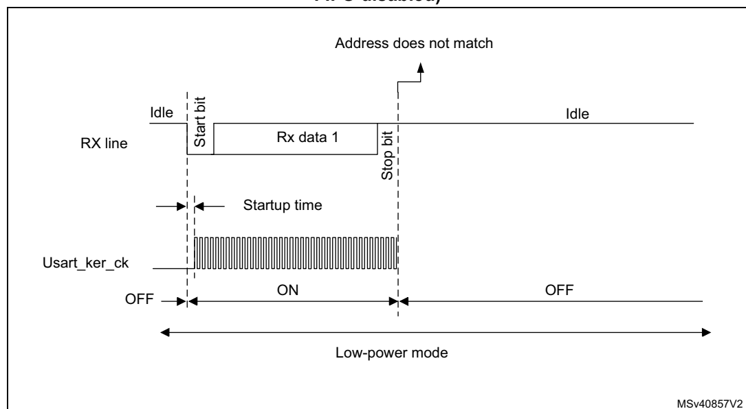
Figure 339. Wakeup event not verified (wakeup event = address match, FIFO disabled)
