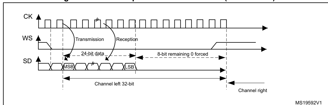
Figure 372. I 2 S Philips standard waveforms (24-bit frame)
