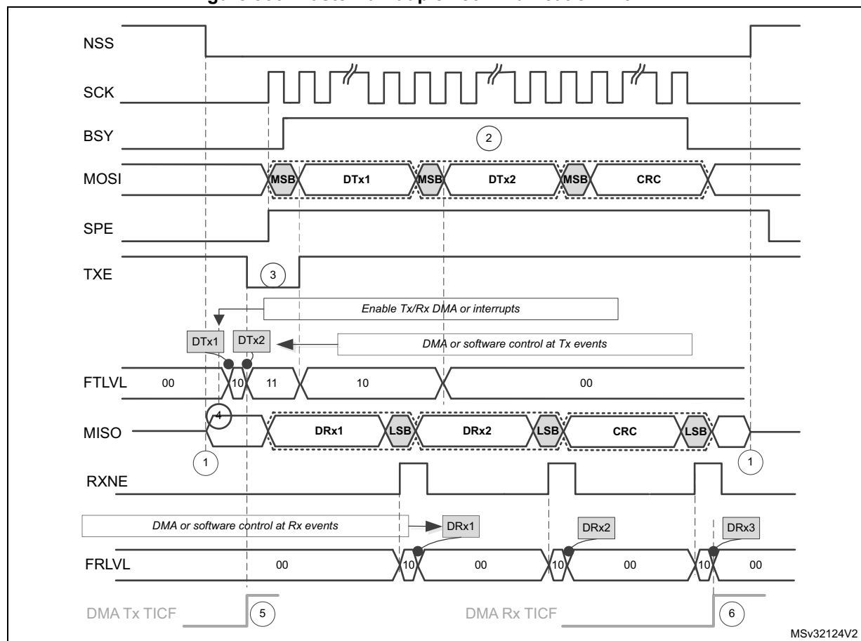
Figure 366. Master full-duplex communication with CRC
