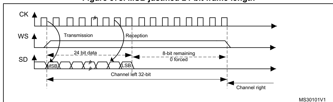
Figure 378. MSB justified 24-bit frame length
