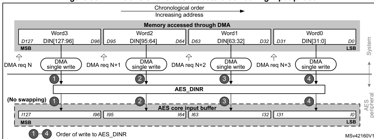
Figure 98. DMA transfer of a 128-bit data block during input phase
