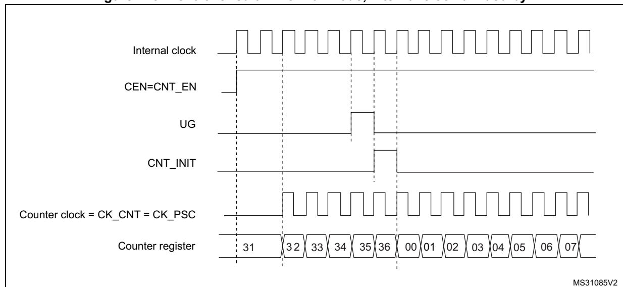
Figure 123. Control circuit in normal mode, internal clock divided by 1
