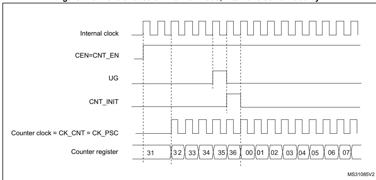
Figure 219. Control circuit in normal mode, internal clock divided by 1
