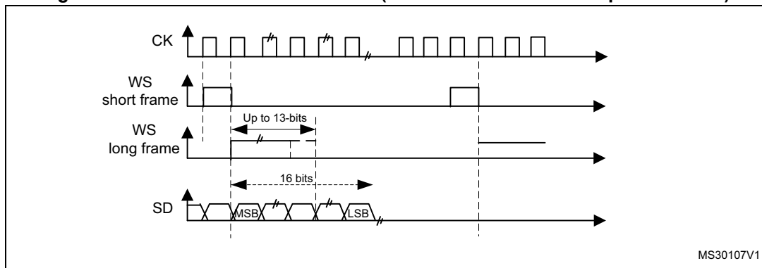
Figure 387. PCM standard waveforms (16-bit extended to 32-bit packet frame)
