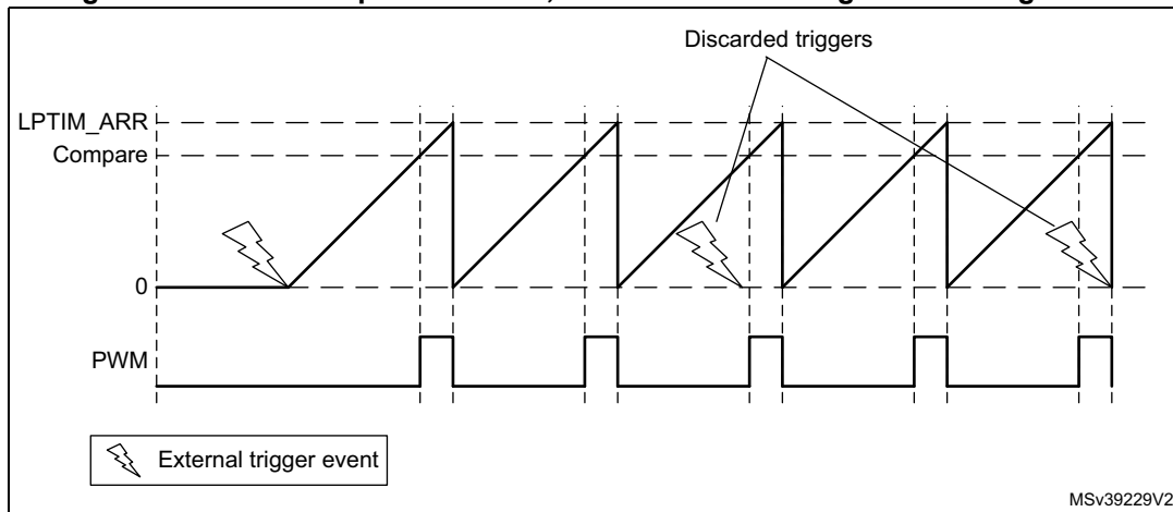
Figure 273. LPTIM output waveform, Continuous counting mode configuration
