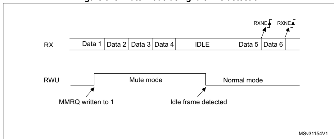
Figure 345. Mute mode using Idle line detection
