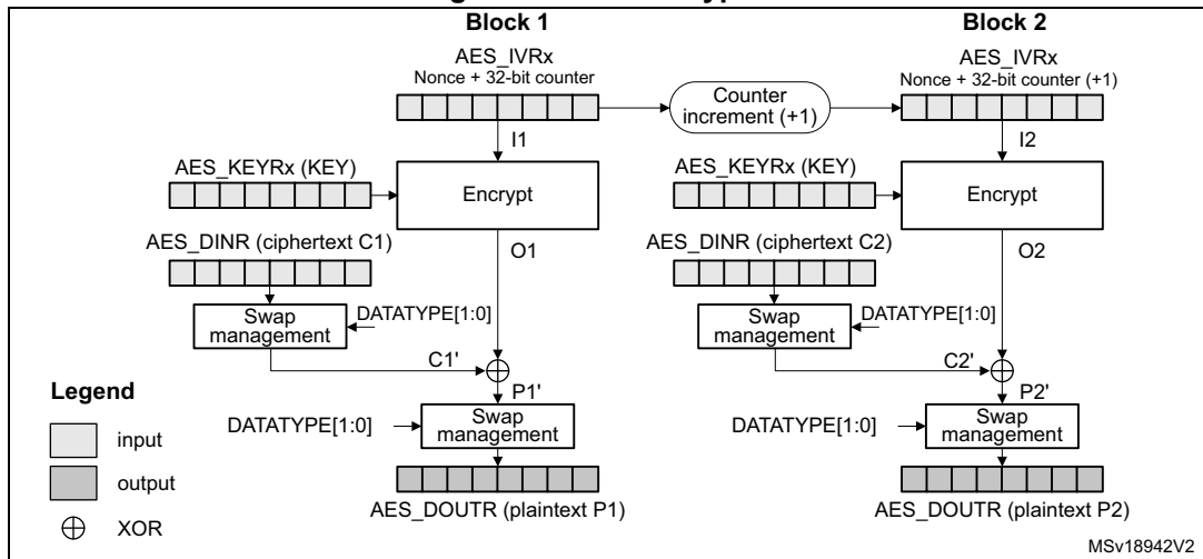
Figure 90. CTR decryption
