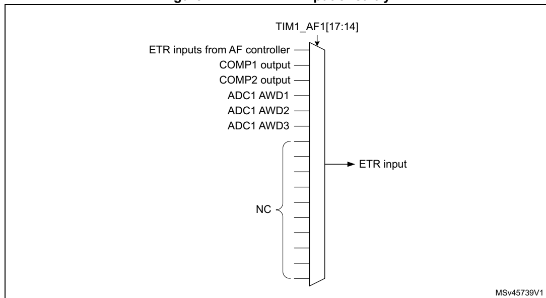
Figure 122. TIM1 ETR input circuitry
