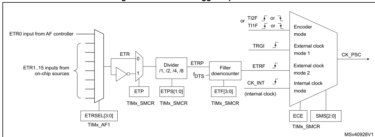
Figure 183. External trigger input block
