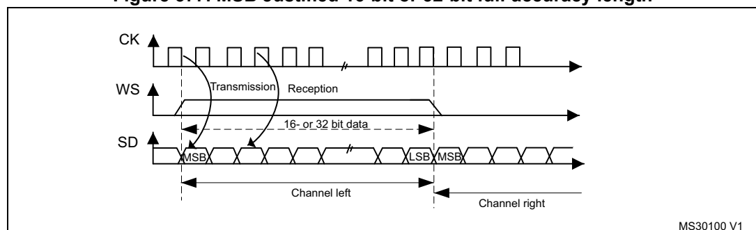
Figure 377. MSB Justified 16-bit or 32-bit full-accuracy length
