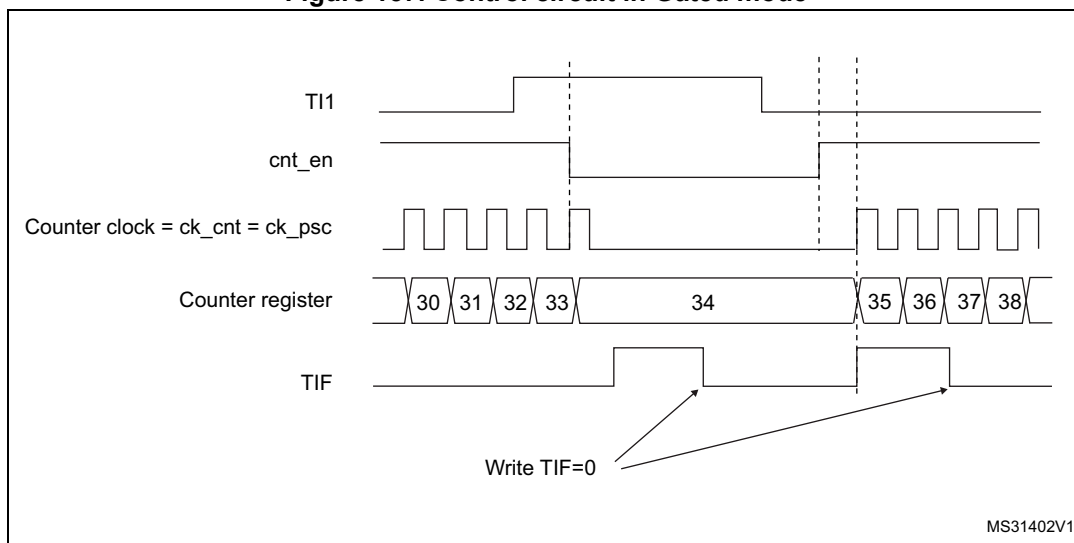
Figure 157. Control circuit in Gated mode
