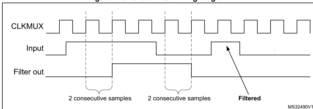
Figure 270. Glitch filter timing diagram
