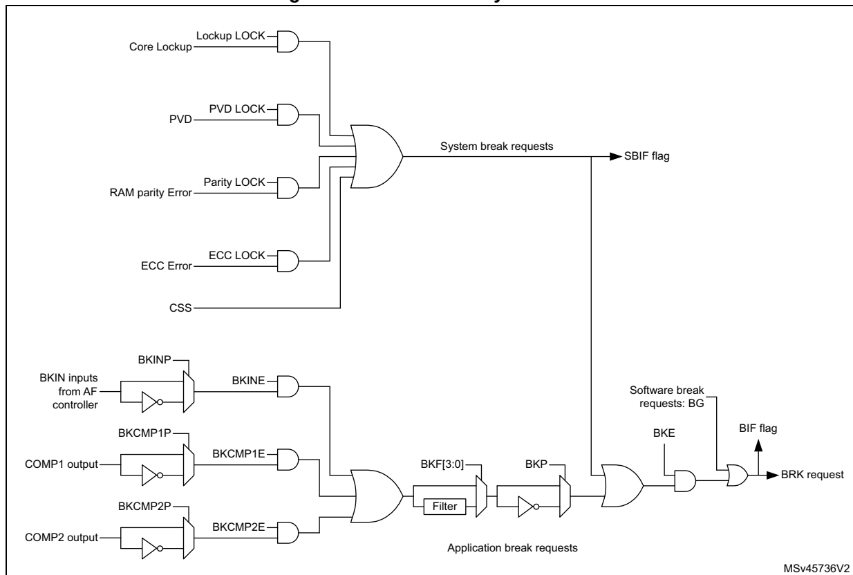
Figure 260. Break circuitry overview
