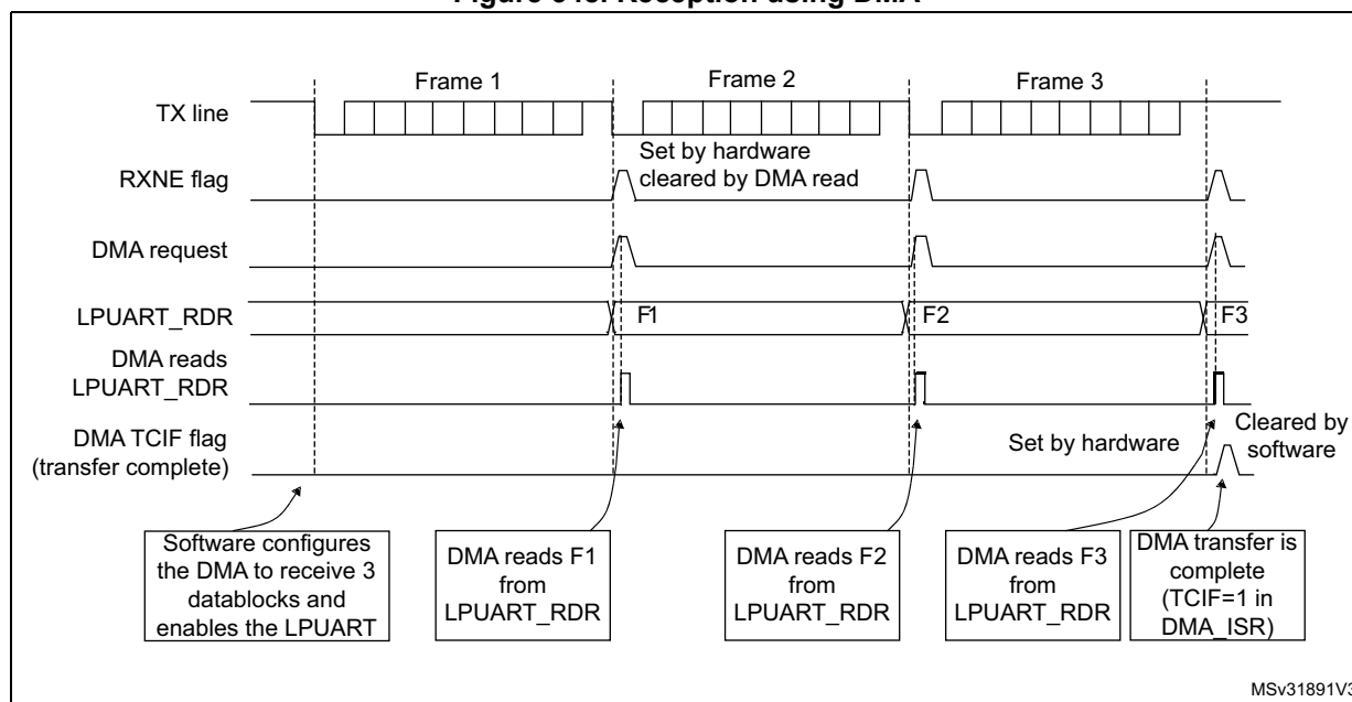
Figure 348. Reception using DMA
