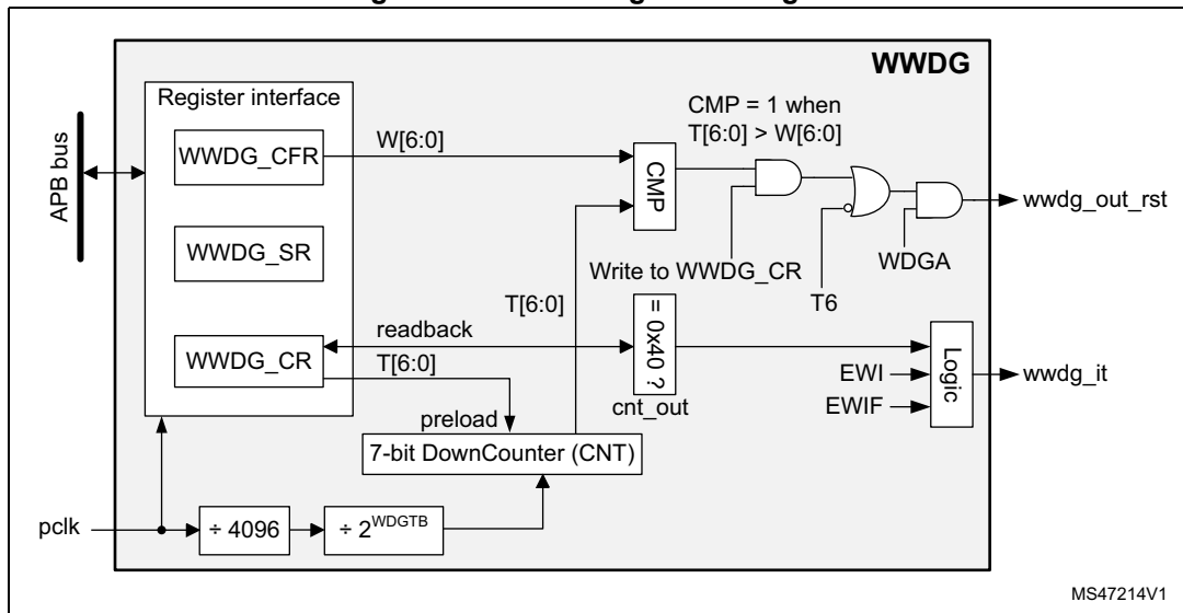
Figure 278. Watchdog block diagram
