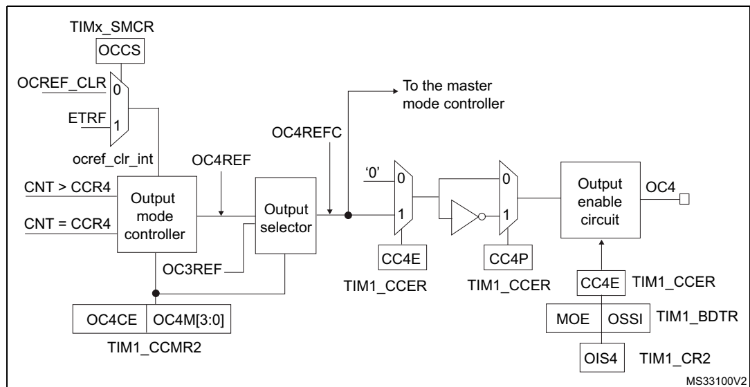
Figure 131. Output stage of capture/compare channel (channel 4)
