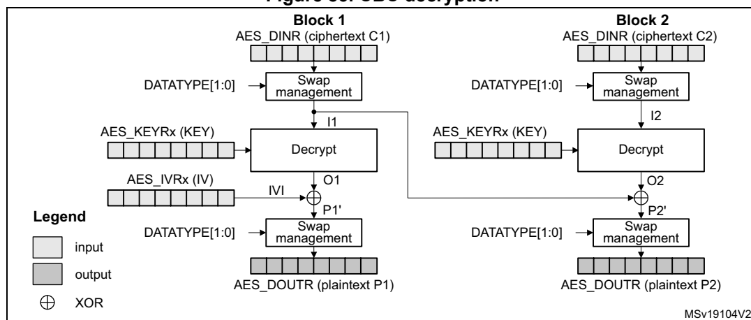
Figure 85. CBC decryption
