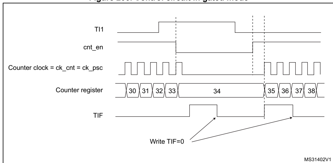
Figure 200. Control circuit in gated mode
