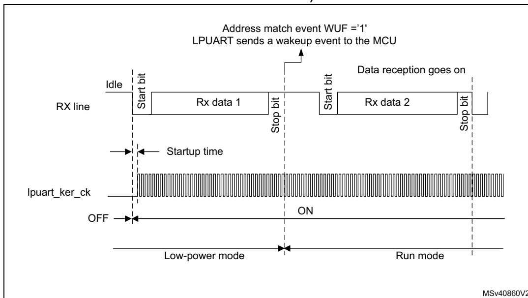
Figure 352. Wakeup event verified (wakeup event = address match, FIFO disabled)
