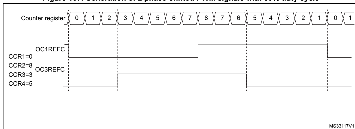
Figure 137. Generation of 2 phase-shifted PWM signals with 50% duty cycle
