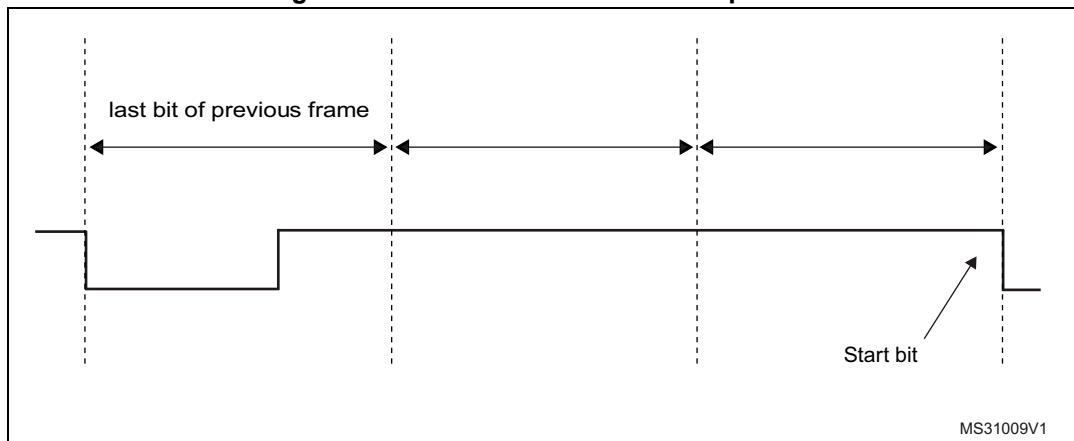
Figure 408. SFT of three nominal bit periods
