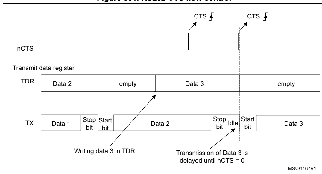
Figure 351. RS232 CTS flow control
