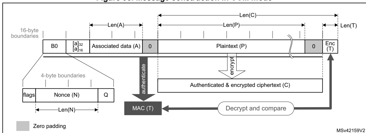
Figure 95. Message construction in CCM mode
