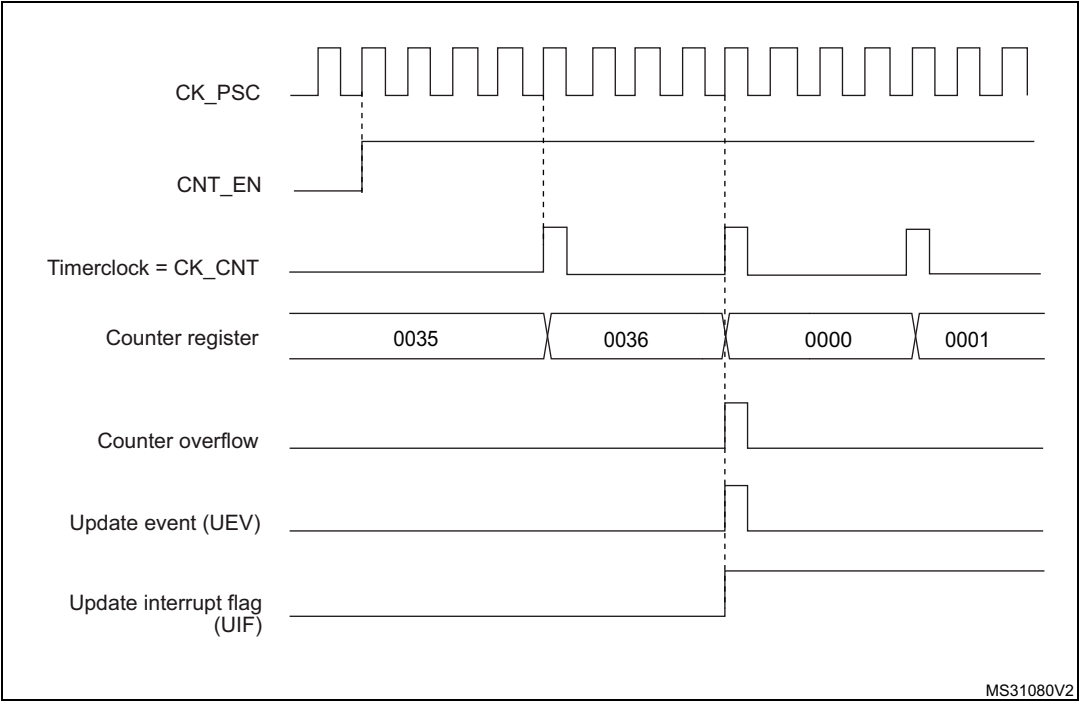
Figure 225. Counter timing diagram, internal clock divided by 4
