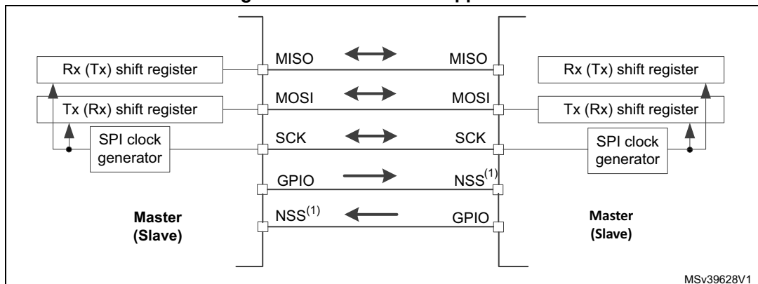
Figure 359. Multi-master application
