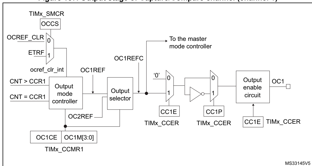
Figure 187. Output stage of Capture/Compare channel (channel 1)
