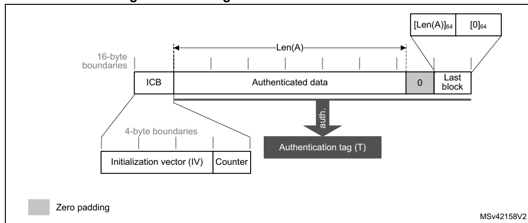
Figure 93. Message construction in GMAC mode
