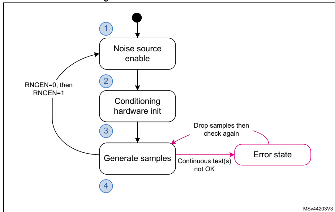
Figure 72. RNG initialization overview
