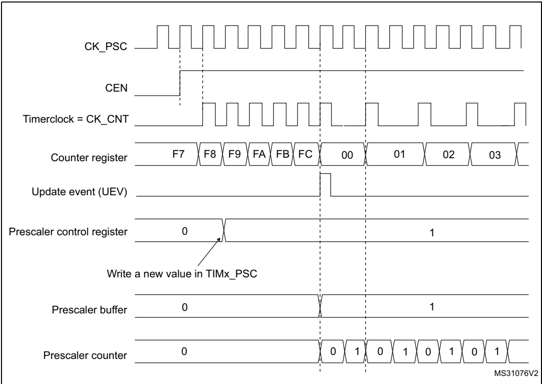
Figure 211. Counter timing diagram with prescaler division change from 1 to 2
