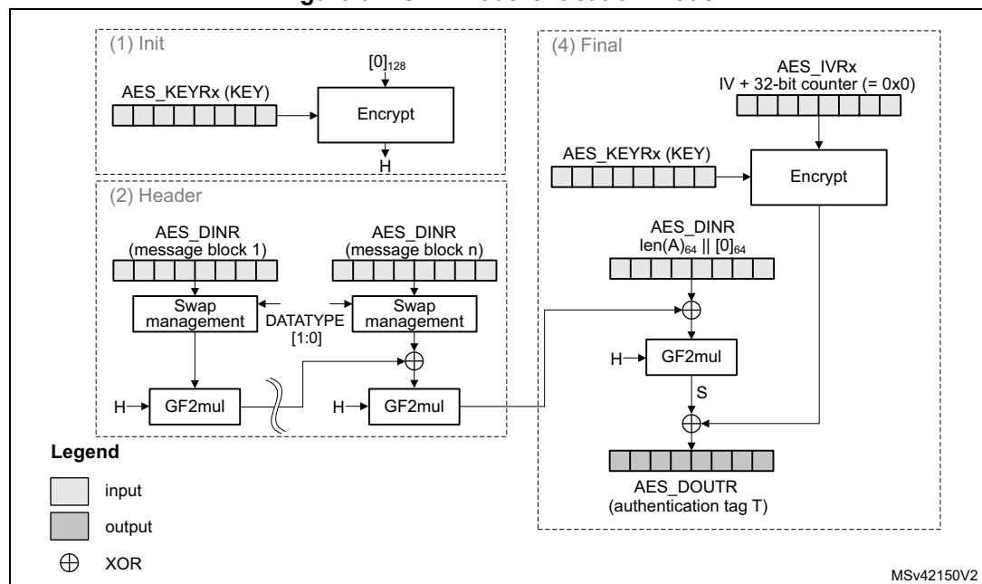
Figure 94. GMAC authentication mode
