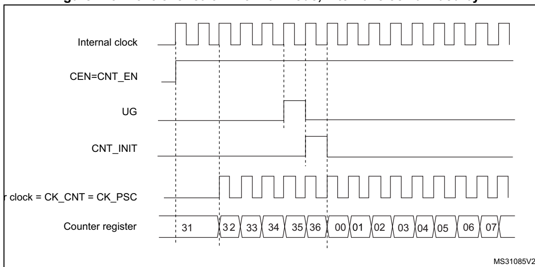
Figure 229. Control circuit in normal mode, internal clock divided by 1
