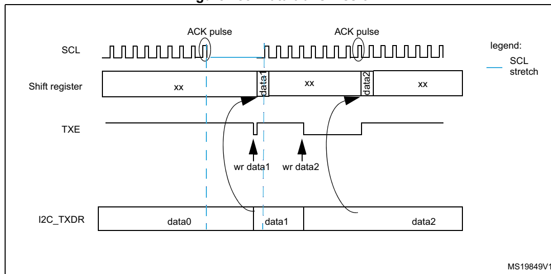
Figure 288. Data transmission
