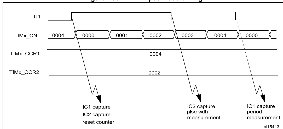
Figure 253. PWM input mode timing
