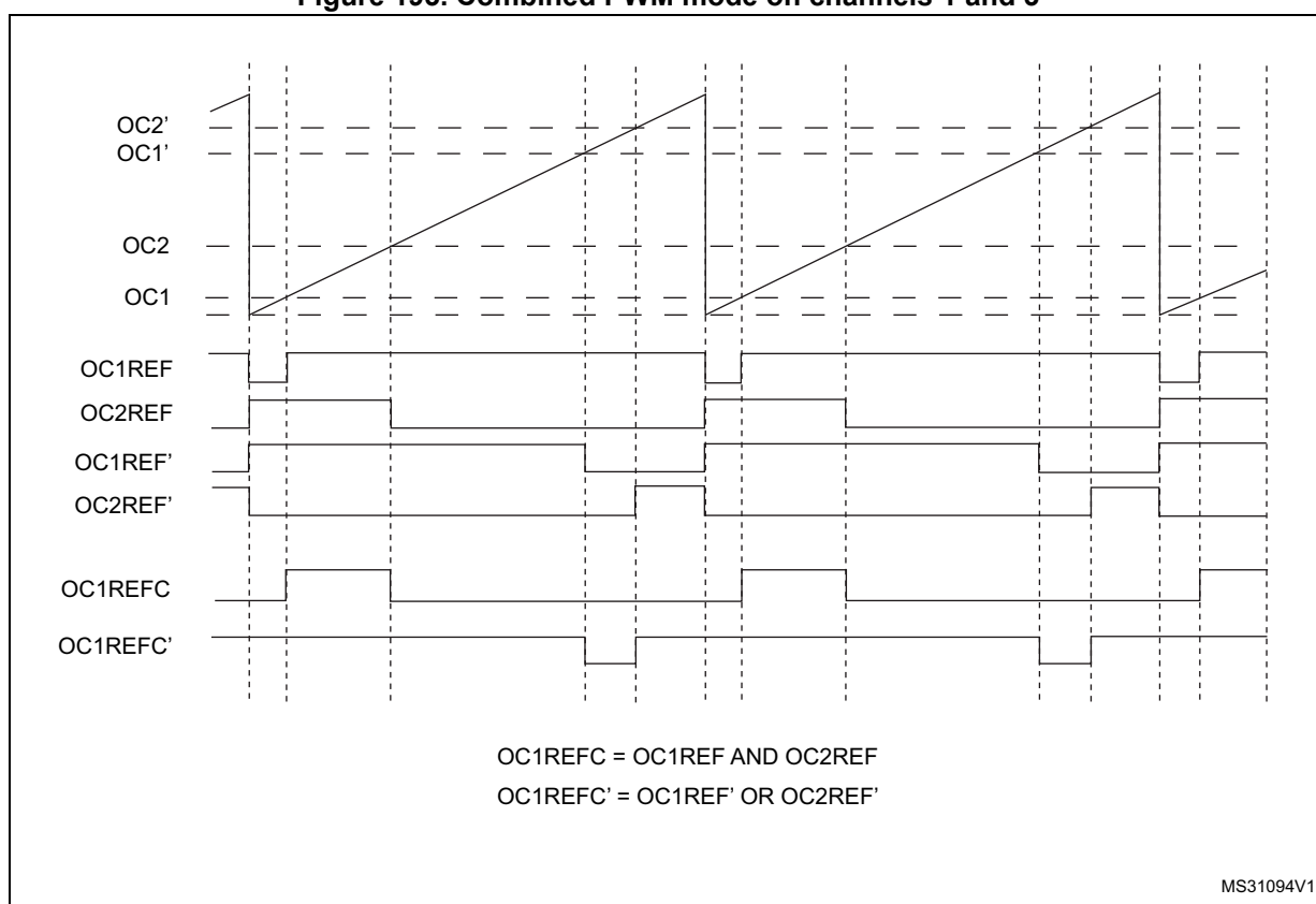
Figure 193. Combined PWM mode on channels 1 and 3
