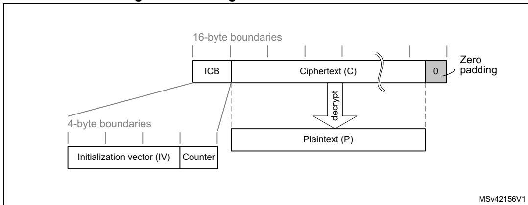
Figure 88. Message construction in CTR mode
