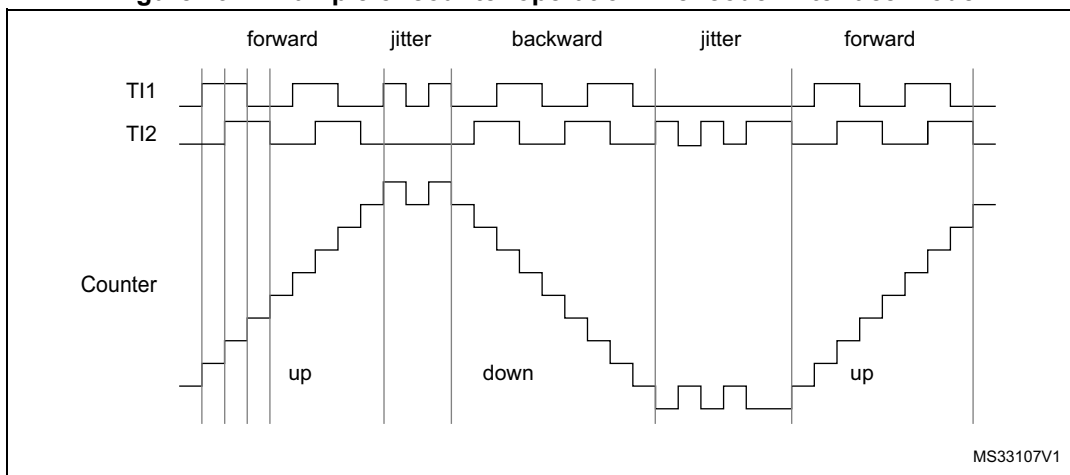
Figure 197. Example of counter operation in encoder interface mode
