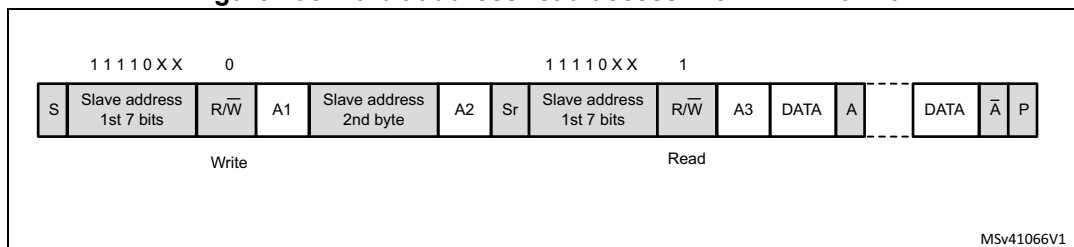
Figure 298. 10-bit address read access with HEAD10R=0
