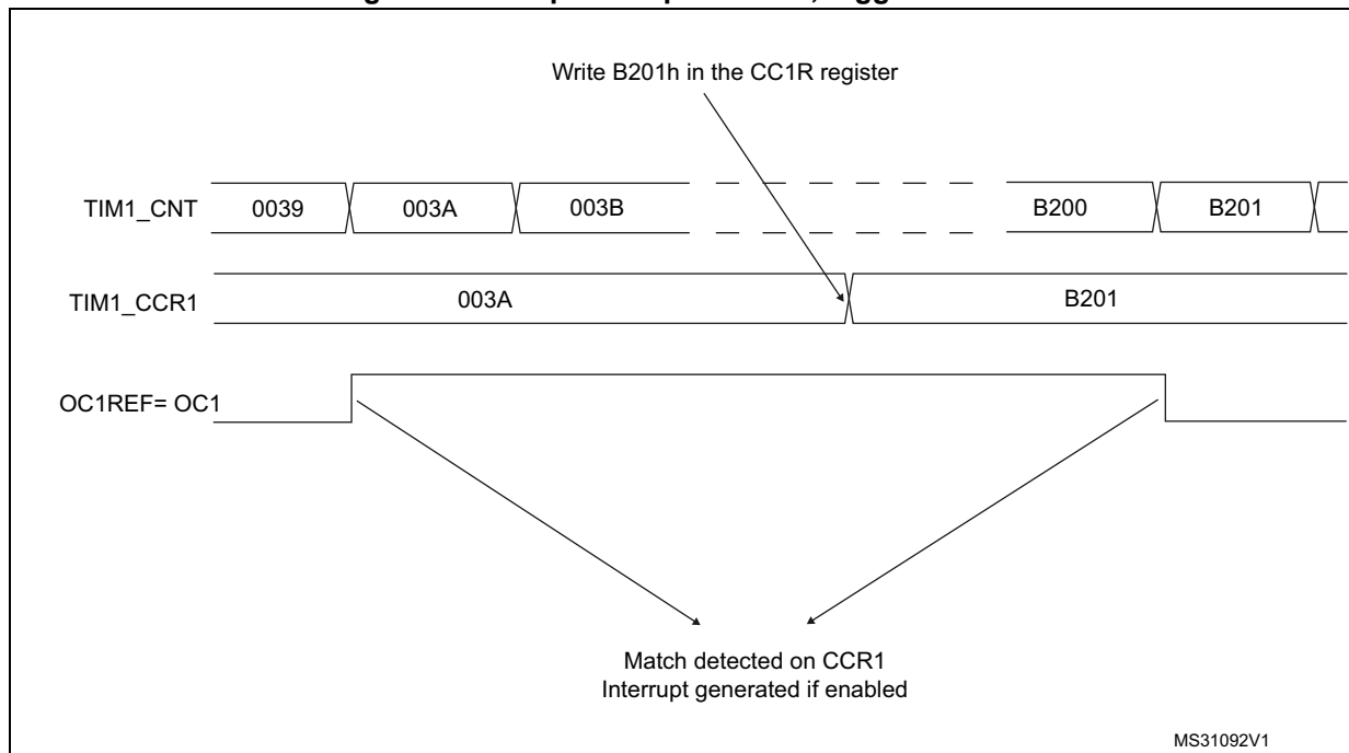
Figure 189. Output compare mode, toggle on OC1
