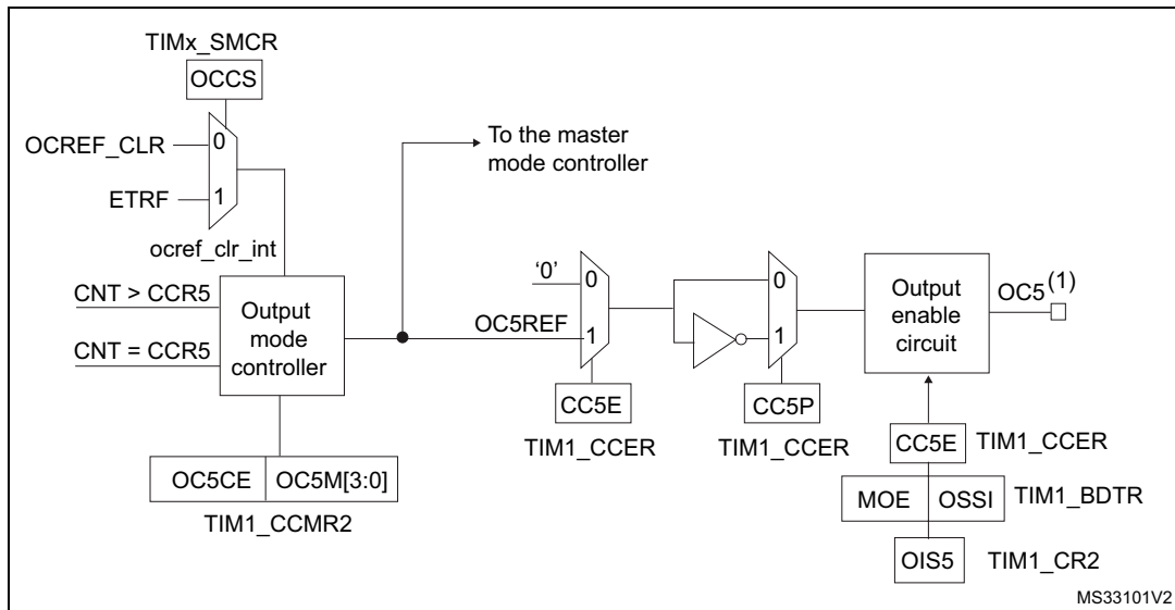
Figure 132. Output stage of capture/compare channel (channel 5, idem ch. 6)
