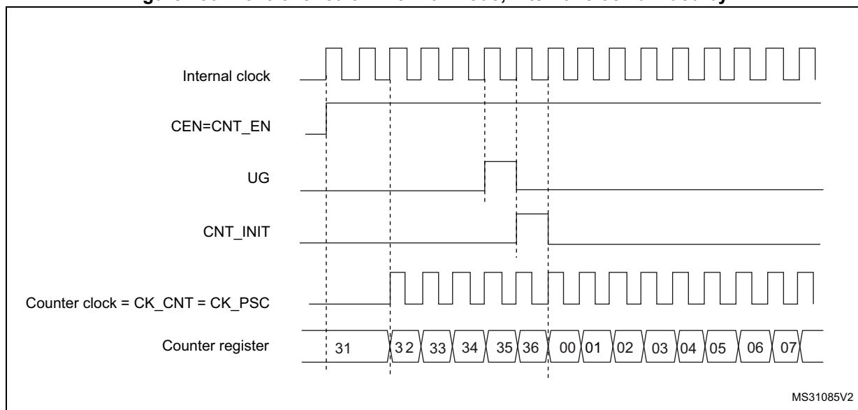
Figure 180. Control circuit in normal mode, internal clock divided by 1
