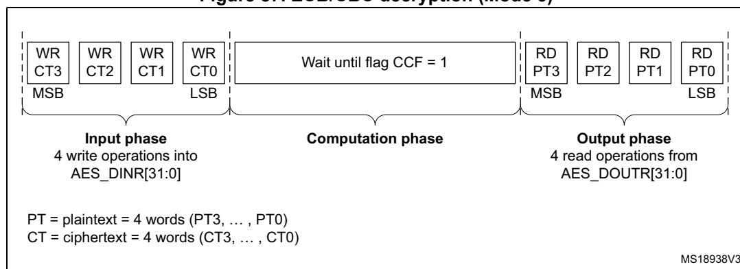
Figure 87. ECB/CBC decryption (Mode 3)
