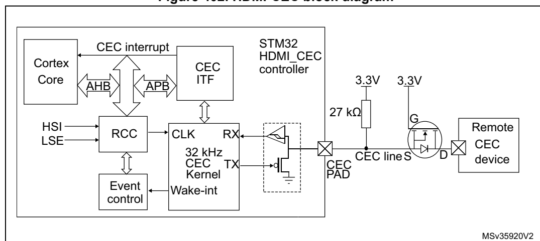
Figure 402. HDMI-CEC block diagram
