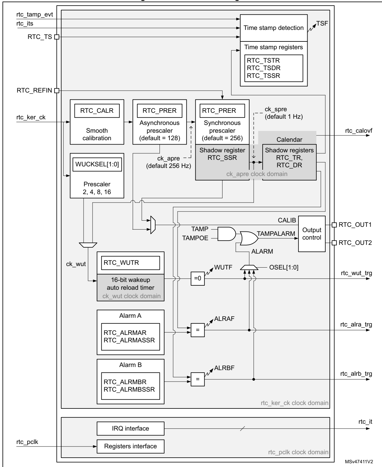
Figure 280. RTC block diagram
