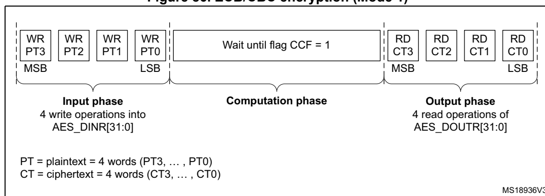
Figure 86. ECB/CBC encryption (Mode 1)
