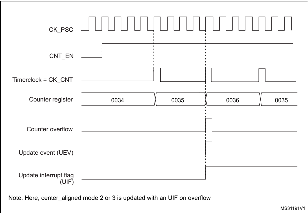
Figure 176. Counter timing diagram, internal clock divided by 4, TIMx_ARR=0x36
