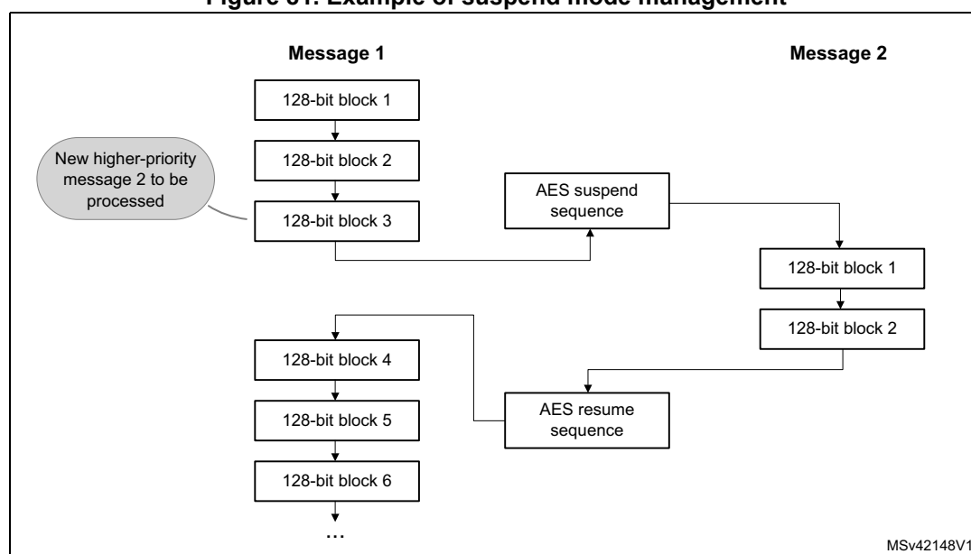
Figure 81. Example of suspend mode management
