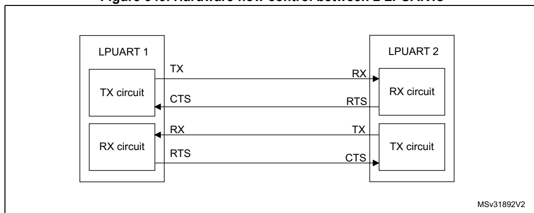
Figure 349. Hardware flow control between 2 LPUARTs
