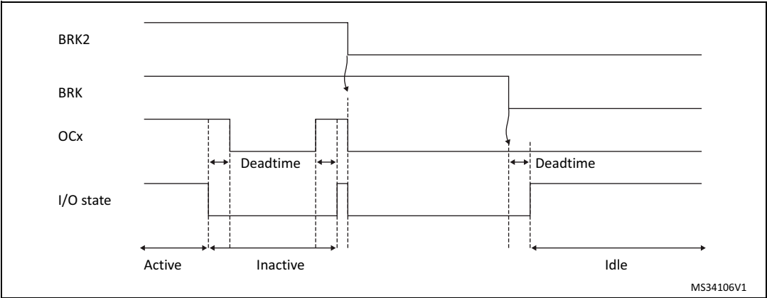
Figure 145. PWM output state following BRK and BRK2 pins assertion ( OSSl=1 )
