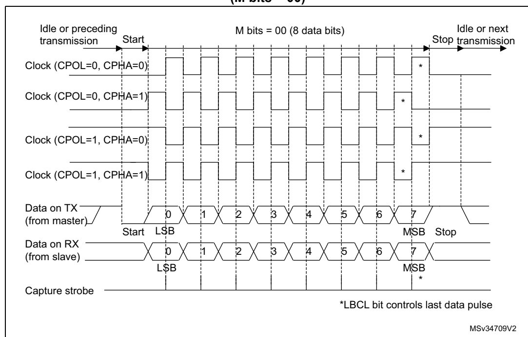
Figure 326. USART data clock timing diagram in synchronous master mode (M bits = 00)
