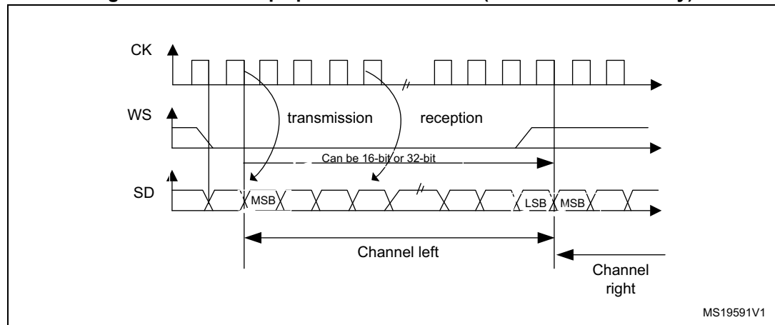
Figure 371. I 2 S Philips protocol waveforms (16/32-bit full accuracy)
