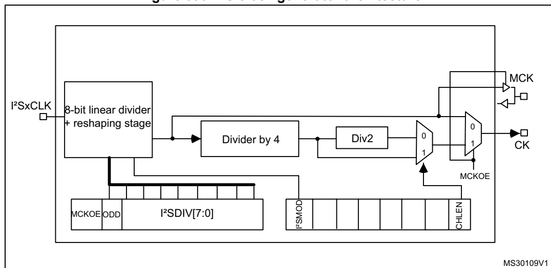
Figure 390. I 2 S clock generator architecture
