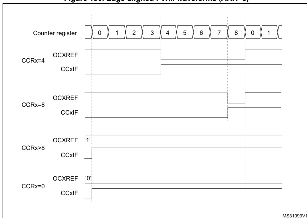
Figure 190. Edge-aligned PWM waveforms (ARR=8)
