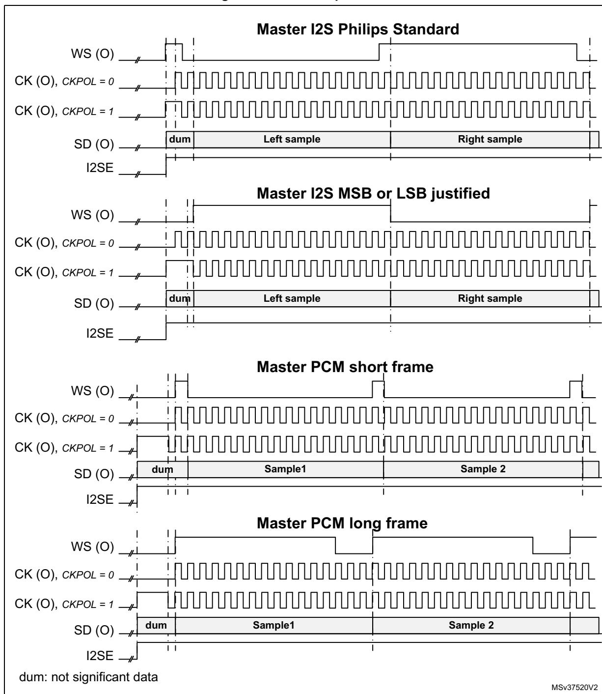
Figure 388. Start sequence in master mode
