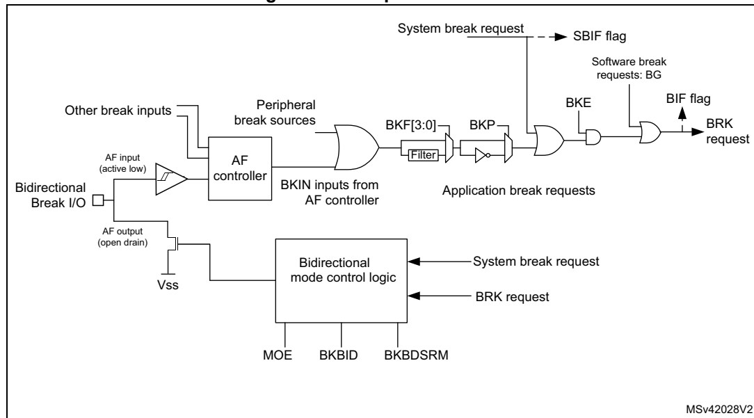
Figure 262. Output redirection
