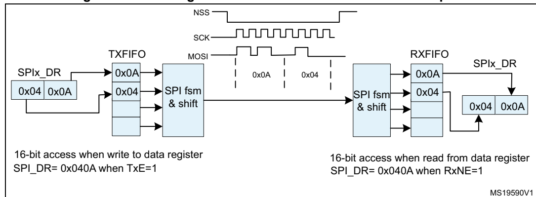
Figure 363. Packing data in FIFO for transmission and reception
