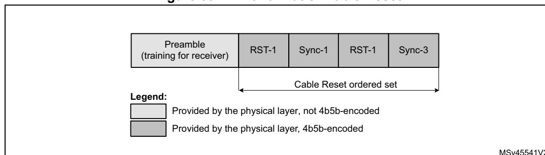
Figure 397. Line format of Cable Reset
