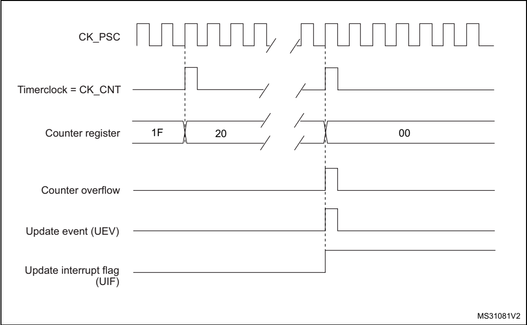
Figure 226. Counter timing diagram, internal clock divided by N
