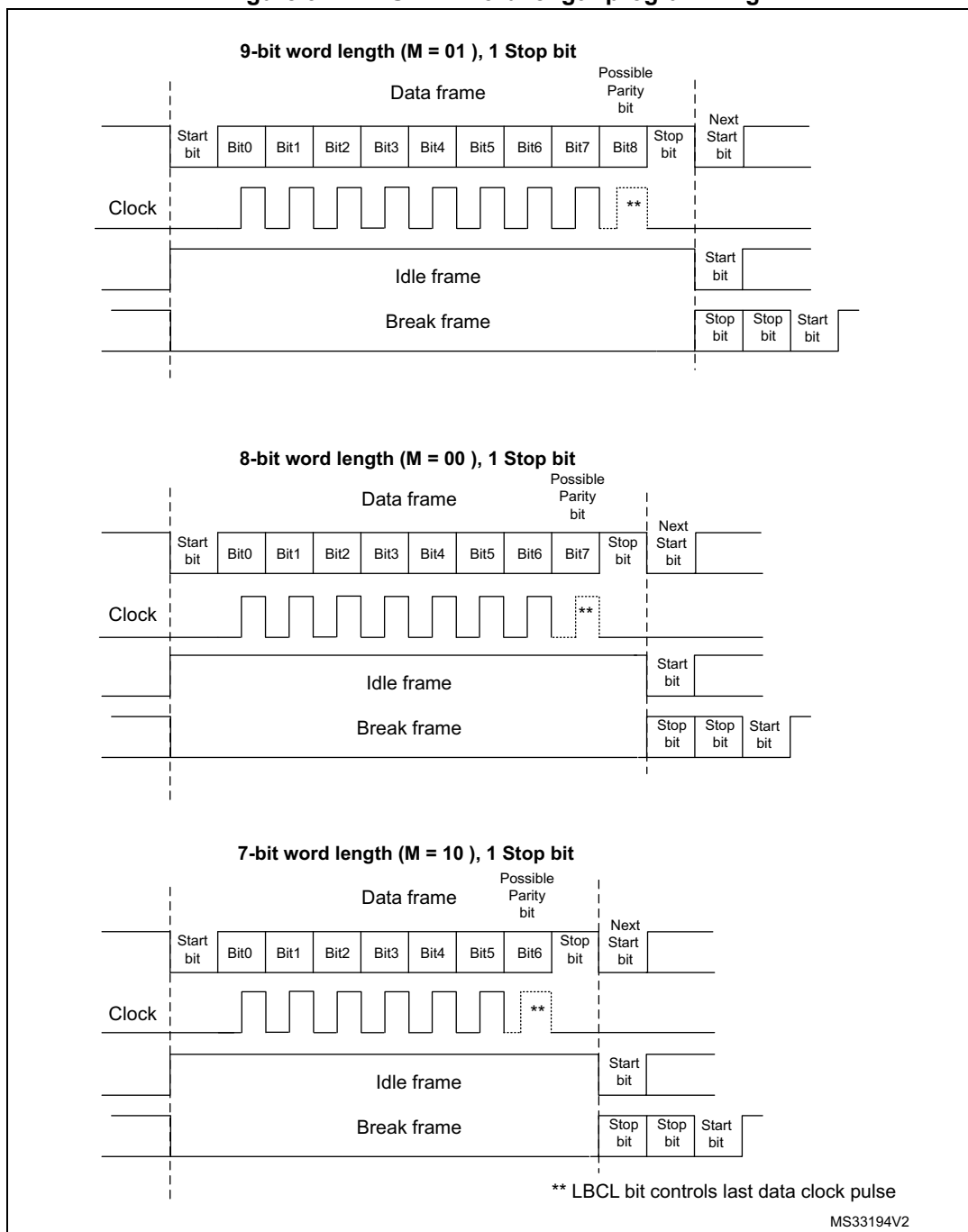
Figure 341. LPUART word length programming
