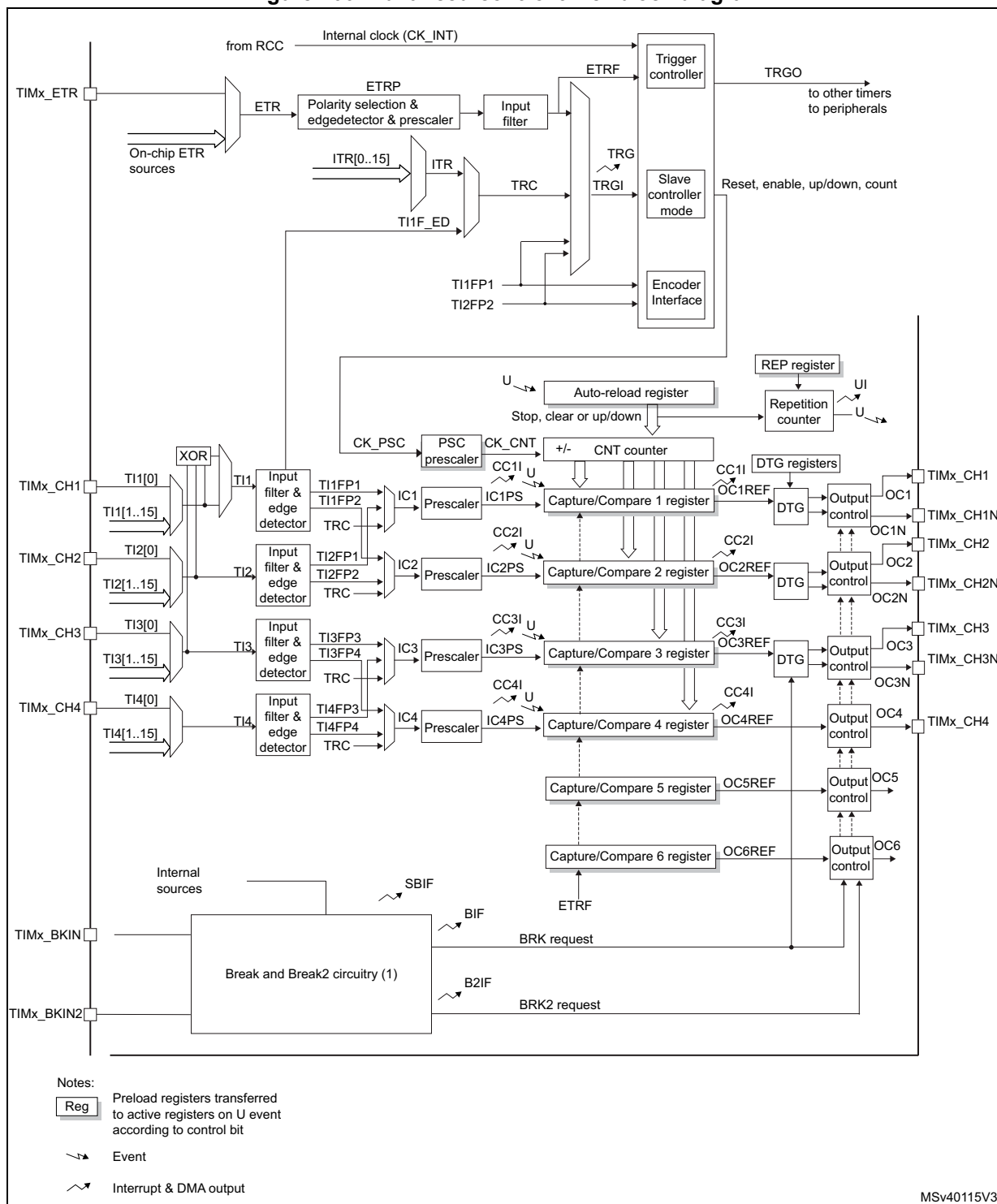
Figure 100. Advanced-control timer block diagram
