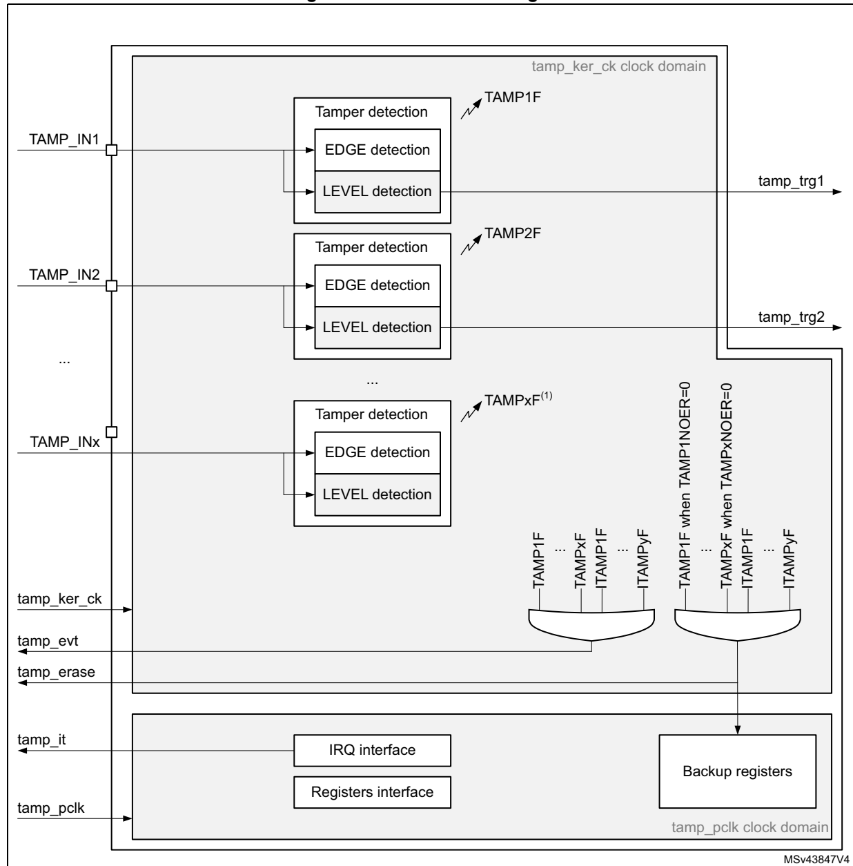
Figure 281. TAMP block diagram
