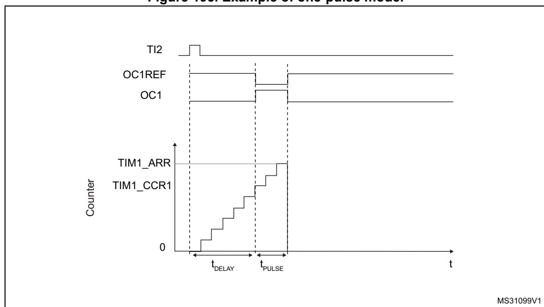
Figure 195. Example of one-pulse mode.
