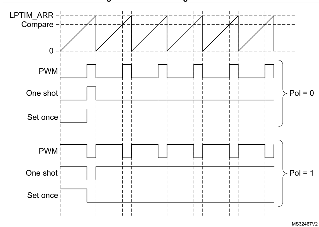
Figure 274. Waveform generation
