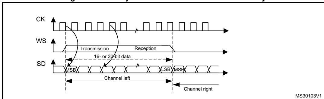
Figure 380. LSB justified 16-bit or 32-bit full-accuracy
