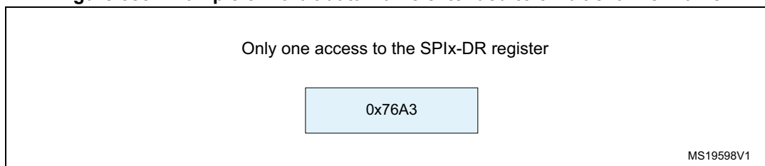
Figure 385. Example of 16-bit data frame extended to 32-bit channel frame
