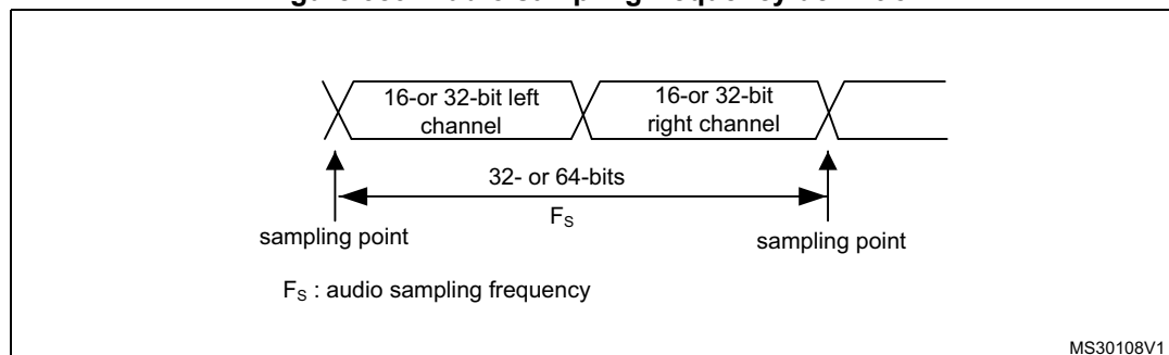
Figure 389. Audio sampling frequency definition
