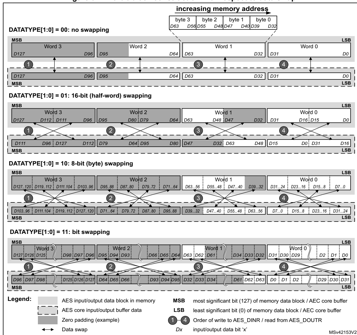
Figure 97. 128-bit block construction with respect to data swap
