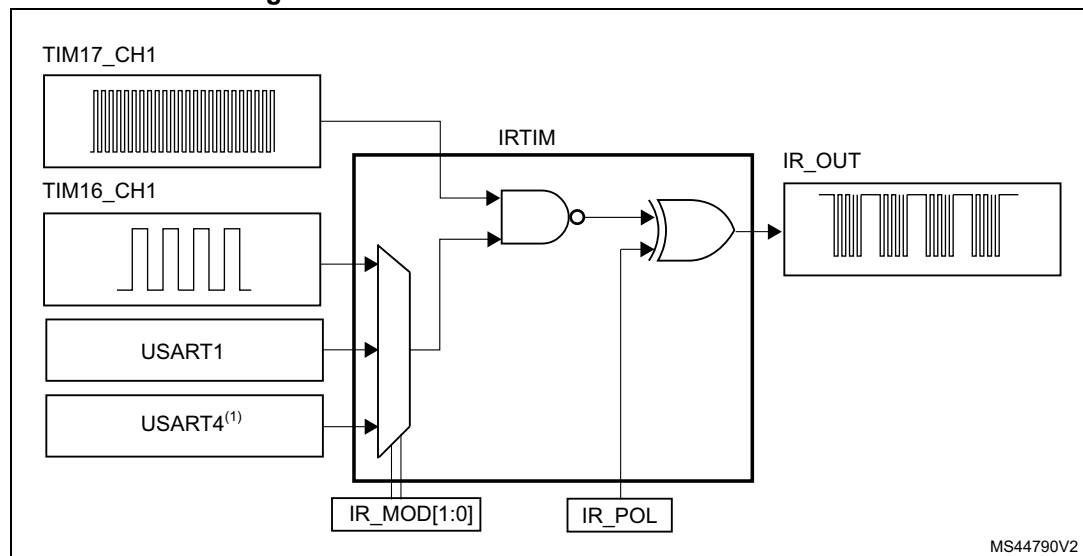
Figure 276. IRTIM internal hardware connections
