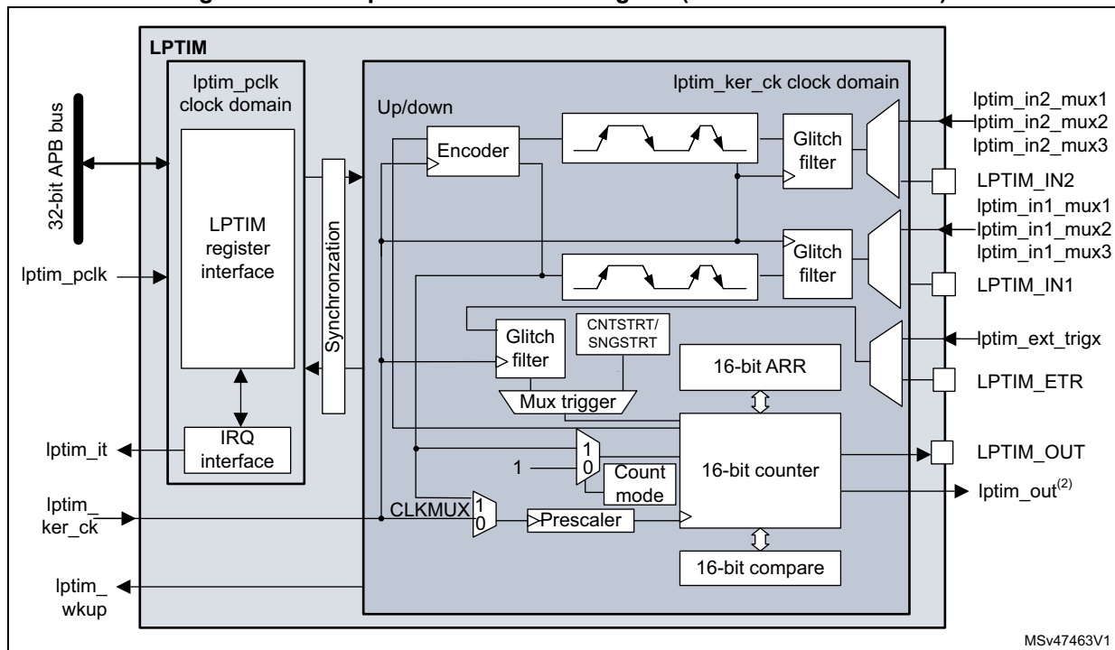
Figure 269. Low-power timer block diagram (LPTIM1 and LPTIM2 (1) )
