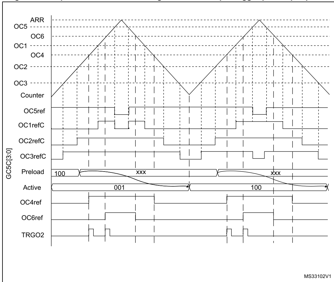
Figure 139. 3-phase combined PWM signals with multiple trigger pulses per period
