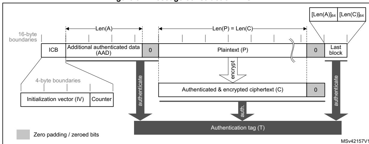
Figure 91. Message construction in GCM
