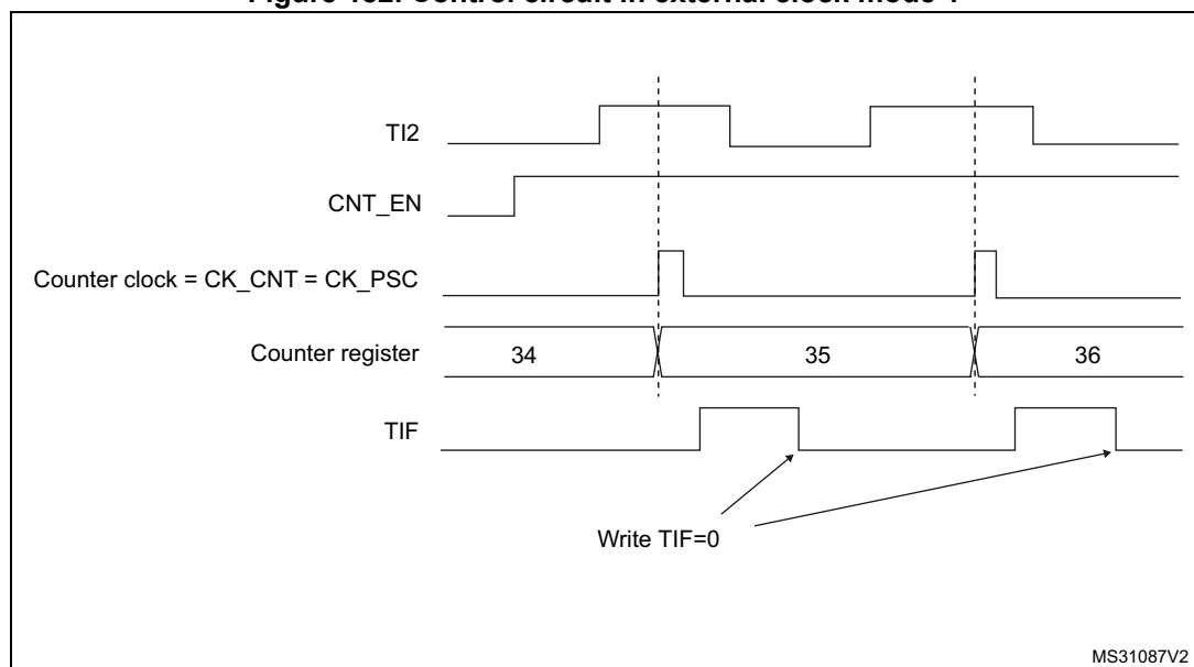
Figure 182. Control circuit in external clock mode 1
