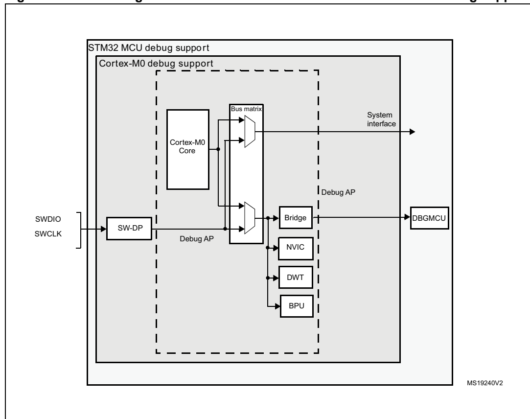
Figure 412. Block diagram of STM32G0x1 MCU and Cortex®-M0+-level debug support
