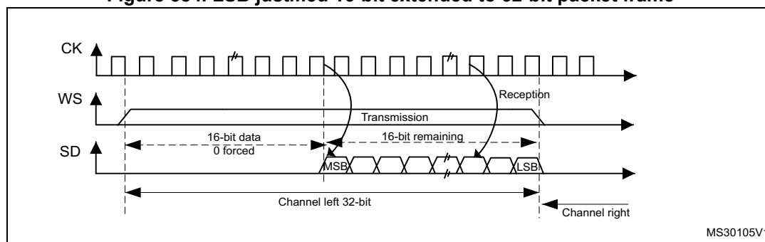
Figure 384. LSB justified 16-bit extended to 32-bit packet frame
