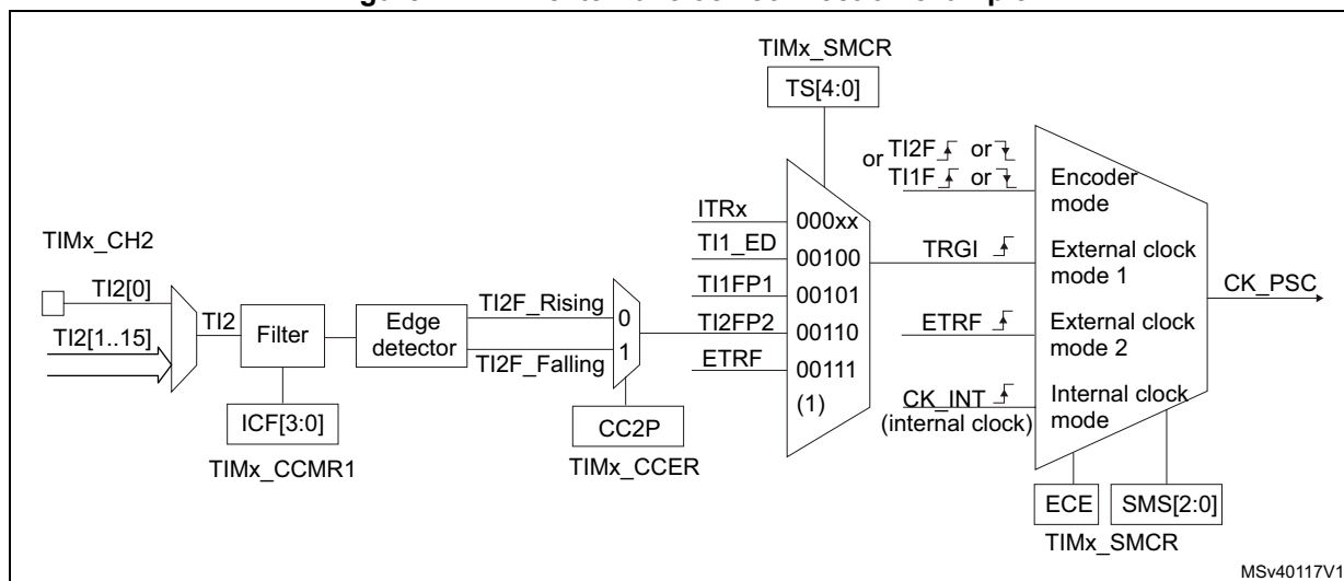
Figure 124. TI2 external clock connection example
