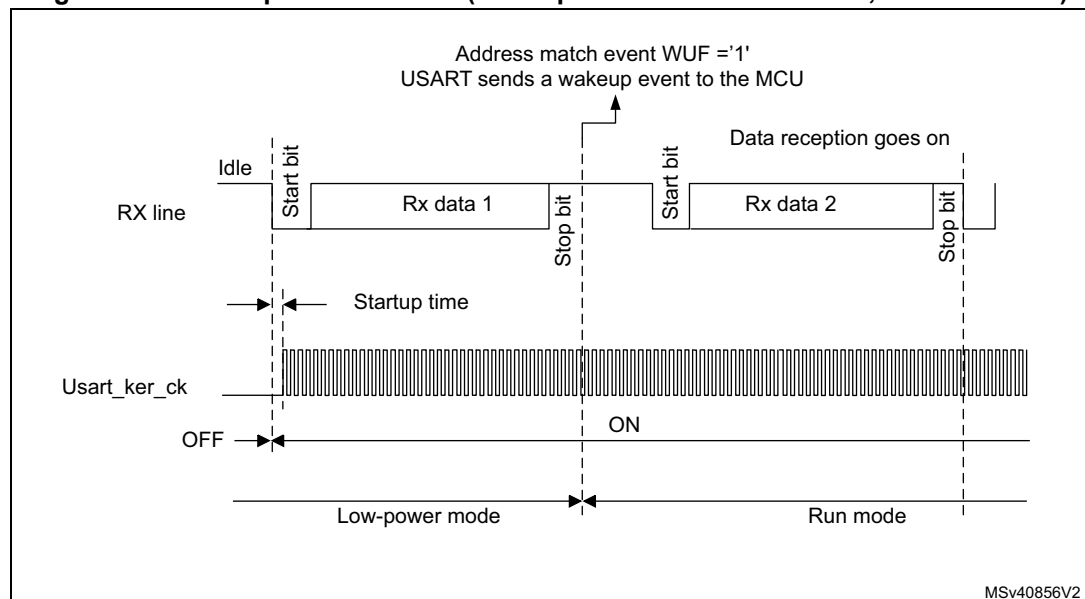
Figure 338. Wakeup event verified (wakeup event = address match, FIFO disabled)
