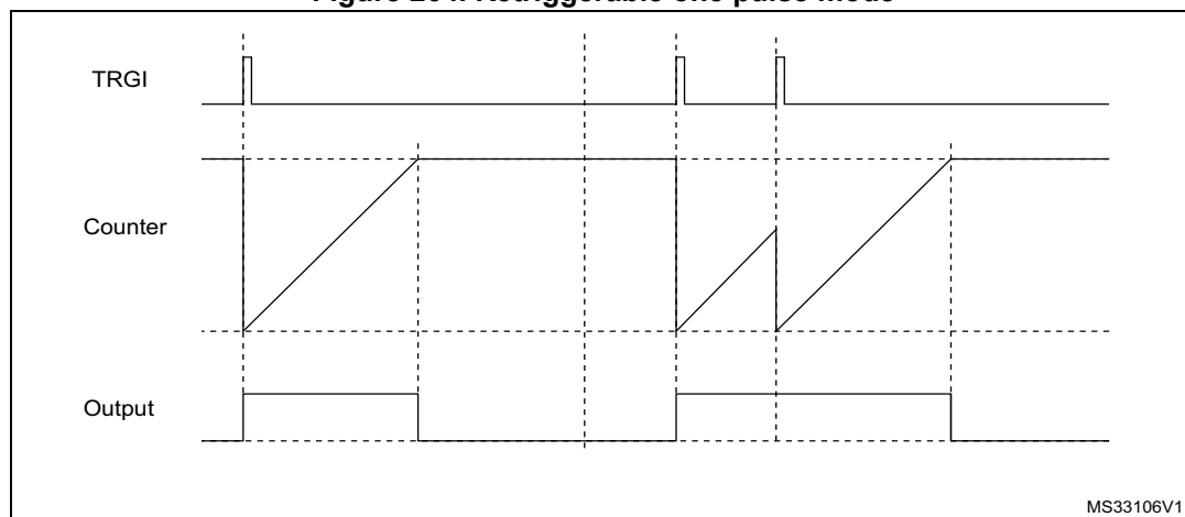
Figure 264. Retriggerable one pulse mode
