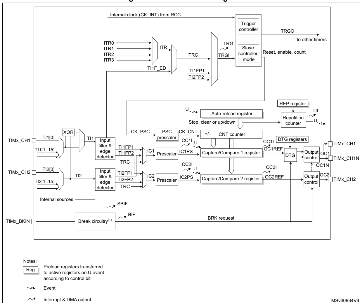
Figure 235. TIM15 block diagram
