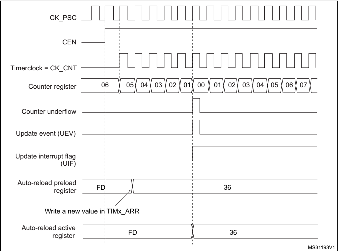
Figure 178. Counter timing diagram, Update event with ARPE=1 (counter underflow)
