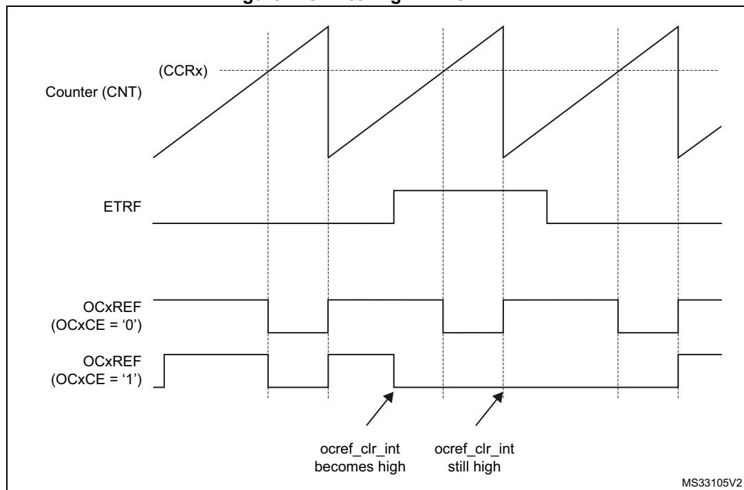
Figure 148. Clearing TIMx OCxREF
