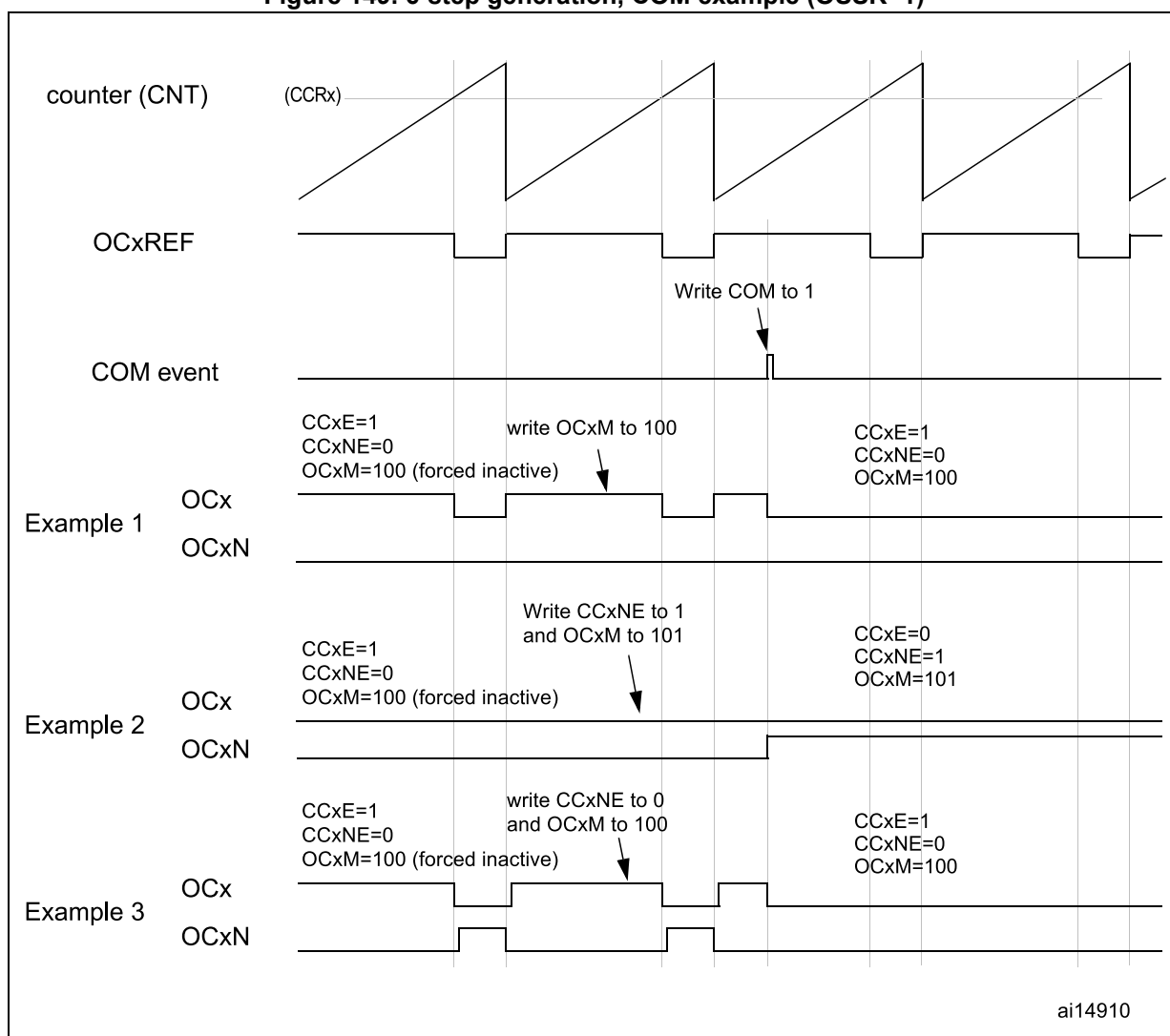
Figure 149. 6-step generation, COM example (OSSR=1)
