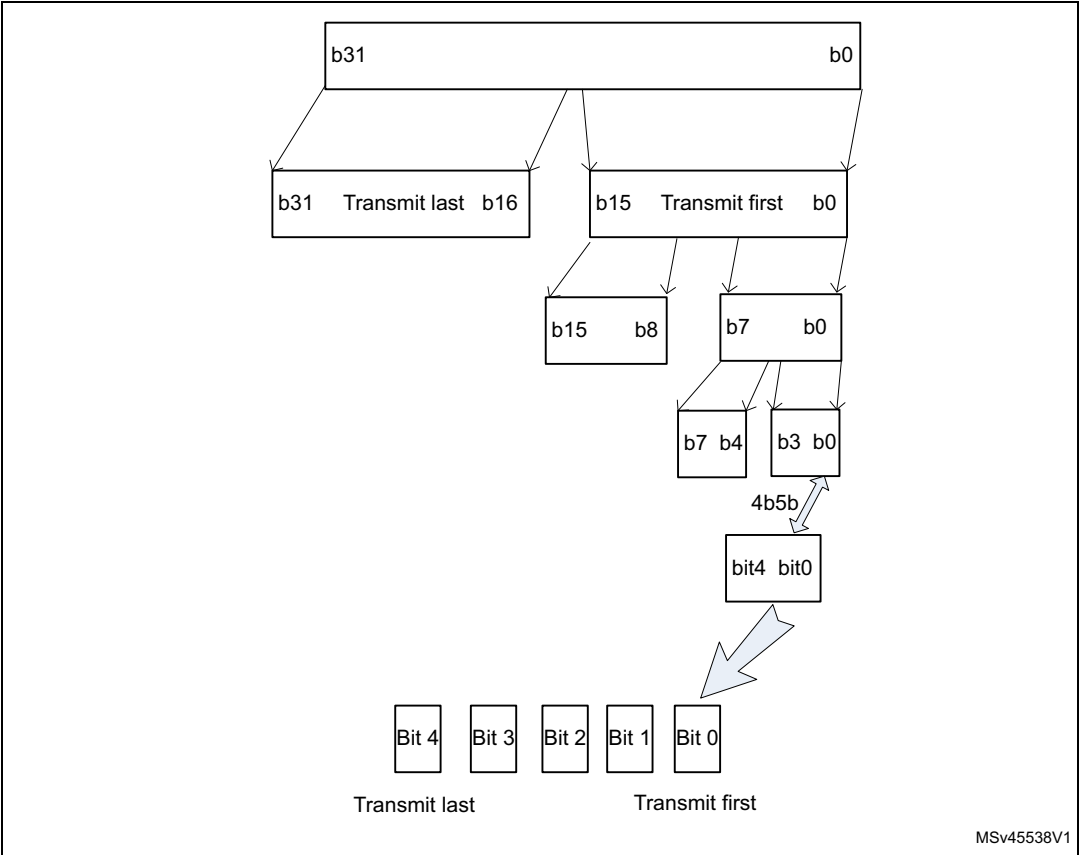
Figure 394. Transmit order for various sizes of data
