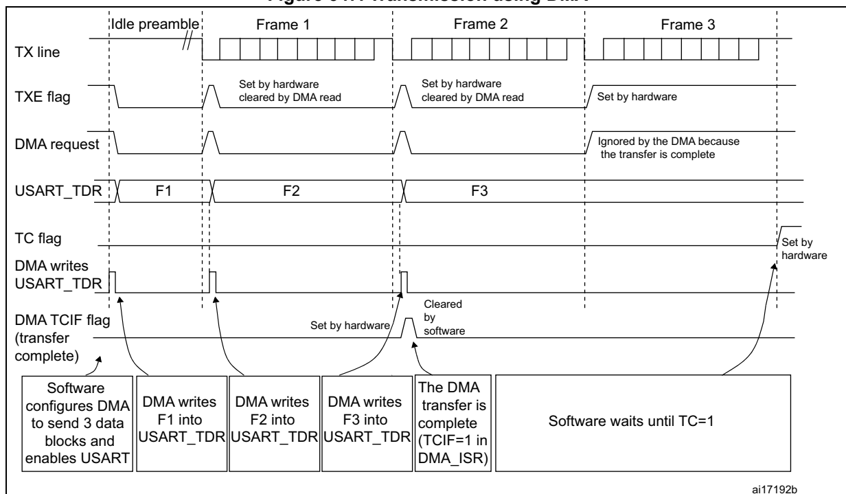
Figure 347. Transmission using DMA
