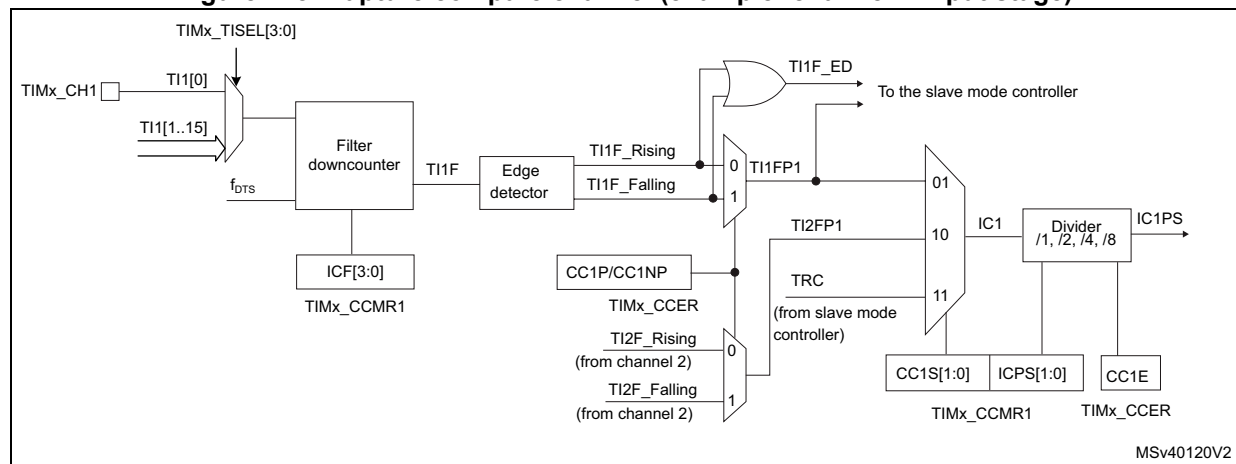
Figure 128. Capture/compare channel (example: channel 1 input stage)
