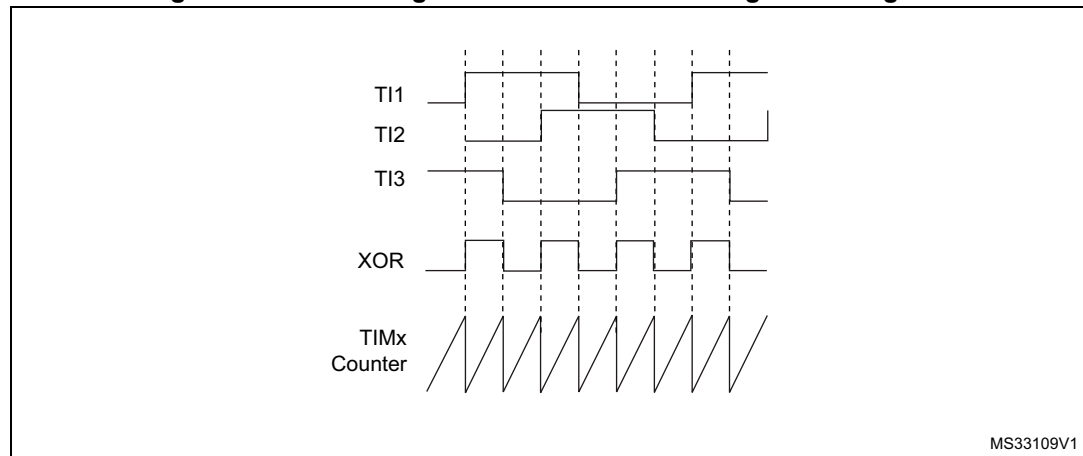
Figure 154. Measuring time interval between edges on 3 signals
