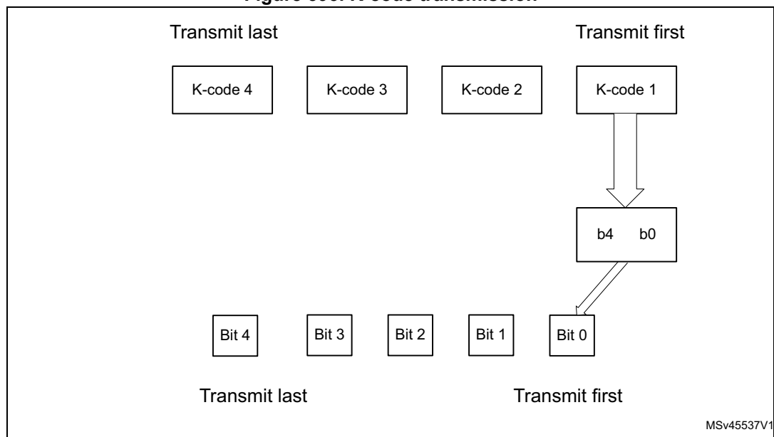
Figure 393. K-code transmission
