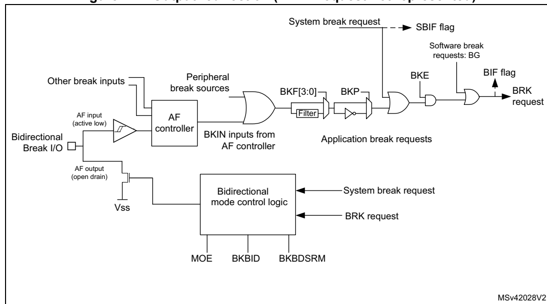
Figure 147. Output redirection (BRK2 request not represented)
