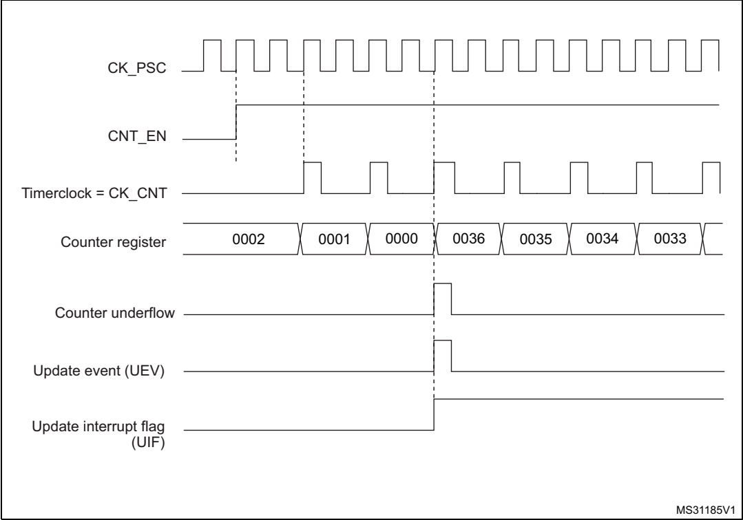
Figure 170. Counter timing diagram, internal clock divided by 2
