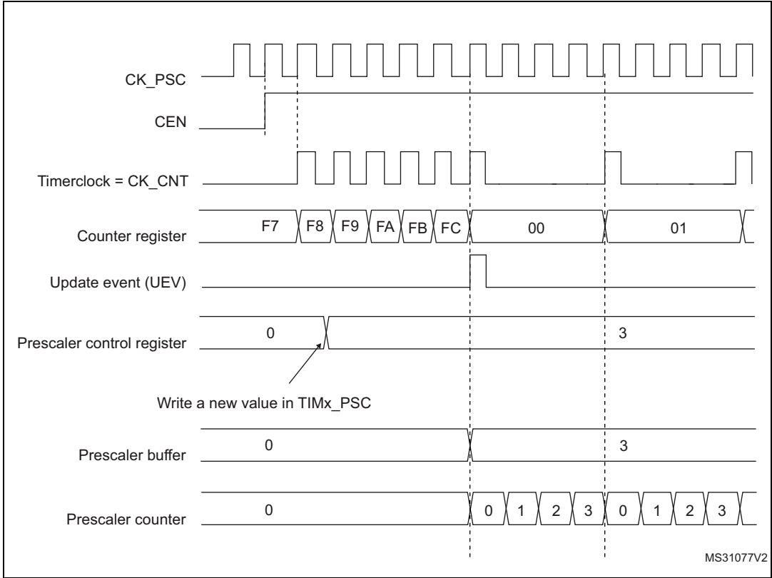
Figure 212. Counter timing diagram with prescaler division change from 1 to 4
