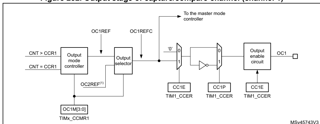
Figure 232. Output stage of capture/compare channel (channel 1)
