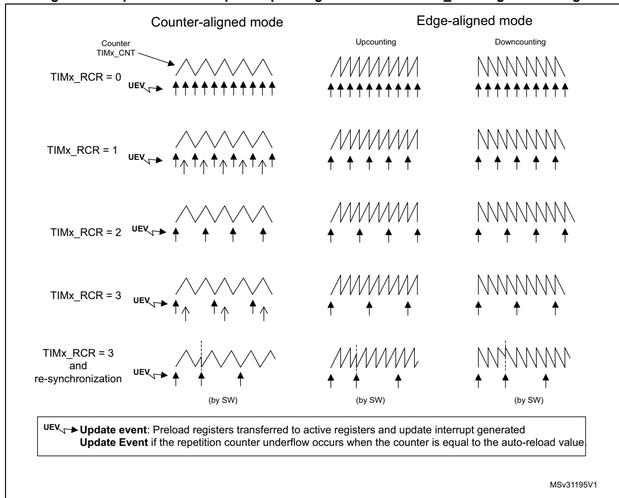
Figure 120. Update rate examples depending on mode and TIMx_RCR register settings
