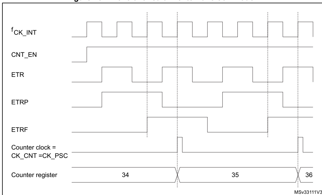
Figure 184. Control circuit in external clock mode 2
