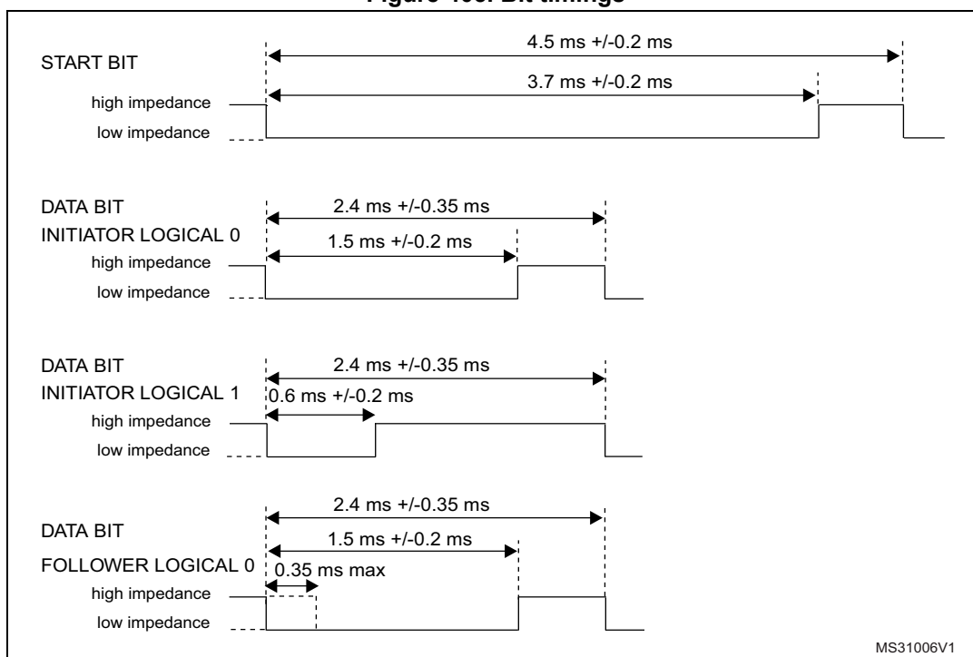
Figure 405. Bit timings
