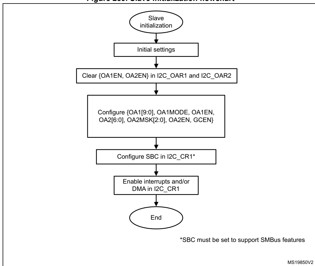
Figure 289. Slave initialization flowchart
