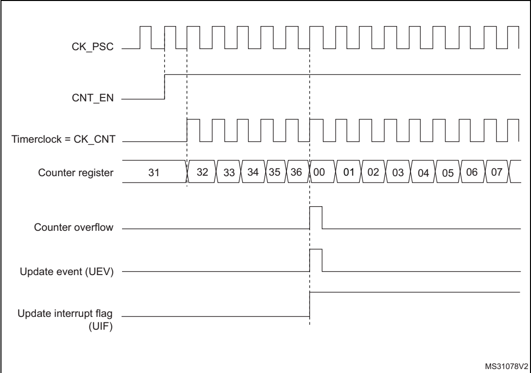
Figure 239. Counter timing diagram, internal clock divided by 1
