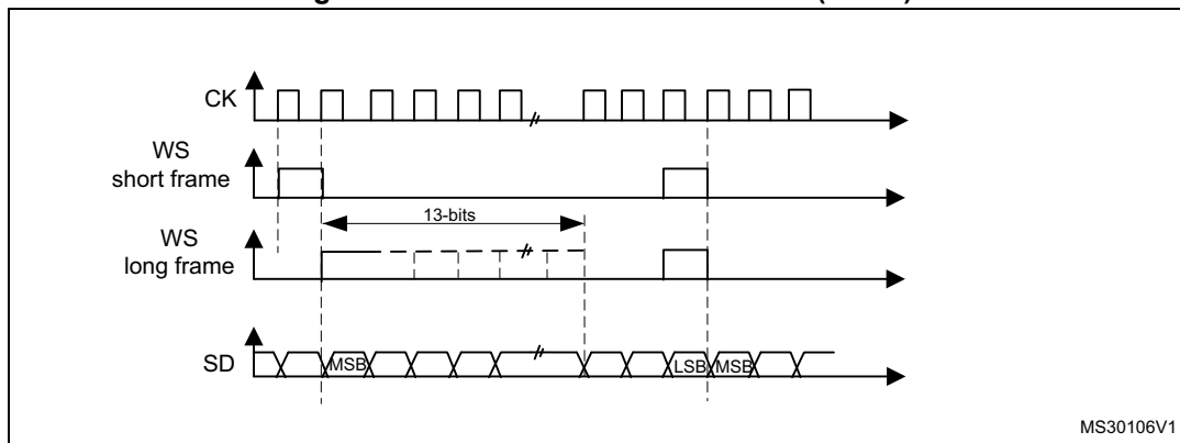
Figure 386. PCM standard waveforms (16-bit)
