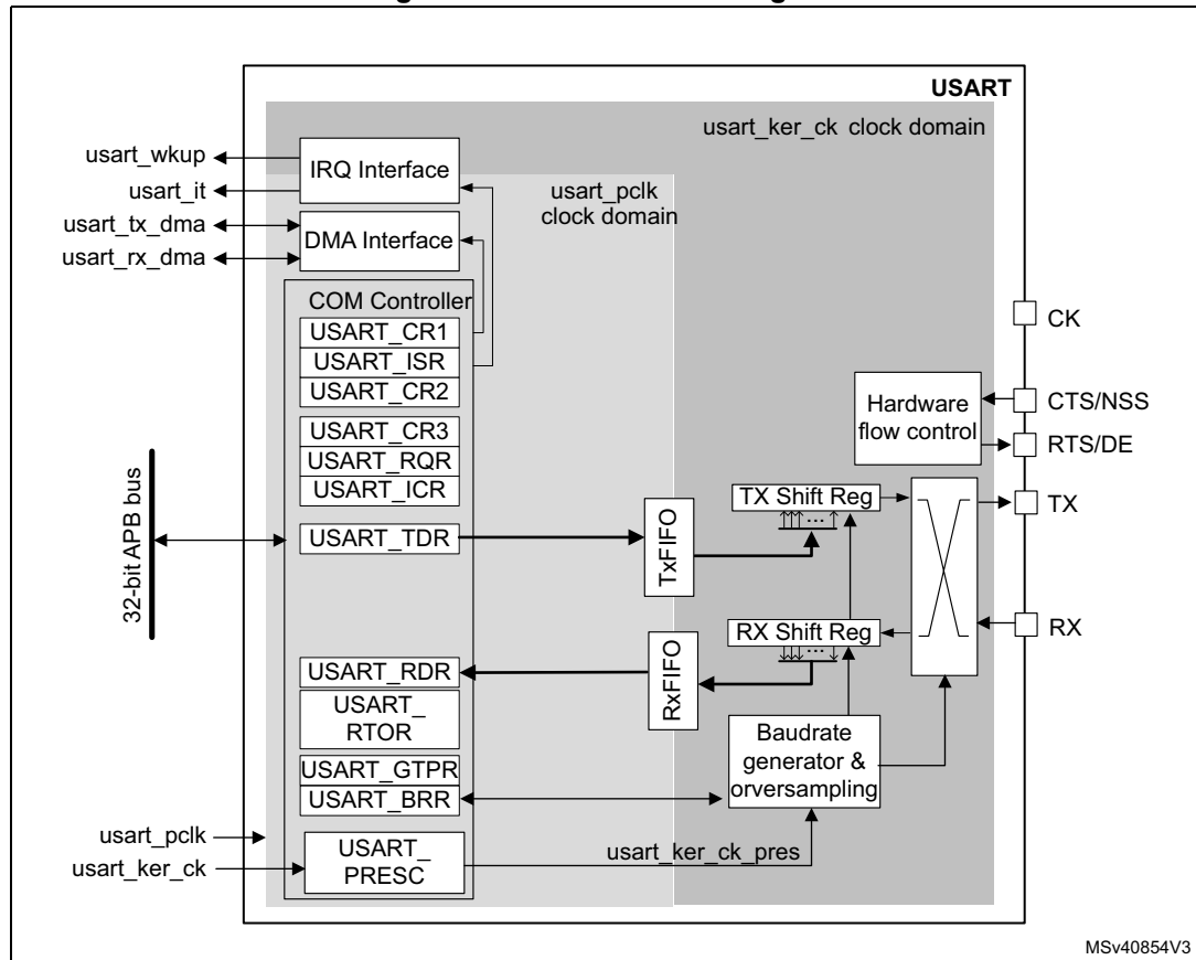
Figure 313. USART block diagram
