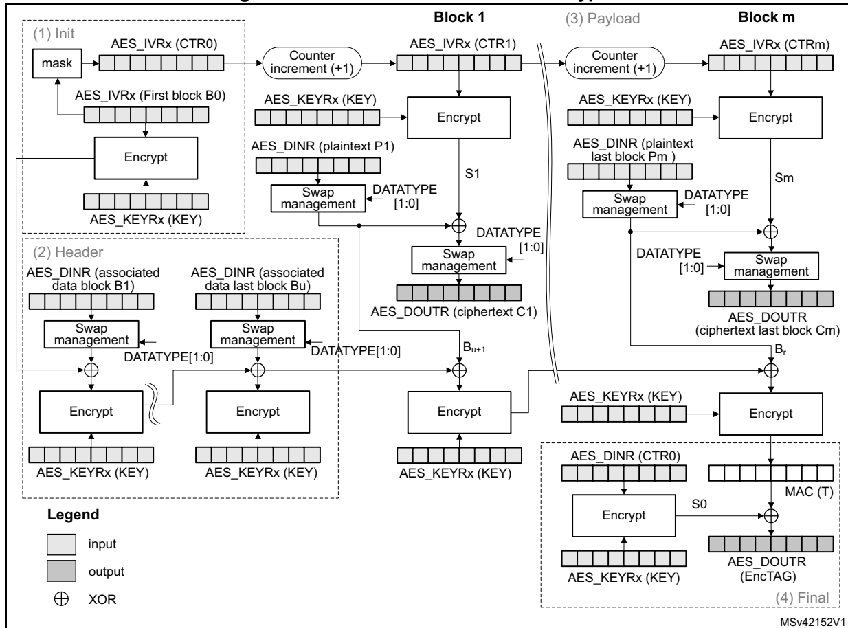
Figure 96. CCM mode authenticated encryption
