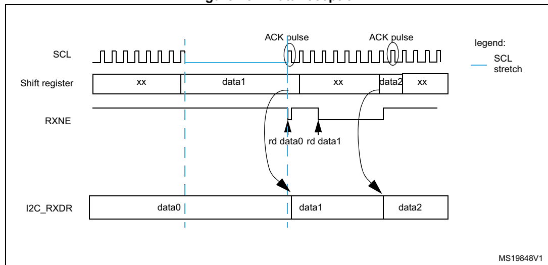
Figure 287. Data reception
