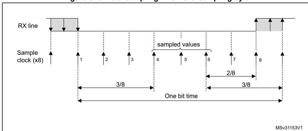
Figure 320. Data sampling when oversampling by 8
