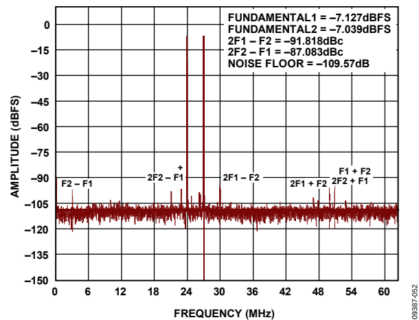
Figure 58. Measured Two-Tone Performance of the Circuit in Figure 55 for a 100 MHz Input Signal
