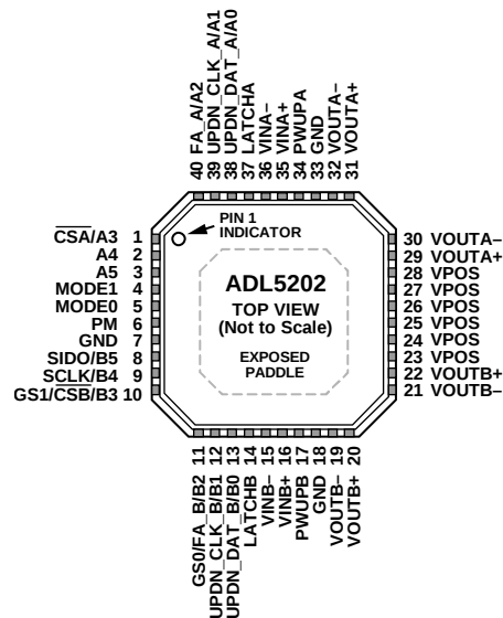
Figure 5. Pin Configuration
