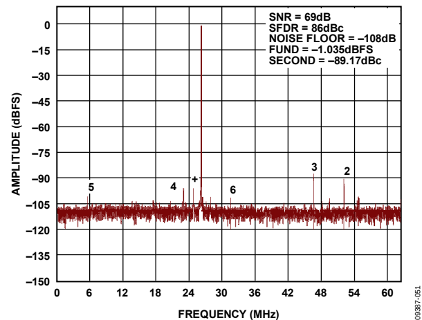
Figure 57. Measured Single-Tone Performance of the Circuit in Figure 55 for a 100 MHz Input Signal
