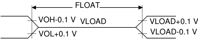
Figure 45. Float Waveforms
