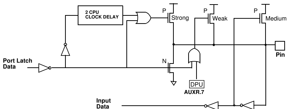
Figure 11. Quasi-Bidirectional Output
