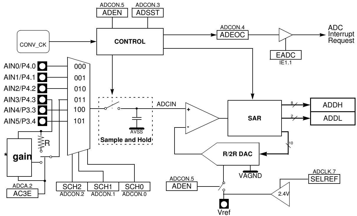
Figure 26. ADC Description
