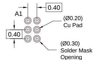
RECOMMENDED LAND PATTERN (NSMD PAD TYPE)
