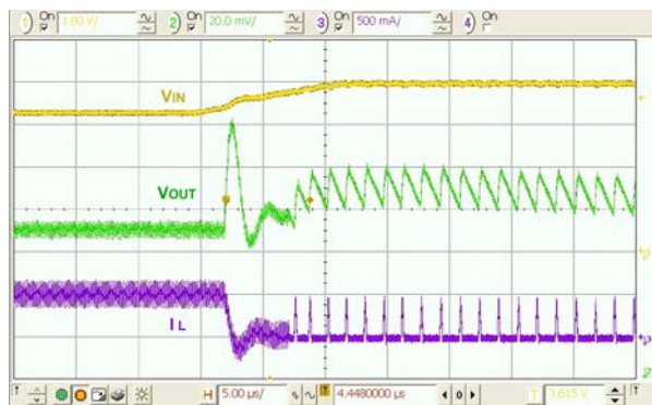
Figure 23. Combined Line / Load Transient, 3.3-3.9 V_{IN} , 10 \mu\text{s} Edge, 400-36 mA Load, 100 ns Edge
