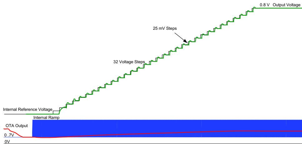
Figure 30. Soft-Start Details
