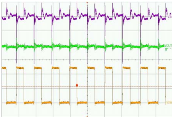
Input = 12 V, Output = 5.0 V, Load = 2 A, CH3 (Purple) = V_{IN} , CH2 (Green) = V_{OUT} , CH1 (Yellow) = V_{SW} CH3: 200 mV/div; CH2: 50 mV/div; CH1: 5.0 V/div Time Scale: 2.0 \mu s/div; Figure 45
