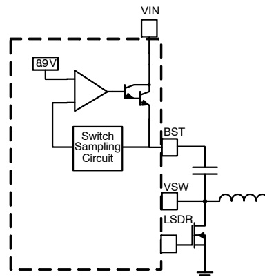
Figure 37. Boost Circuit
