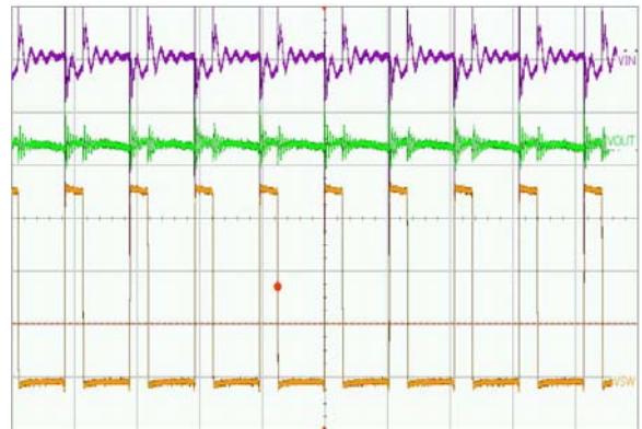
Input = 18 V, Output = 5.0 V, Load = 2 A, CH3 (Purple) = V_{IN} , CH2 (Green) = V_{OUT} , CH1 (Yellow) = V_{SW} CH3: 200 mV/div; CH2: 50 mV/div; CH1: 5.0 V/div Time Scale: 2.0 \mu s/div; Figure 45
