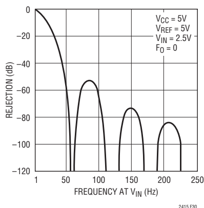
Figure 30. Rejection vs Frequency at V_{IN}
