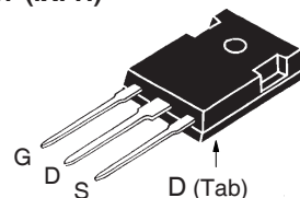
TO-247 (IXFH)
