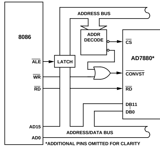
Figure 19. AD7880–8086 Interface
