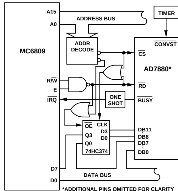
Figure 20. AD7880–6809 Interface
