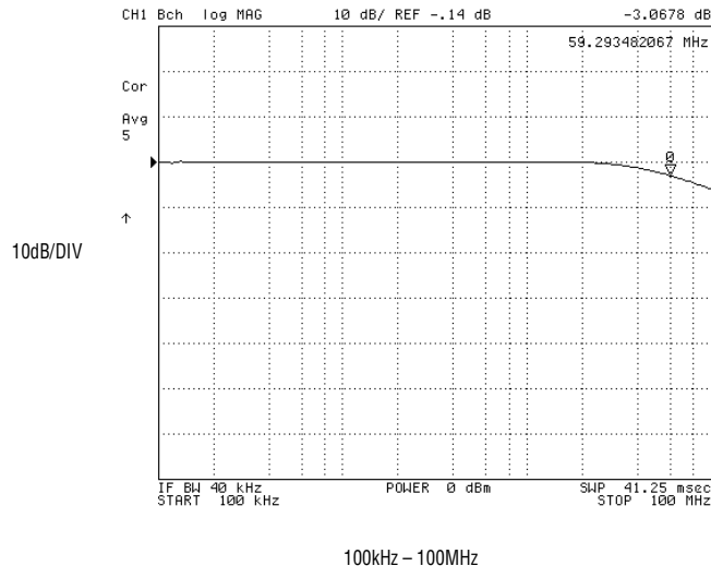
Figure 2. Typical Small-Signal Frequency Response
