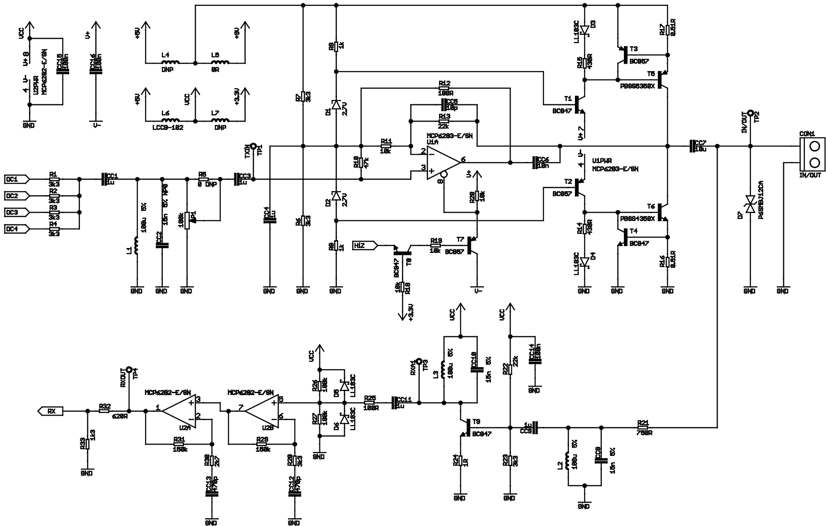
FIGURE A-4: CONSUMER-BAND BPSK 7.2 kbps PLM PICTail™ PLUS DAUGHTER BOARD SCHEMATIC SHEET 1 OF 2
