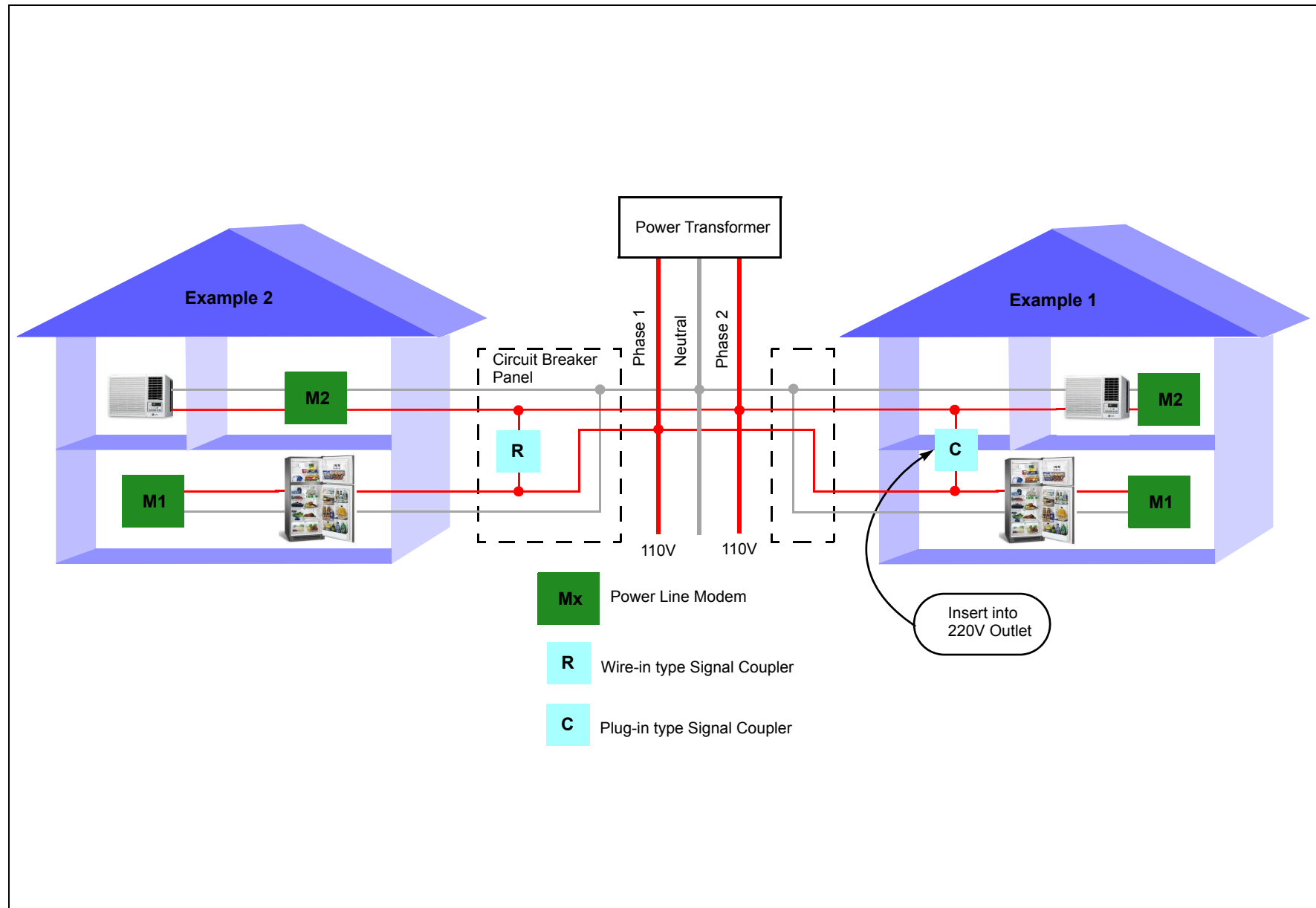
FIGURE 1-4: DUAL-PHASE POWER SUPPLY EXAMPLES
