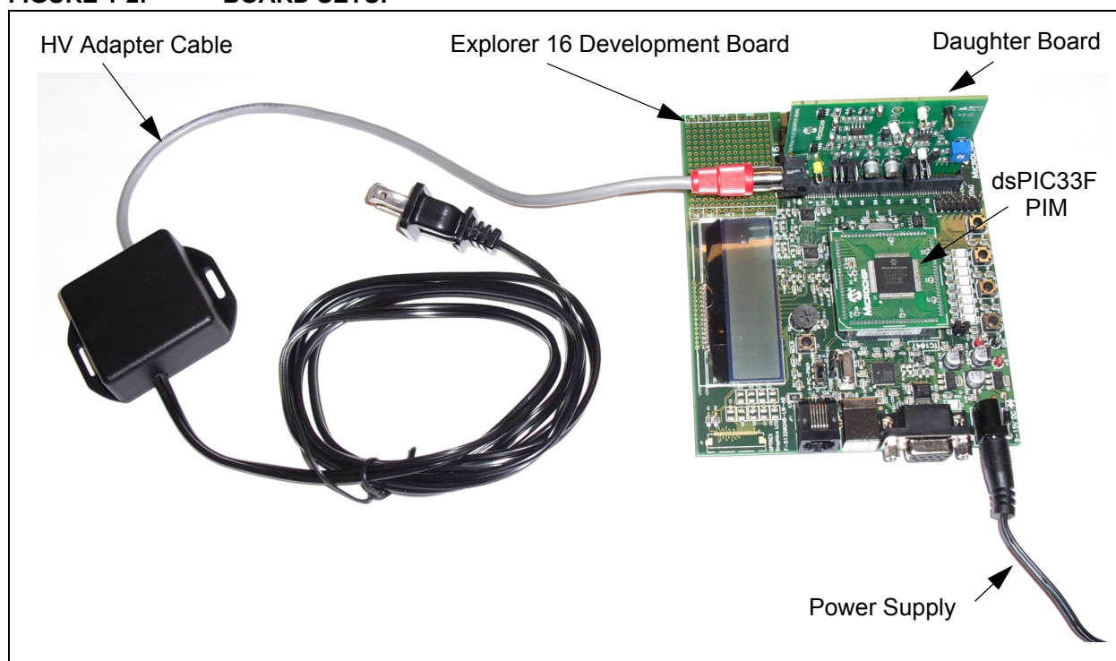
FIGURE 1-2: BOARD SETUP
