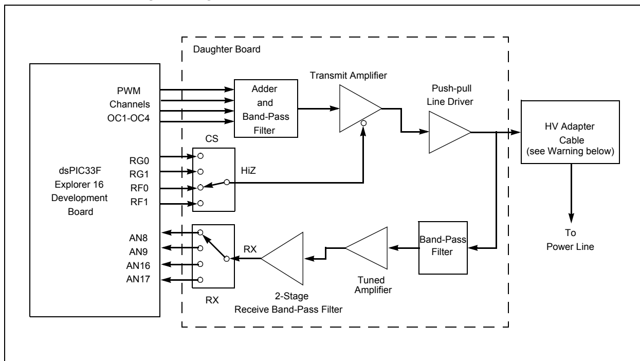
FIGURE 2-1: CONSUMER-BAND BPSK 7.2 kbps PLM PICTail™ PLUS DAUGHTER BOARD BLOCK DIAGRAM
