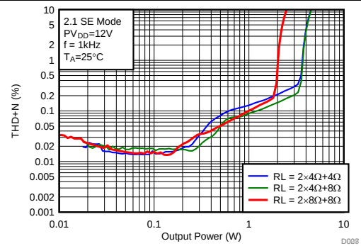
Figure 6. Total Harmonic Distortion + Noise vs Output Power
