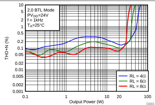
Figure 21. Total Harmonic Distortion + Noise vs Output Power
