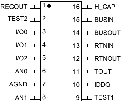
Figure 3. 33784 Pin Connections
