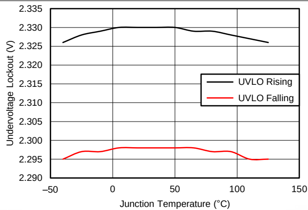
Figure 1. UVLO – Undervoltage Lockout – V
