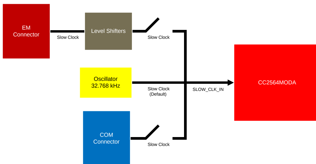
Figure 9. Clock Input
