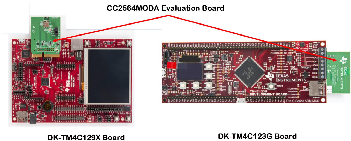
Figure 3. TM4C Hardware Setup Example
