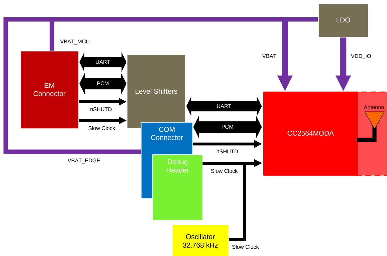
Figure 7. CC2564MODAEM Block Diagram
