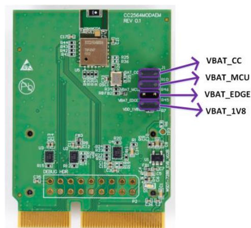
Figure 8. Jumper Configurations
