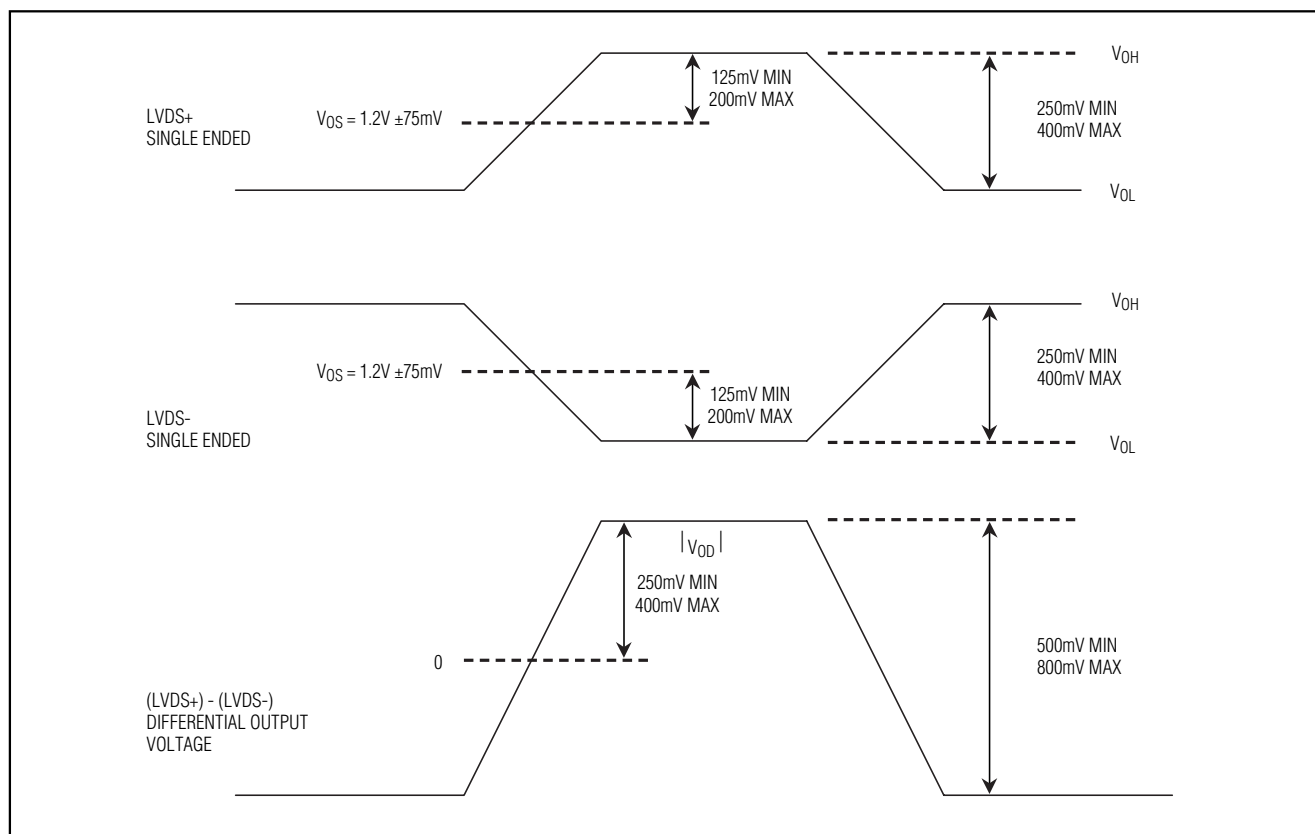
Figure 1. LVDS Output Levels
