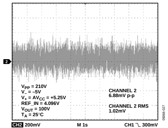
Figure 15. Wideband Noise
