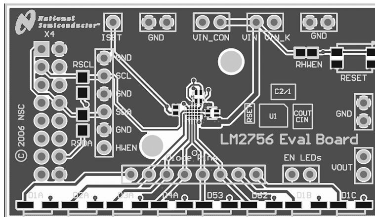
Figure 1. Top Layer
