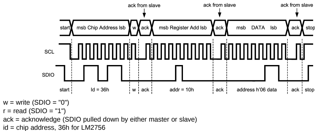
Figure 7. Write Cycle
