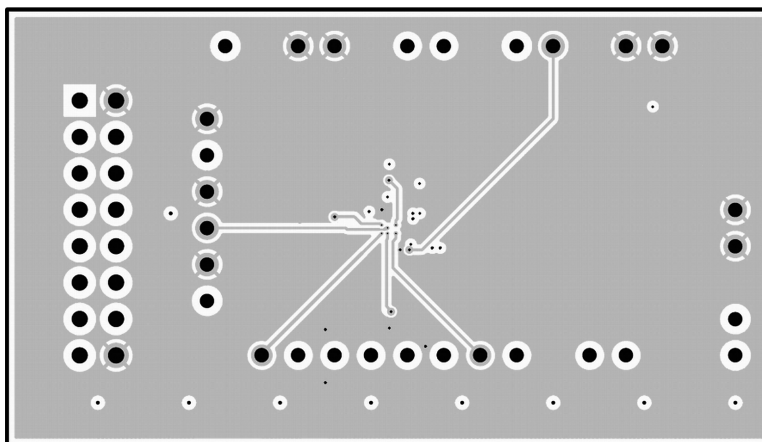
Figure 2. Middle Layer 1
