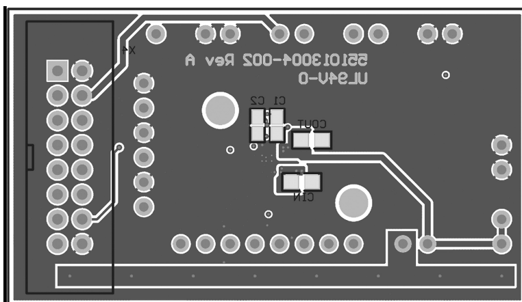
Figure 4. Bottom Layer (unmirrored)
