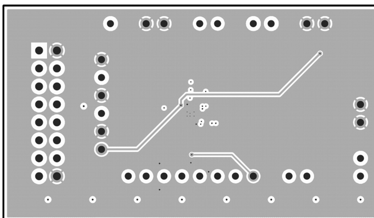
Figure 3. Middle Layer 2
