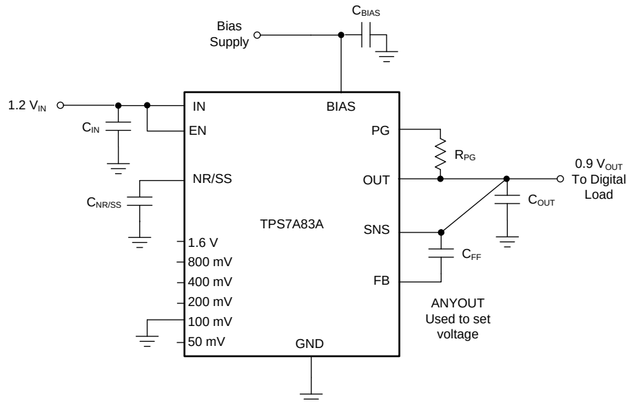
Figure 67. TPS7A83A Typical Application: Low-Input, Low-Output (LILO) Voltage Conditions
