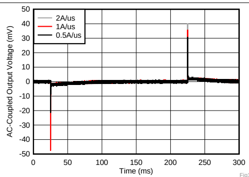
Figure 16. Load Transient vs Time for V_{OUT} = 0.8\text{ V}
