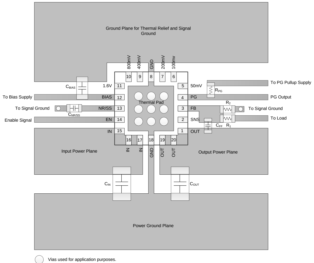
Figure 70. Example Layout
