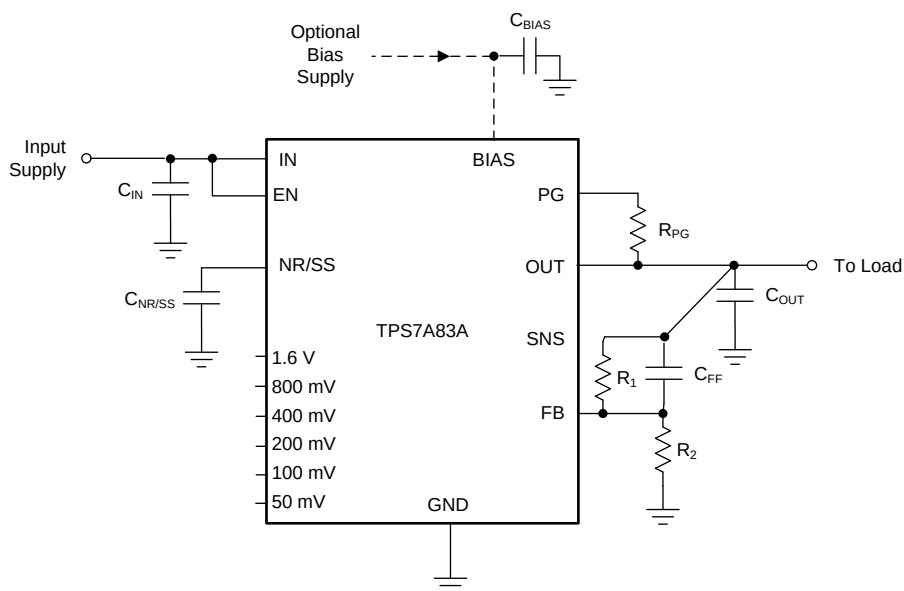
Figure 47. Adjustable Operation
