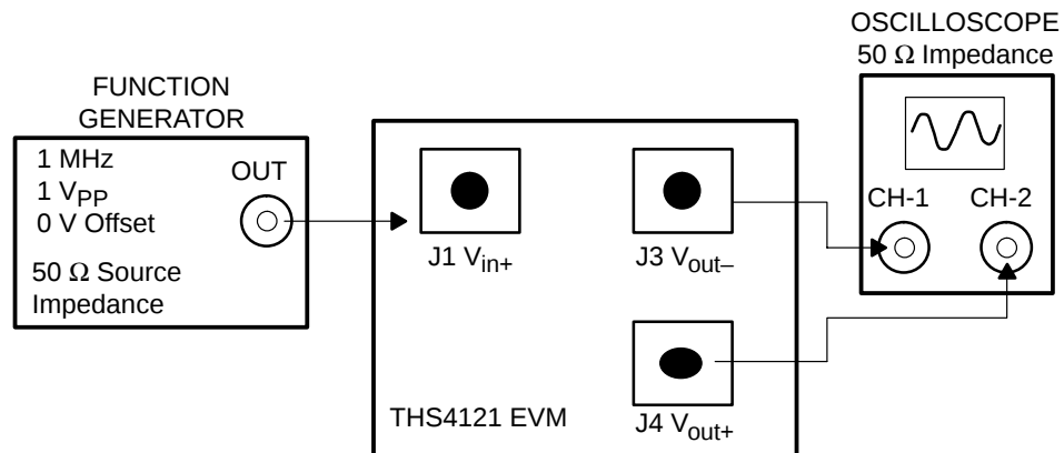
Figure 2–2. Signal Connections
