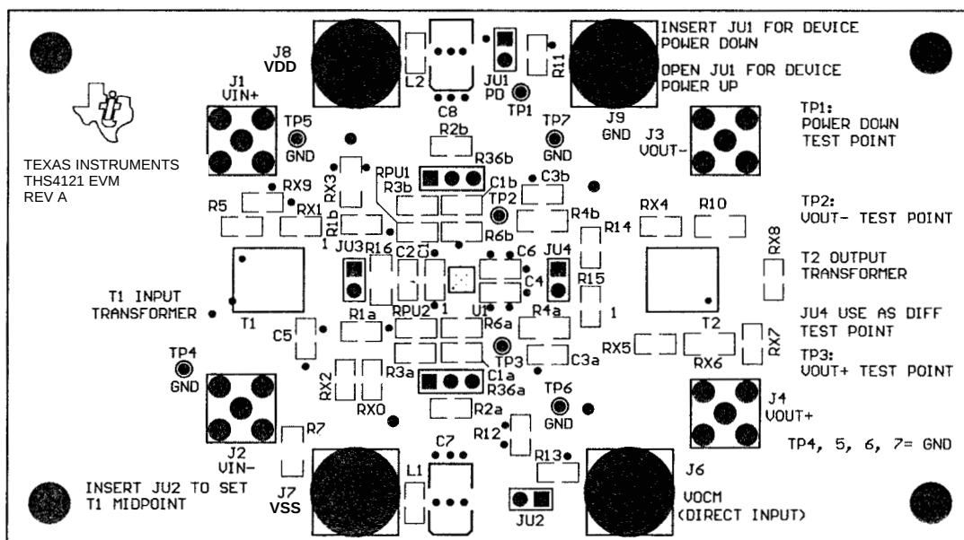
Figure 1–7. Top Layer (Silkscreen)
