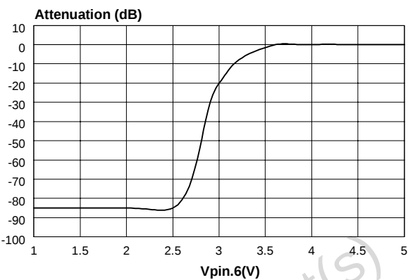
Figure 9. Mute Attenuation vs Vpin 6
