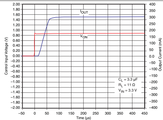
Figure 20. t_{ON} Response
