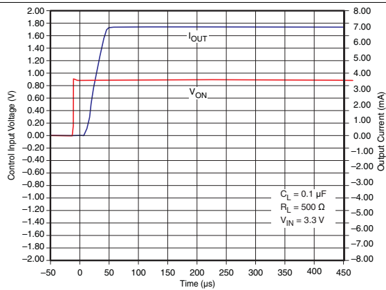
Figure 17. t_{ON} Response
