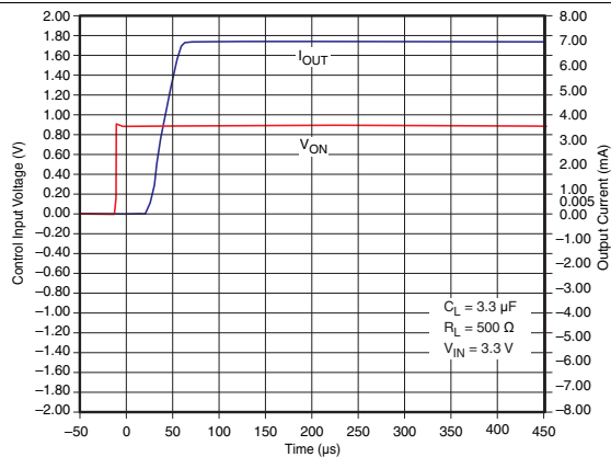
Figure 19. t_{ON} Response
