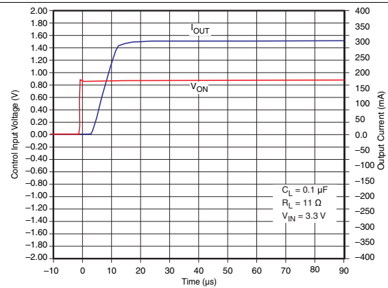
Figure 18. t_{ON} Response
