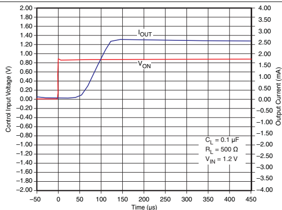
Figure 21. t_{ON} Response
