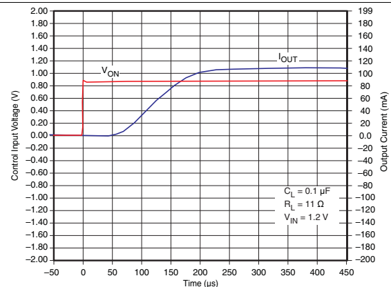
Figure 22. t_{ON} Response
