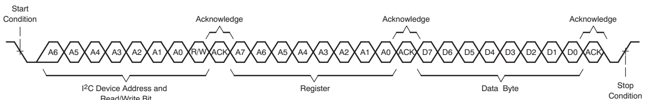
Figure 20. Single-Byte Write Transfer
