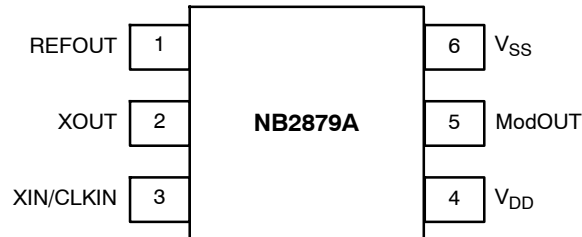
Figure 2. Pin Configuration
