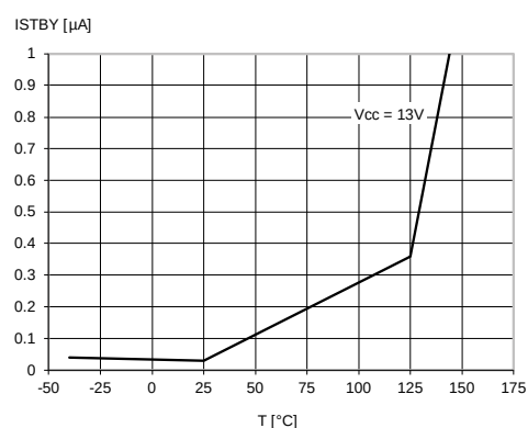
Figure 16: Standby current
