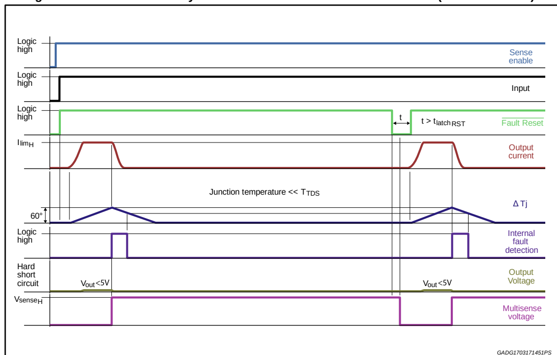
Figure 10: Latch functionality - behavior in hard short circuit condition ( T_{AMB} \ll T_{TDS} )
